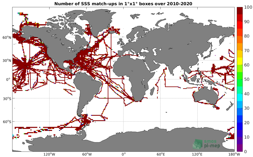
Figure 4: Number of SSS match-ups between TSG (SAMOS) SSS and the SMOS SSS L3 v5 - 18 Days (CATDS-CECOS-LOCEAN) SSS product for the Global Ocean Pi-MEP region over 1°x1° boxes and for the full satellite product period.
