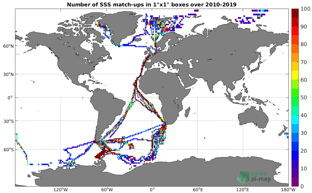
Figure 4: Number of SSS match-ups between TSG (Polarstern) SSS and the SMOS SSS L3 v5 - 18 Days (CATDS-CECOS-LOCEAN) SSS product for the Global Ocean Pi-MEP region over 1^\circ \times 1^\circ boxes and for the full satellite product period.
