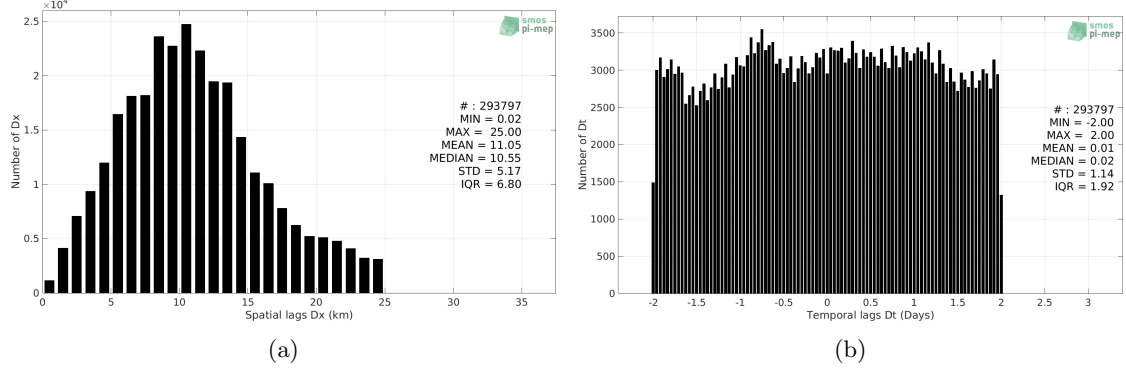
Figure 5: Histograms of the spatial (a) and temporal (b) lags between the time of the TSG (Polarstern) measurements and the date of the corresponding SMOS SSS L3 v5 - 18 Days (CATDS-CECOS-LOCEAN) SSS product.
