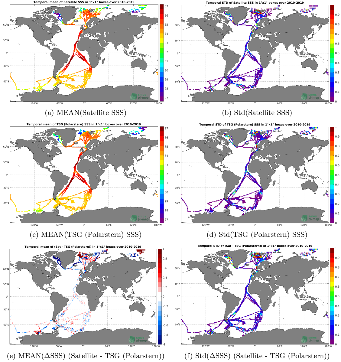
Figure 6: Temporal mean (left) and Std (right) of SSS from SMOS SSS L3 v5 - 18 Days (CATDS-CECOS-LOCEAN) (top), TSG (Polarstern) (middle), and of \Delta SSS (Satellite - TSG (Polarstern)). Only match-up pairs are used to generate these maps.
