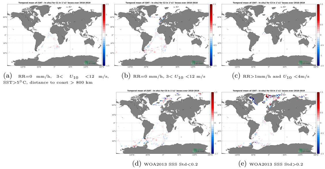
Figure 12: Temporal mean gridded over spatial boxes of size 1^\circ \times 1^\circ of \Delta SSS (SMOS SSS L3 v5 - 18 Days (CATDS-CECOS-LOCEAN) - TSG (Polarstern)) for 5 different subdatasets corresponding to: RR=0 mm/h, 3 < U_{10} < 12 m/s, SST > 5^\circ C , distance to coast > 800 km (a), RR=0 mm/h, 3 < U_{10} < 12 m/s (b), RR > 1 mm/h and U_{10} < 4 m/s (c), WOA2013 SSS Std < 0.2 (d), WOA2013 SSS Std > 0.2 (e).
