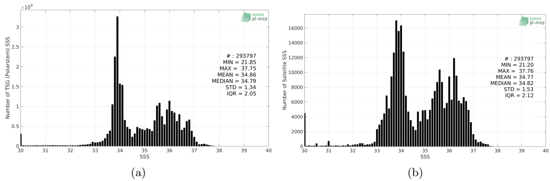
Figure 2: Histograms of SSS from TSG (Polarstern) (a) and SMOS SSS L3 v5 - 18 Days (CATDS-CECOS-LOCEAN) (b) considering all match-up pairs per bins of 0.1 over the Global Ocean Pi-MEP region and for the full satellite product period.
