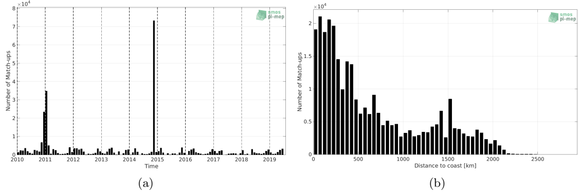
Figure 1: Number of match-ups between TSG (Polarstern) and SMOS SSS L3 v5 - 18 Days (CATDS-CECOS-LOCEAN) SSS as a function of time (a) and as function of the distance to coast (b) over the Global Ocean Pi-MEP region and for the full satellite product period.
