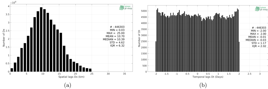
Figure 5: Histograms of the spatial (a) and temporal (b) lags between the location/time of the TSG (NCEI-0170743) measurement and the date of the corresponding SMOS SSS L3 v5 - 18 Days (CATDS-CECOS-LOCEAN) SSS pixel.
