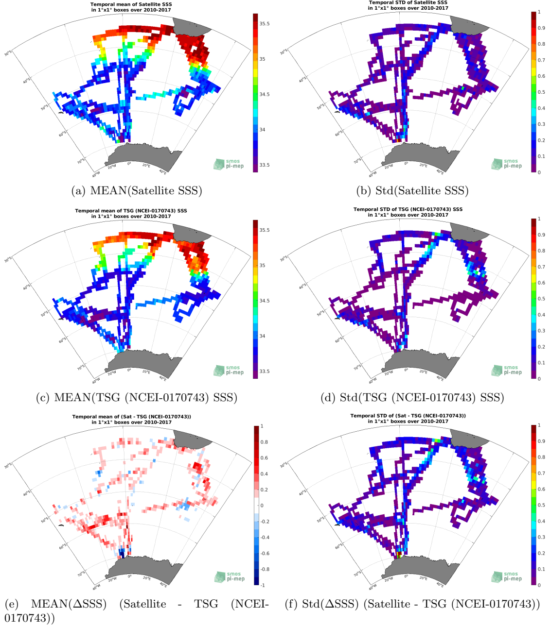
Figure 6: Temporal mean (left) and Std (right) of SSS from SMOS SSS L3 v5 - 18 Days (CATDS-CECOS-LOCEAN) (top), TSG (NCEI-0170743) (middle), and of \Delta SSS (Satellite - TSG (NCEI-0170743)). Only match-up pairs are used to generate these maps.
