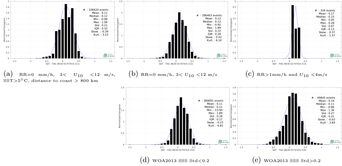
Figure 13: Normalized histogram of \Delta SSS (SMOS SSS L3 v5 - 18 Days (CATDS-CECOS-LOCEAN) - TSG (NCEI-0170743)) for 5 different subdatasets corresponding to: RR=0 mm/h, 3 < U_{10} < 12 m/s, SST>5°C, distance to coast > 800 km (a), RR=0 mm/h, 3 < U_{10} < 12 m/s (b), RR>1mm/h and U_{10} < 4 m/s (c), WOA2013 SSS Std<0.2 (d), WOA2013 SSS Std>0.2 (e).
