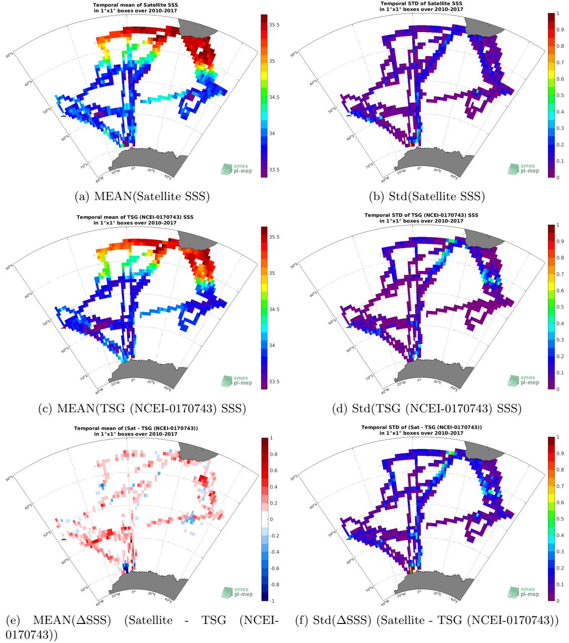
Figure 6: Temporal mean (left) and Std (right) of SSS from SMOS SSS L3 v5 - 18 Days (CATDS-CECOS-LOCEAN) (top), TSG (NCEI-0170743) (middle), and of \Delta SSS (Satellite - TSG (NCEI-0170743)). Only match-up pairs are used to generate these maps.
