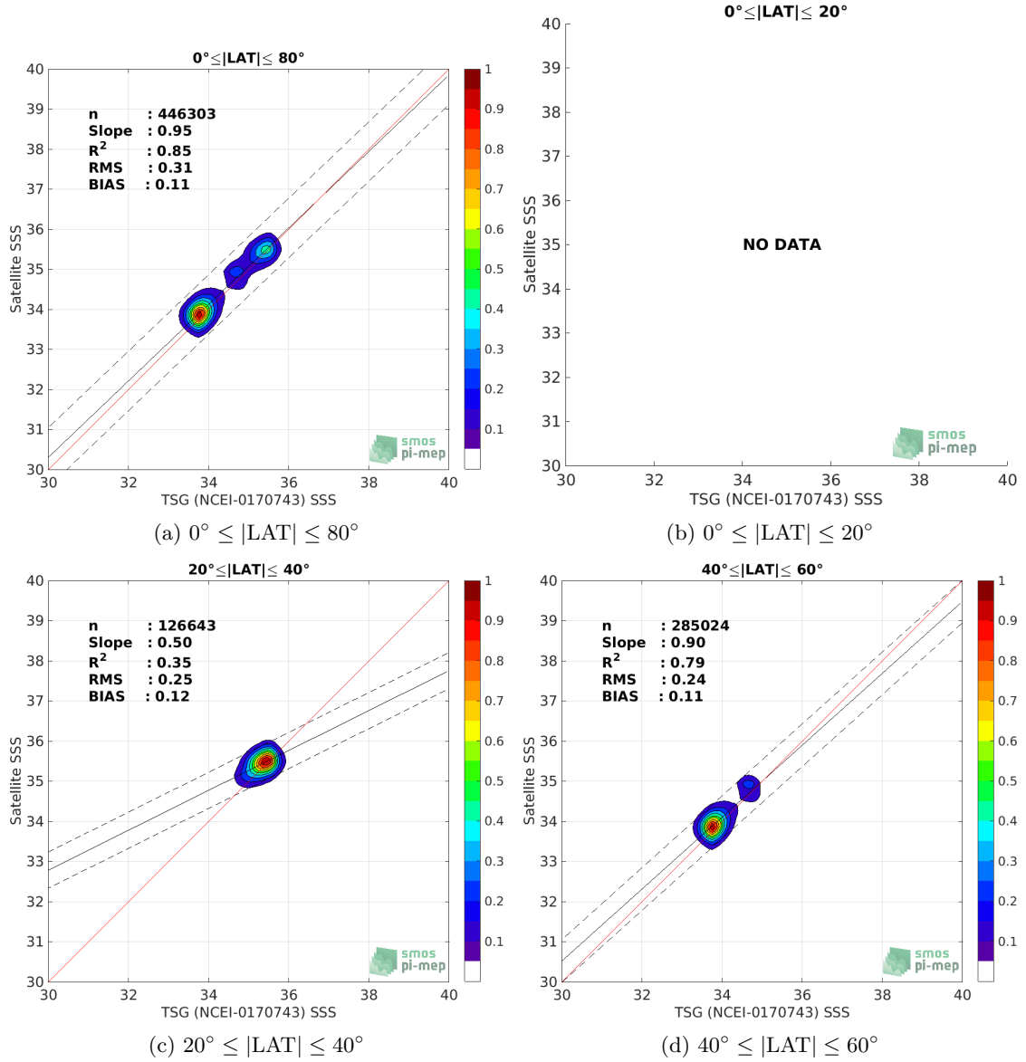
Figure 9: Contour maps of the concentration of SMOS SSS L3 v5 - 18 Days (CATDS-CECOS-LOCEAN) SSS (y-axis) versus TSG (NCEI-0170743) SSS (x-axis) at match-up pairs for different latitude bands. For each plot, the red line shows x=y . The black thin and dashed lines indicate a linear fit through the data cloud and the \pm 95\% confidence levels, respectively. The number match-up pairs n , the slope and R^2 coefficient of the linear fit, the root mean square (RMS) and the mean bias between satellite and in situ data are indicated for each latitude band in each plots.
