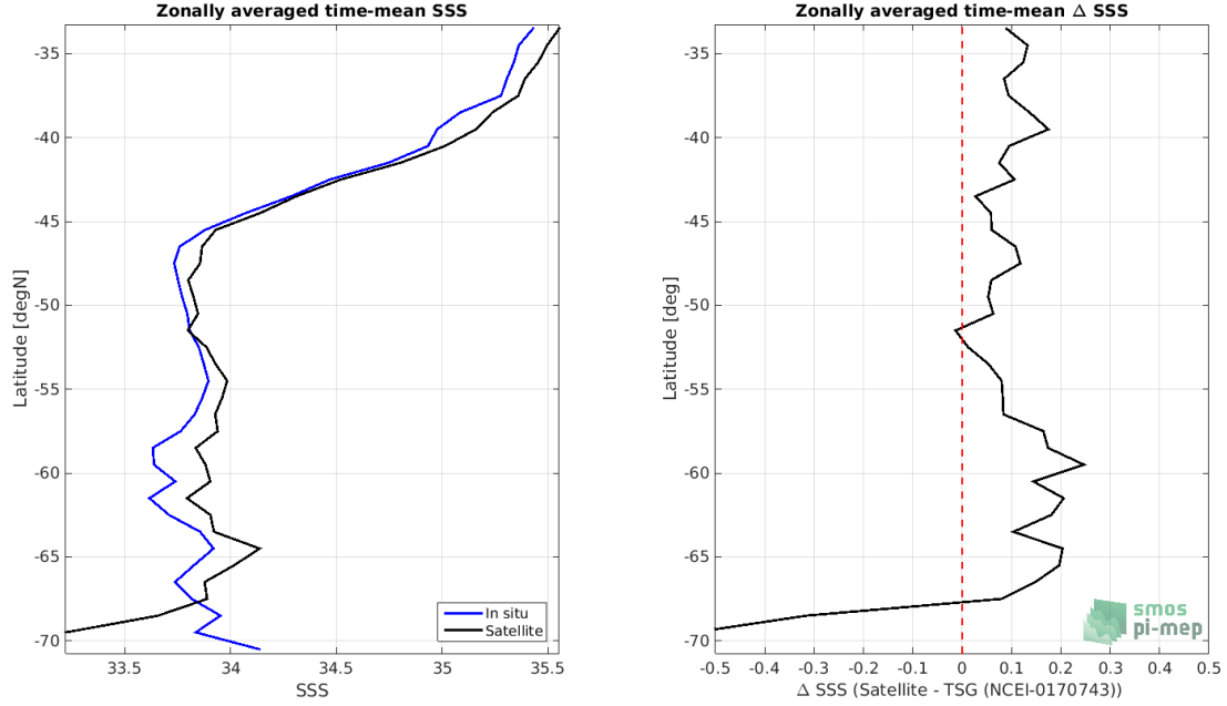
Figure 8: Left panel: Zonal mean SSS from SMOS SSS L3 v5 - 18 Days (CATDS-CECOS-LOCEAN) satellite product (black) and from TSG (NCEI-0170743) (blue). Right panel: Zonal mean of \Delta SSS (Satellite - TSG (NCEI-0170743)) for all the collected Pi-MEP match-up pairs estimated over the full satellite product period.
