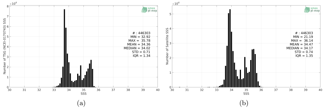
Figure 2: Histograms of SSS from TSG (NCEI-0170743) (a) and SMOS SSS L3 v5 - 18 Days (CATDS-CECOS-LOCEAN) (b) considering all match-up pairs per bins of 0.1 over the Global Ocean Pi-MEP region and for the full satellite product period.
