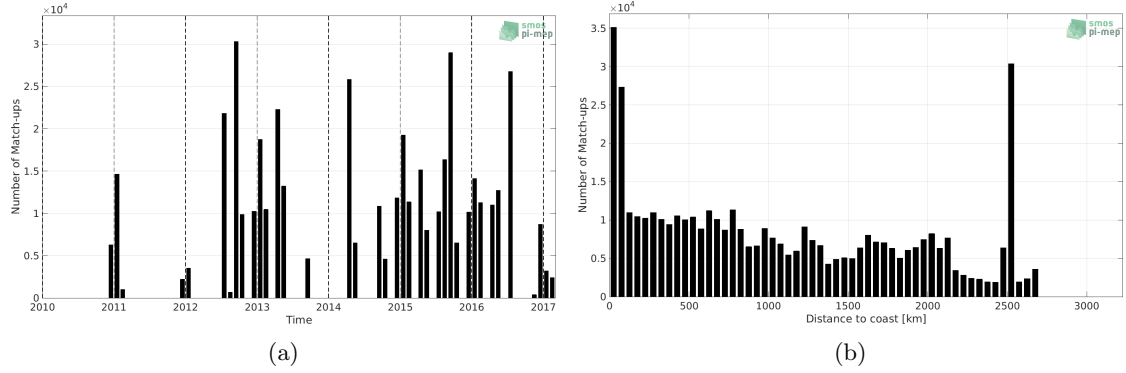
Figure 1: Number of match-ups between TSG (NCEI-0170743) and SMOS SSS L3 v5 - 18 Days (CATDS-CECOS-LOCEAN) SSS as a function of time (a) and as function of the distance to coast (b) over the Global Ocean Pi-MEP region and for the full satellite product period.
