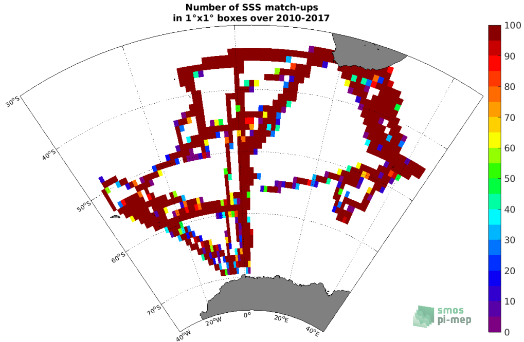
Figure 4: Number of SSS match-ups between TSG (NCEI-0170743) SSS and the SMOS SSS L3 v5 - 18 Days (CATDS-CECOS-LOCEAN) SSS product for the Global Ocean Pi-MEP region over 1°x1° boxes and for the full satellite product period.
