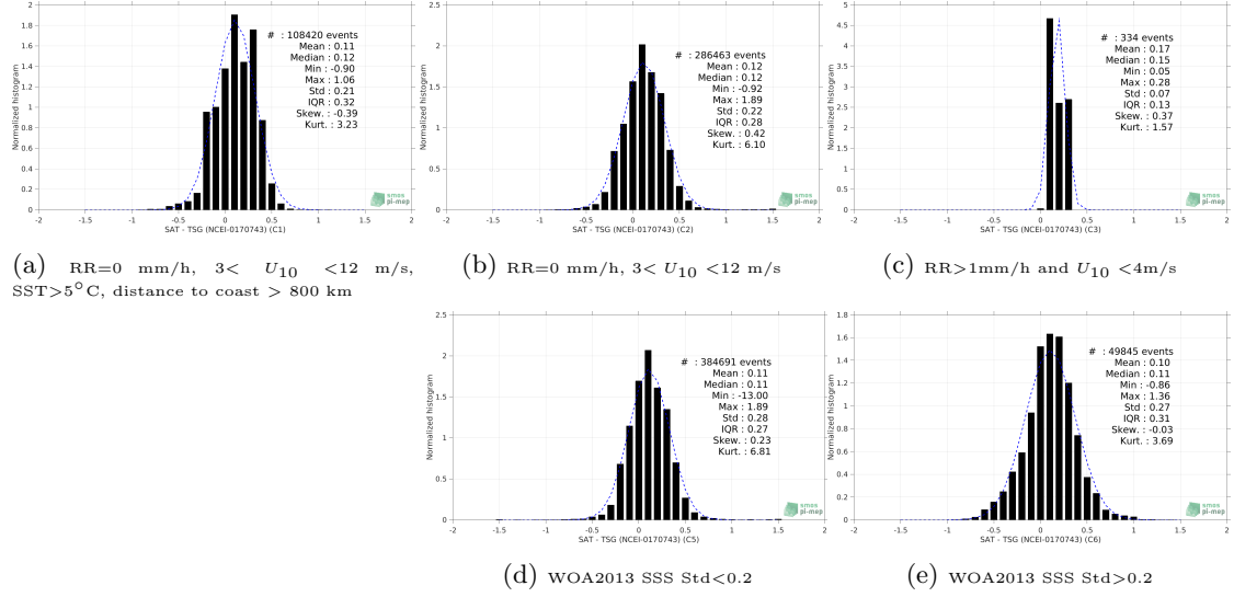
Figure 13: Normalized histogram of \Delta SSS (SMOS SSS L3 v5 - 18 Days (CATDS-CECOS-LOCEAN) - TSG (NCEI-0170743)) for 5 different subdatasets corresponding to: RR=0 mm/h, 3 < U_{10} < 12 m/s, SST>5°C, distance to coast > 800 km (a), RR=0 mm/h, 3 < U_{10} < 12 m/s (b), RR>1mm/h and U_{10} < 4 m/s (c), WOA2013 SSS Std<0.2 (d), WOA2013 SSS Std>0.2 (e).
