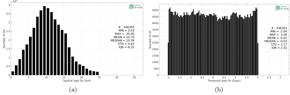
Figure 5: Histograms of the spatial (a) and temporal (b) lags between the time of the TSG (NCEI-0170743) measurements and the date of the corresponding SMOS SSS L3 v5 - 18 Days (CATDS-CECOS-LOCEAN) SSS product.
