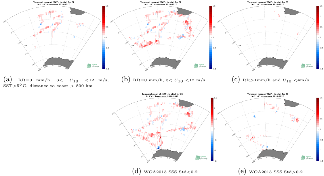
Figure 12: Temporal mean gridded over spatial boxes of size 1^{\circ}\times 1^{\circ} of \Delta\text{SSS} (SMOS SSS L3 v5 - 18 Days (CATDS-CECOS-LOCEAN) - TSG (NCEI-0170743)) for 5 different subdatasets corresponding to: RR=0 mm/h, 3 < U_{10} < 12 m/s, SST >5^{\circ}\text{C} , distance to coast > 800 km (a), RR=0 mm/h, 3 < U_{10} < 12 m/s (b), RR >1 mm/h and U_{10} < 4 m/s (c), WOA2013 SSS Std <0.2 (d), WOA2013 SSS Std >0.2 (e).
