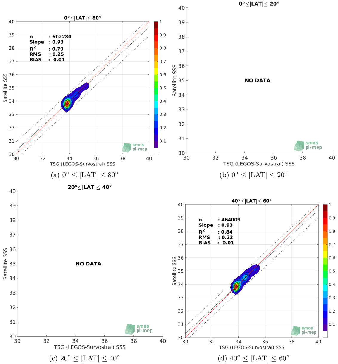
Figure 9: Contour maps of the concentration of SMOS SSS L3 v5 - 18 Days (CATDS-CECOS-LOCEAN) SSS (y-axis) versus TSG (LEGOS-Survostral) SSS (x-axis) at match-up pairs for different latitude bands. For each plot, the red line shows x=y . The black thin and dashed lines indicate a linear fit through the data cloud and the \pm 95\% confidence levels, respectively. The number match-up pairs n , the slope and R^2 coefficient of the linear fit, the root mean square (RMS) and the mean bias between satellite and in situ data are indicated for each latitude band in each plots.
