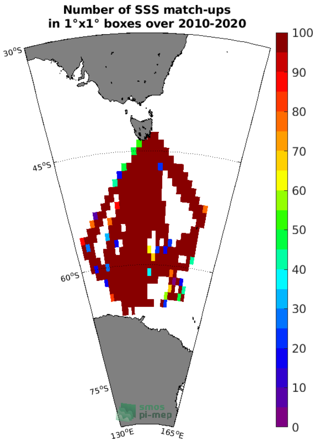
Figure 4: Number of SSS match-ups between TSG (LEGOS-Survostral) SSS and the SMOS SSS L3 v5 - 18 Days (CATDS-CECOS-LOCEAN) SSS product for the Global Ocean Pi-MEP region over 1°x1° boxes and for the full satellite product period.
