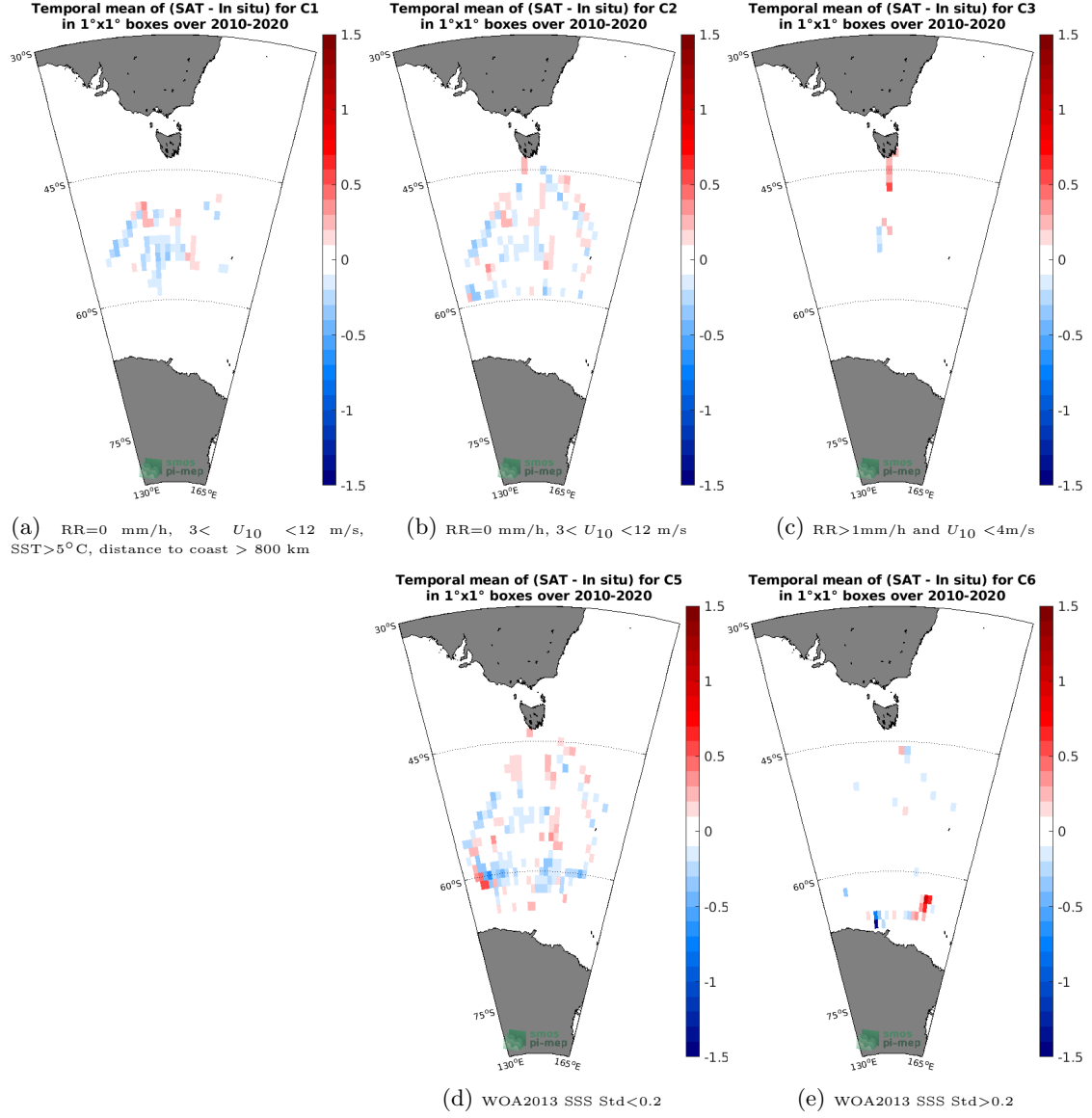
Figure 12: Temporal mean gridded over spatial boxes of size 1^\circ \times 1^\circ of \Delta\text{SSS} (SMOS SSS L3 v5 - 18 Days (CATDS-CECOS-LOCEAN) - TSG (LEGOS-Survostral)) for 5 different subdatasets corresponding to: RR=0 mm/h, 3 < U_{10} < 12 m/s, SST > 5^\circ\text{C} , distance to coast > 800 km (a), RR=0 mm/h, 3 < U_{10} < 12 m/s (b), RR > 1 mm/h and U_{10} < 4 m/s (c), WOA2013 SSS Std < 0.2 (d), WOA2013 SSS Std > 0.2 (e).
