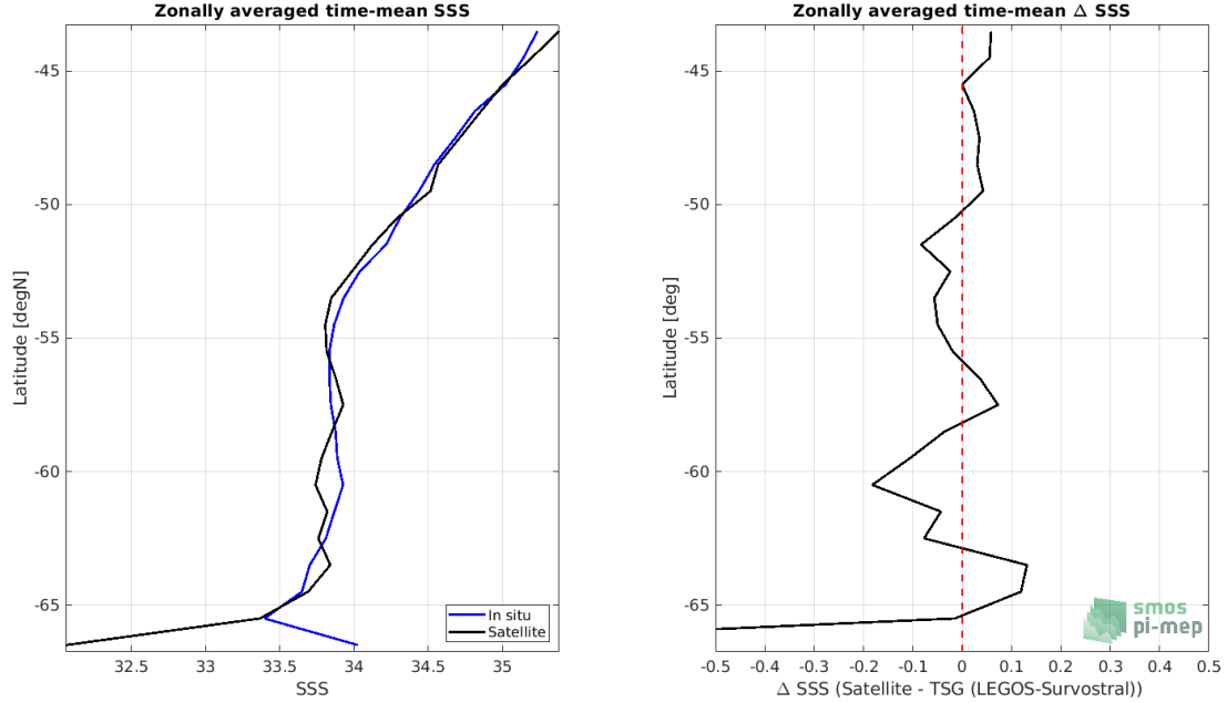
Figure 8: Left panel: Zonal mean SSS from SMOS SSS L3 v5 - 18 Days (CATDS-CECOS-LOCEAN) satellite product (black) and from TSG (LEGOS-Survostral) (blue). Right panel: Zonal mean of \Delta SSS (Satellite - TSG (LEGOS-Survostral)) for all the collected Pi-MEP match-up pairs estimated over the full satellite product period.
