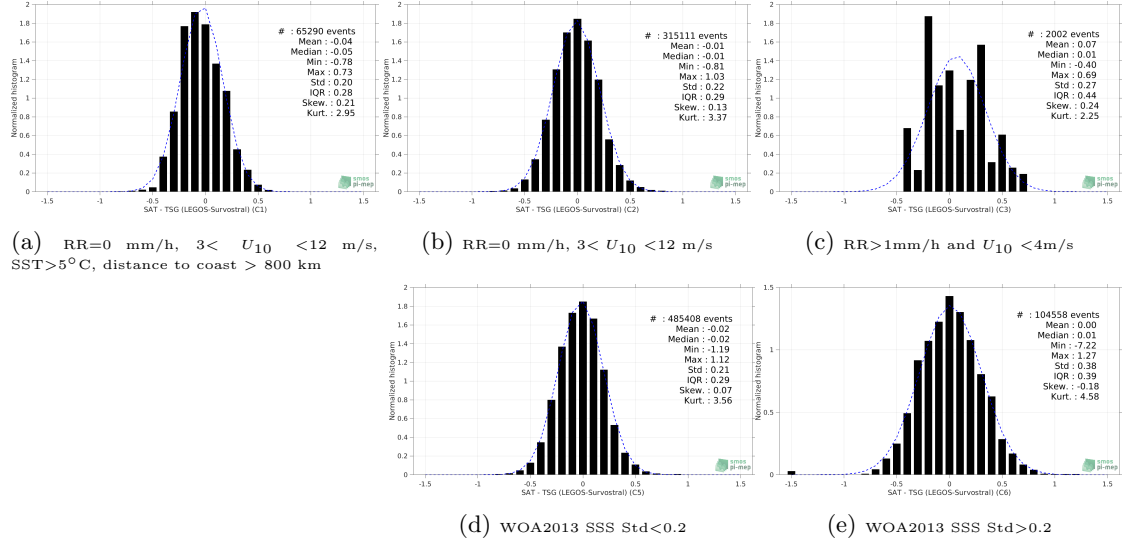
Figure 13: Normalized histogram of \Delta SSS (SMOS SSS L3 v5 - 18 Days (CATDS-CECOS-LOCEAN) - TSG (LEGOS-Survostral)) for 5 different subdatasets corresponding to: RR=0 mm/h, 3 < U_{10} < 12 m/s, SST>5°C, distance to coast > 800 km (a), RR=0 mm/h, 3 < U_{10} < 12 m/s (b), RR>1mm/h and U_{10} < 4 m/s (c), WOA2013 SSS Std<0.2 (d), WOA2013 SSS Std>0.2 (e).
