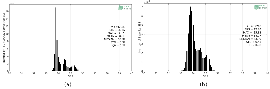
Figure 2: Histograms of SSS from TSG (LEGOS-Survostral) (a) and SMOS SSS L3 v5 - 18 Days (CATDS-CECOS-LOCEAN) (b) considering all match-up pairs per bins of 0.1 over the Global Ocean Pi-MEP region and for the full satellite product period.
