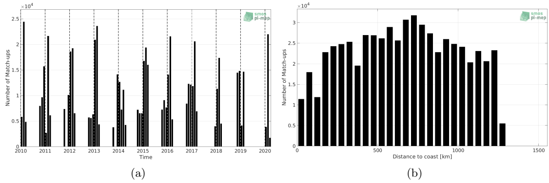
Figure 1: Number of match-ups between TSG (LEGOS-Survostral) and SMOS SSS L3 v5 - 18 Days (CATDS-CECOS-LOCEAN) SSS as a function of time (a) and as function of the distance to coast (b) over the Global Ocean Pi-MEP region and for the full satellite product period.
