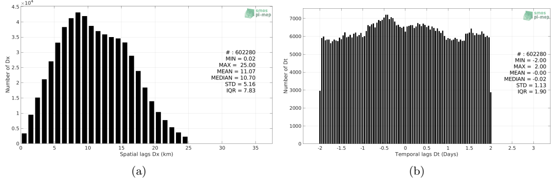
Figure 5: Histograms of the spatial (a) and temporal (b) lags between the location/time of the TSG (LEGOS-Survostral) measurement and the date of the corresponding SMOS SSS L3 v5 - 18 Days (CATDS-CECOS-LOCEAN) SSS pixel.
