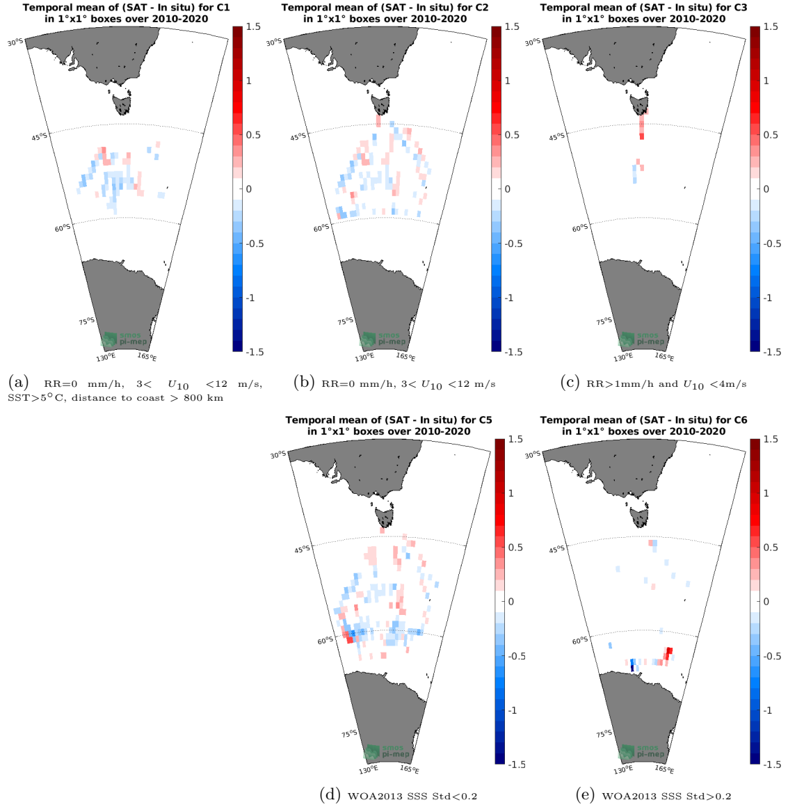
Figure 12: Temporal mean gridded over spatial boxes of size 1°x1° of \Delta\text{SSS} (SMOS SSS L3 v5 - 18 Days (CATDS-CECOS-LOCEAN) - TSG (LEGOS-Survostral)) for 5 different subdatasets corresponding to: RR=0 mm/h, 3 < U_{10} < 12 m/s, SST > 5^\circ\text{C} , distance to coast > 800 km (a), RR=0 mm/h, 3 < U_{10} < 12 m/s (b), RR > 1 mm/h and U_{10} < 4 m/s (c), WOA2013 SSS Std < 0.2 (d), WOA2013 SSS Std > 0.2 (e).
