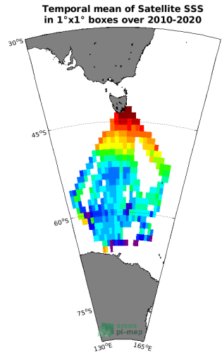
(a) MEAN(Satellite SSS)
