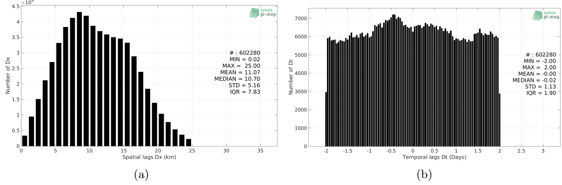
Figure 5: Histograms of the spatial (a) and temporal (b) lags between the time of the TSG (LEGOS-Survostral) measurements and the date of the corresponding SMOS SSS L3 v5 - 18 Days (CATDS-CECOS-LOCEAN) SSS product.
