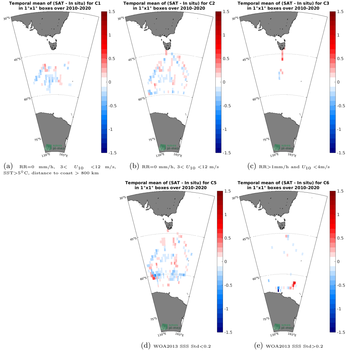
Figure 12: Temporal mean gridded over spatial boxes of size 1°x1° of \Delta SSS (SMOS SSS L3 v5 - 18 Days (CATDS-CECOS-LOCEAN) - TSG (LEGOS-Survostral)) for 5 different subdatasets corresponding to: RR=0 mm/h, 3 < U_{10} < 12 m/s, SST>5°C, distance to coast > 800 km (a), RR=0 mm/h, 3 < U_{10} < 12 m/s (b), RR > 1 mm/h and U_{10} < 4 m/s (c), WOA2013 SSS Std<0.2 (d), WOA2013 SSS Std>0.2 (e).
