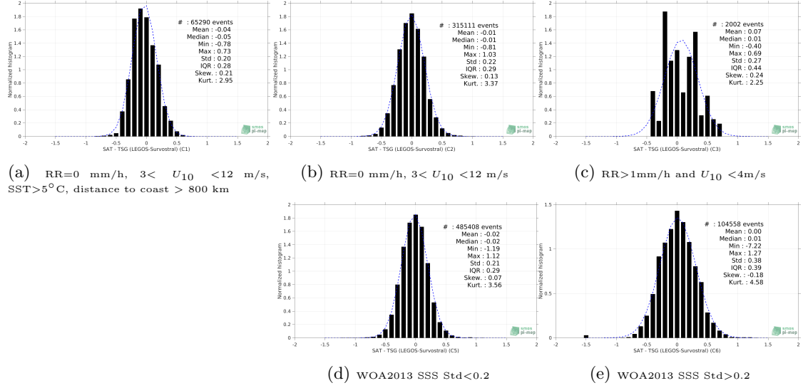
Figure 13: Normalized histogram of \Delta SSS (SMOS SSS L3 v5 - 18 Days (CATDS-CECOS-LOCEAN) - TSG (LEGOS-Survostral)) for 5 different subdatasets corresponding to: RR=0 mm/h, 3 < U_{10} < 12 m/s, SST>5°C, distance to coast > 800 km (a), RR=0 mm/h, 3 < U_{10} < 12 m/s (b), RR>1mm/h and U_{10} < 4 m/s (c), WOA2013 SSS Std<0.2 (d), WOA2013 SSS Std>0.2 (e).
