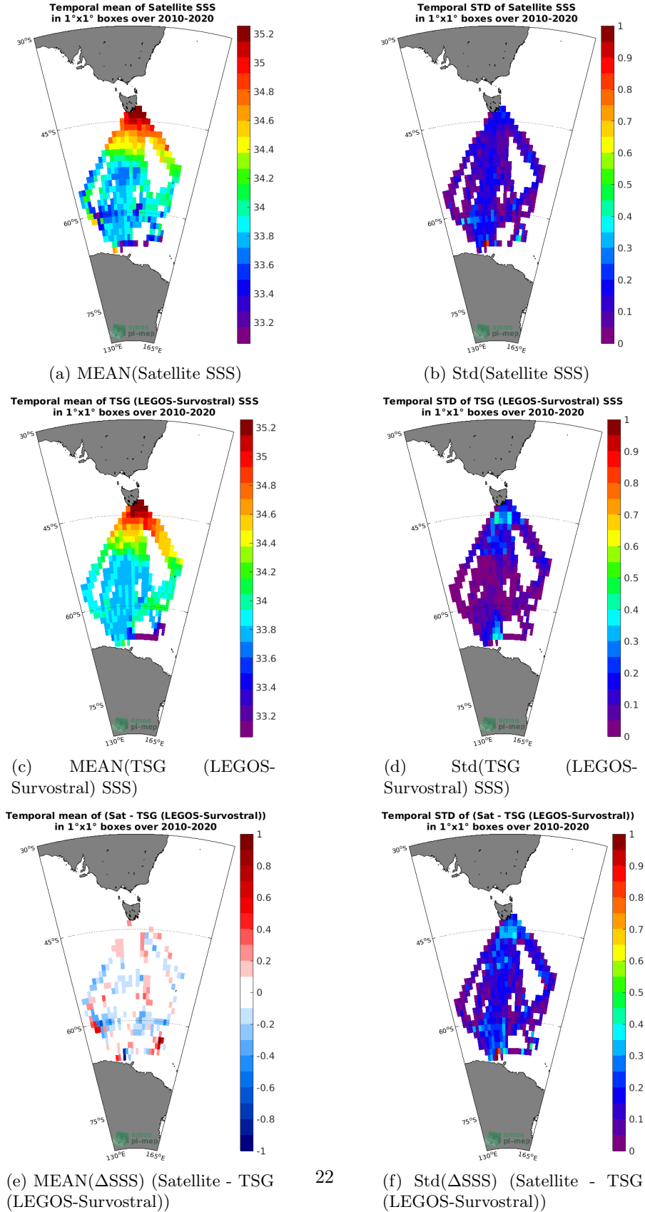
Figure 6: Temporal mean (left) and Std (right) of SSS from SMOS SSS L3 v5 - 18 Days (CATDS-CECOS-LOCEAN) (top), TSG (LEGOS-Survostral) (middle), and of \Delta SSS (Satellite - TSG (LEGOS-Survostral)). Only match-up pairs are used to generate these maps.
