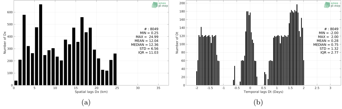
Figure 5: Histograms of the spatial (a) and temporal (b) lags between the location/time of the TSG (LEGOS-Surv-Adel) measurement and the date of the corresponding SMOS SSS L3 v5 - 18 Days (CATDS-CECOS-LOCEAN) SSS pixel.
