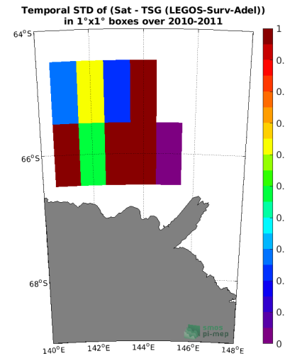
(f) Std( \Delta SSS) (Satellite - TSG (LEGOS-Surv-Adel))
