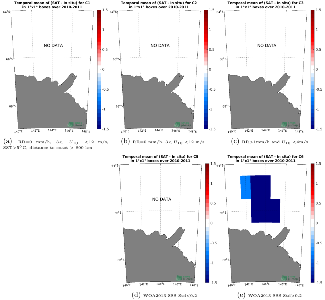
Figure 12: Temporal mean gridded over spatial boxes of size 1°x1° of \Delta SSS (SMOS SSS L3 v5 - 18 Days (CATDS-CECOS-LOCEAN) - TSG (LEGOS-Surv-Adel)) for 5 different subdatasets corresponding to: RR=0 mm/h, 3 < U_{10} < 12 m/s, SST>5°C, distance to coast > 800 km (a), RR=0 mm/h, 3 < U_{10} < 12 m/s (b), RR>1mm/h and U_{10} < 4 m/s (c), WOA2013 SSS Std<0.2 (d), WOA2013 SSS Std>0.2 (e).
