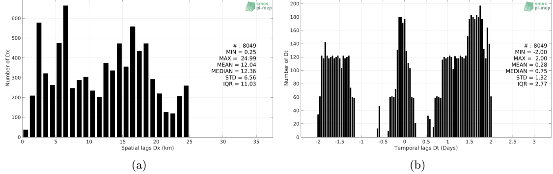
Figure 5: Histograms of the spatial (a) and temporal (b) lags between the time of the TSG (LEGOS-Surv-Adel) measurements and the date of the corresponding SMOS SSS L3 v5 - 18 Days (CATDS-CECOS-LOCEAN) SSS product.
