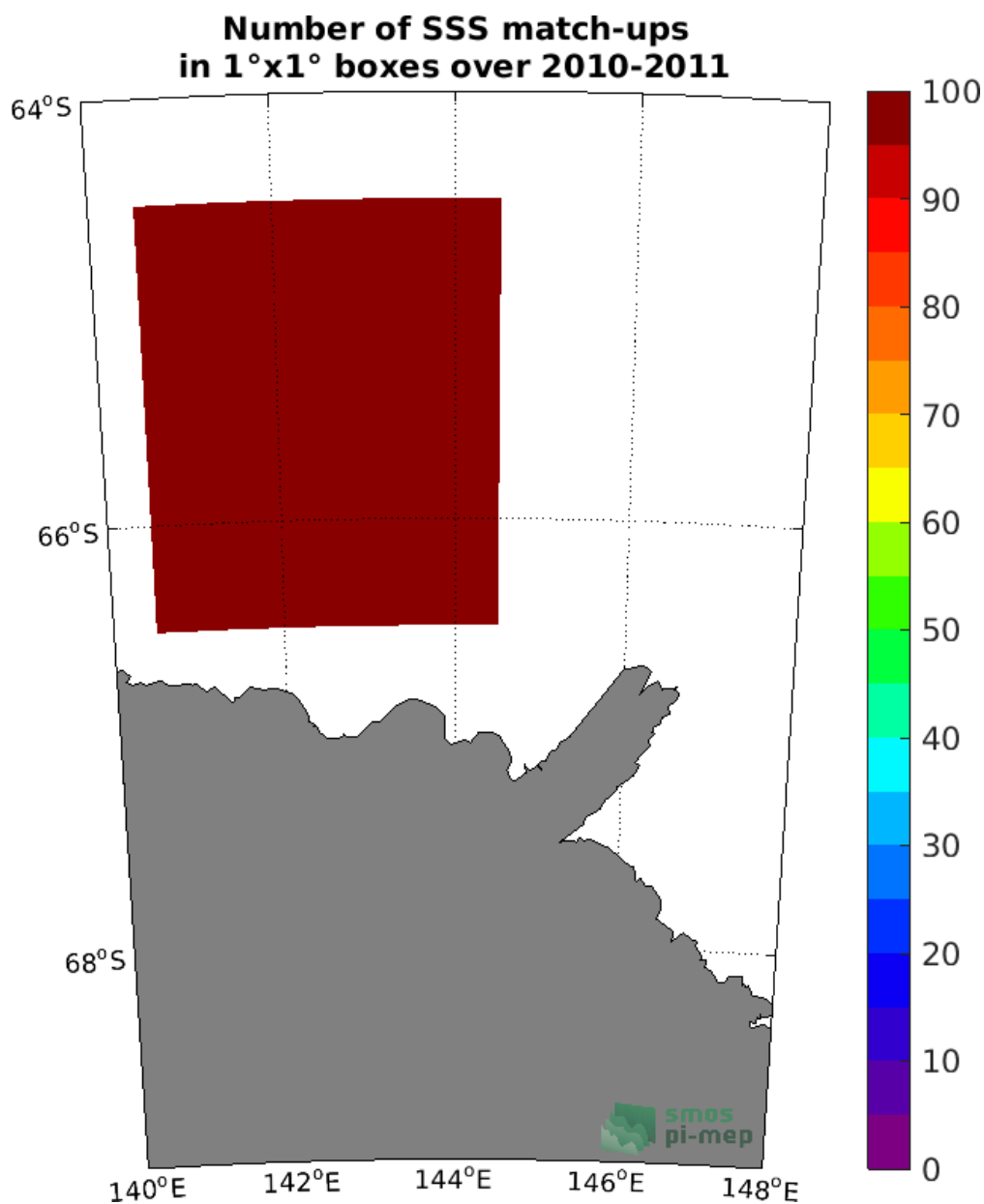
Figure 4: Number of SSS match-ups between TSG (LEGOS-Surv-Adel) SSS and the SMOS SSS L3 v5 - 18 Days (CATDS-CECOS-LOCEAN) SSS product for the Global Ocean Pi-MEP region over 1°x1° boxes and for the full satellite product period.
