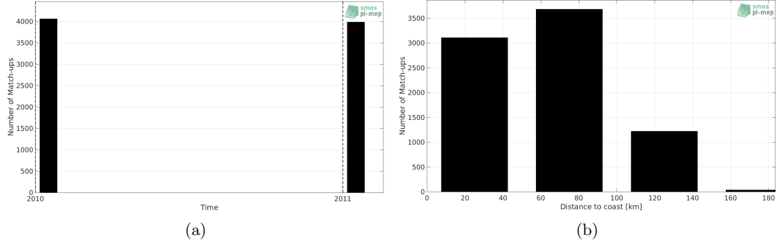
Figure 1: Number of match-ups between TSG (LEGOS-Surv-Adel) and SMOS SSS L3 v5 - 18 Days (CATDS-CECOS-LOCEAN) SSS as a function of time (a) and as function of the distance to coast (b) over the Global Ocean Pi-MEP region and for the full satellite product period.
