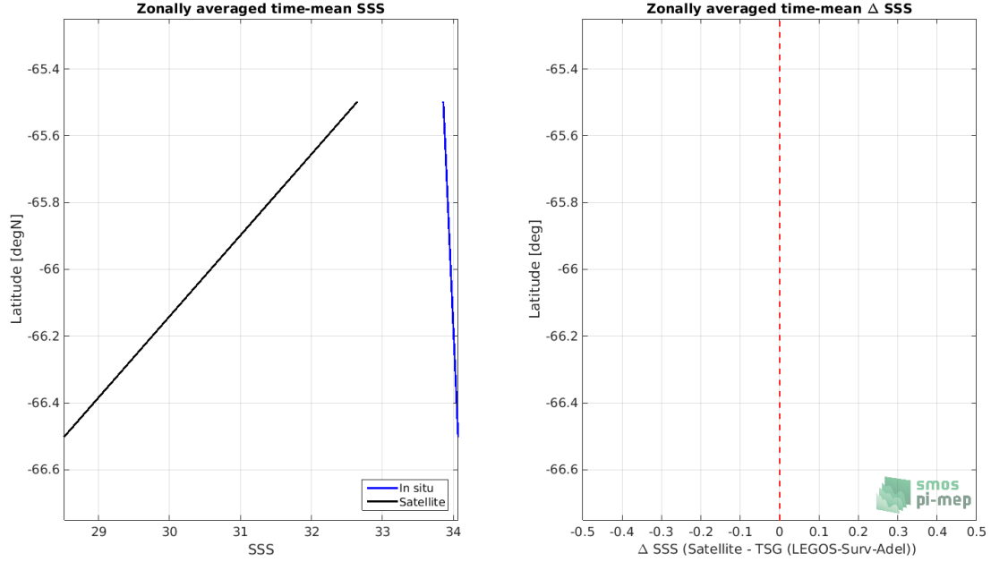
Figure 8: Left panel: Zonal mean SSS from SMOS SSS L3 v5 - 18 Days (CATDS-CECOS-LOCEAN) satellite product (black) and from TSG (LEGOS-Surv-Adel) (blue). Right panel: Zonal mean of \Delta SSS (Satellite - TSG (LEGOS-Surv-Adel)) for all the collected Pi-MEP match-up pairs estimated over the full satellite product period.
