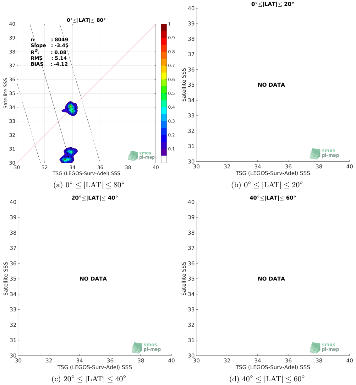
Figure 9: Contour maps of the concentration of SMOS SSS L3 v5 - 18 Days (CATDS-CECOS-LOCEAN) SSS (y-axis) versus TSG (LEGOS-Surv-Adel) SSS (x-axis) at match-up pairs for different latitude bands. For each plot, the red line shows x=y . The black thin and dashed lines indicate a linear fit through the data cloud and the \pm 95\% confidence levels, respectively. The number match-up pairs n , the slope and R^2 coefficient of the linear fit, the root mean square (RMS) and the mean bias between satellite and in situ data are indicated for each latitude band in each plots.
