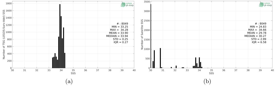
Figure 2: Histograms of SSS from TSG (LEGOS-Surv-Adel) (a) and SMOS SSS L3 v5 - 18 Days (CATDS-CECOS-LOCEAN) (b) considering all match-up pairs per bins of 0.1 over the Global Ocean Pi-MEP region and for the full satellite product period.
