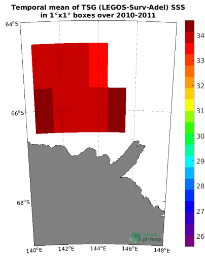
(c) MEAN(TSG (LEGOS-Surv-Adel) SSS)
