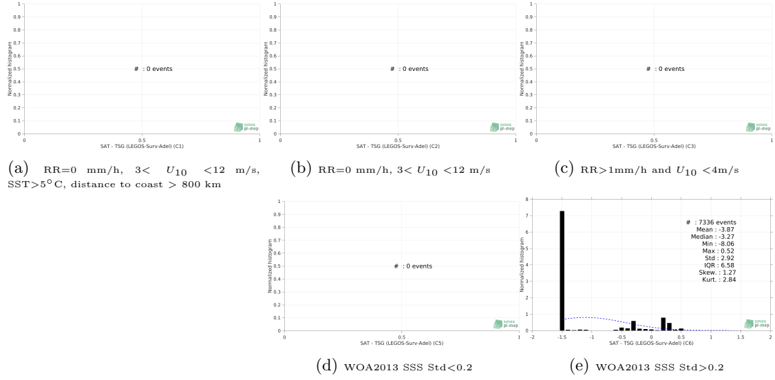
Figure 13: Normalized histogram of \Delta\text{SSS} (SMOS SSS L3 v5 - 18 Days (CATDS-CECOS-LOCEAN) - TSG (LEGOS-Surv-Adel)) for 5 different subdatasets corresponding to: RR=0 mm/h, 3 < U_{10} < 12 m/s, SST > 5^\circ\text{C} , distance to coast > 800 km (a), RR=0 mm/h, 3 < U_{10} < 12 m/s (b), RR > 1\text{mm/h} and U_{10} < 4\text{m/s} (c), WOA2013 SSS Std < 0.2 (d), WOA2013 SSS Std > 0.2 (e).
