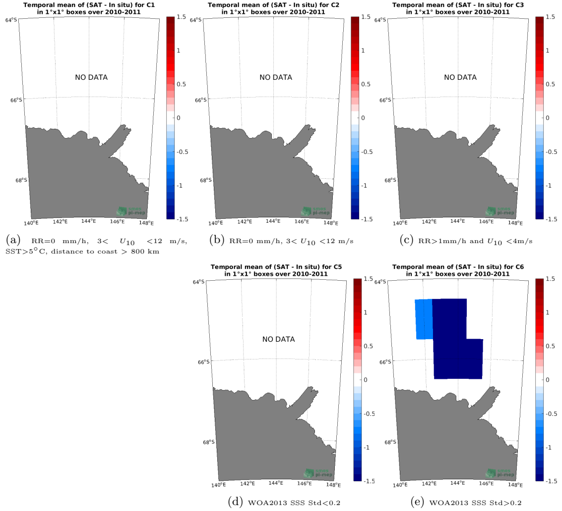
Figure 12: Temporal mean gridded over spatial boxes of size 1°x1° of \Delta\text{SSS} (SMOS SSS L3 v5 - 18 Days (CATDS-CECOS-LOCEAN) - TSG (LEGOS-Surv-Adel)) for 5 different subdatasets corresponding to: RR=0 mm/h, 3 < U_{10} < 12 m/s, SST > 5^\circ\text{C} , distance to coast > 800 km (a), RR=0 mm/h, 3 < U_{10} < 12 m/s (b), RR > 1 mm/h and U_{10} < 4 m/s (c), WOA2013 SSS Std < 0.2 (d), WOA2013 SSS Std > 0.2 (e).
