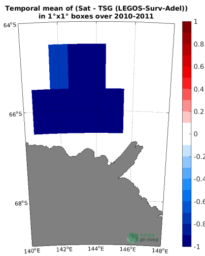
(e) MEAN( \Delta SSS) (Satellite - TSG (LEGOS-Surv-Adel))
