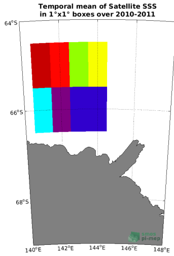
(a) MEAN(Satellite SSS)
