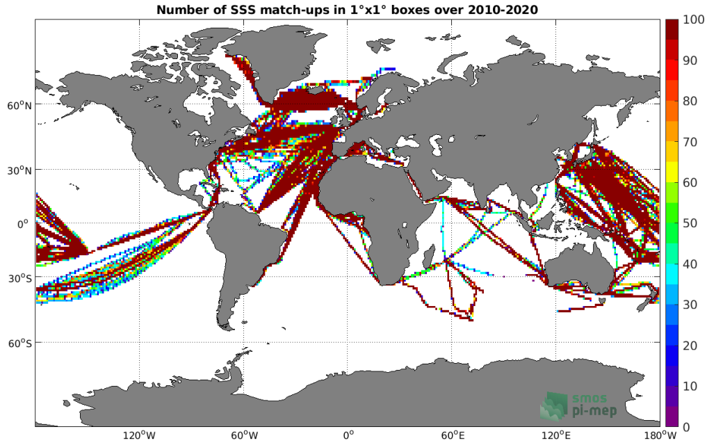
Figure 4: Number of SSS match-ups between TSG (LEGOS-DM) SSS and the SMOS SSS L3 v5 - 18 Days (CATDS-CECOS-LOCEAN) SSS product for the Global Ocean Pi-MEP region over 1^\circ \times 1^\circ boxes and for the full satellite product period.
