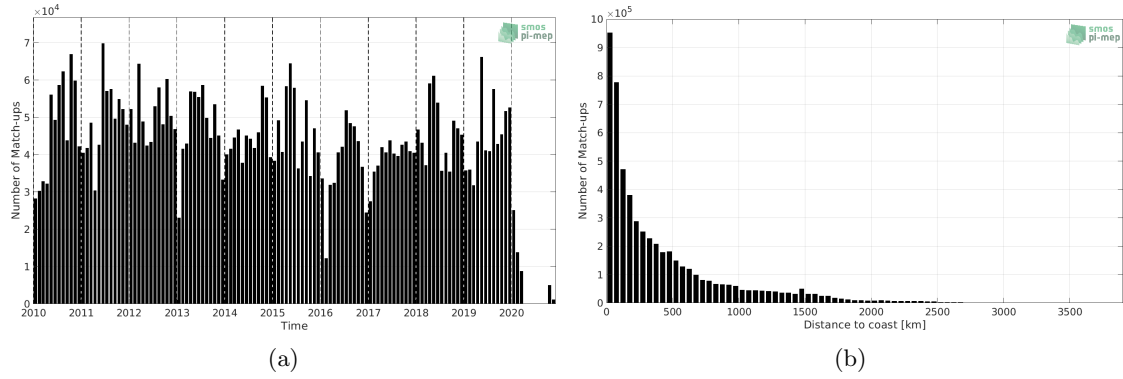
Figure 1: Number of match-ups between TSG (LEGOS-DM) and SMOS SSS L3 v5 - 18 Days (CATDS-CECOS-LOCEAN) SSS as a function of time (a) and as function of the distance to coast (b) over the Global Ocean Pi-MEP region and for the full satellite product period.
