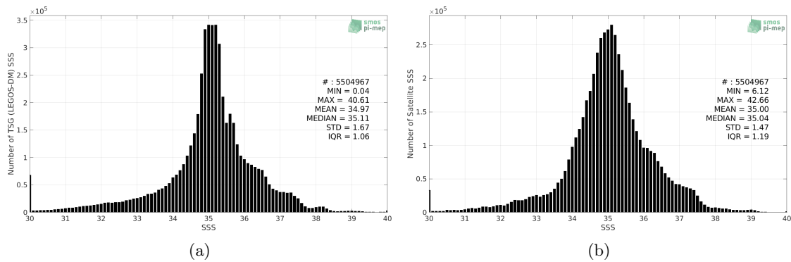
Figure 2: Histograms of SSS from TSG (LEGOS-DM) (a) and SMOS SSS L3 v5 - 18 Days (CATDS-CECOS-LOCEAN) (b) considering all match-up pairs per bins of 0.1 over the Global Ocean Pi-MEP region and for the full satellite product period.
