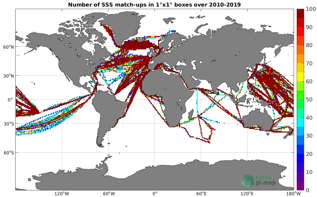
Figure 4: Number of SSS match-ups between TSG (LEGOS-DM) SSS and the SMOS SSS L3 v5 - 18 Days (CATDS-CECOS-LOCEAN) SSS product for the Global Ocean Pi-MEP region over 1°x1° boxes and for the full satellite product period.
