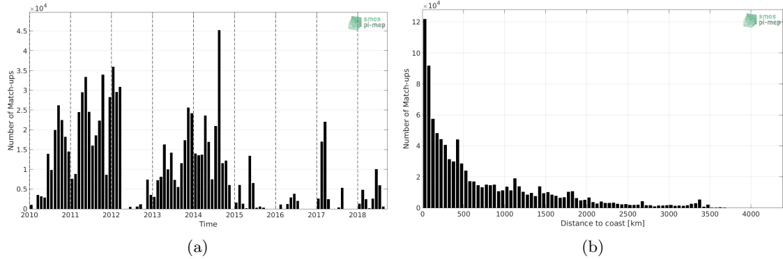
Figure 1: Number of match-ups between TSG (GOSUD-Sailing-ship) and SMOS SSS L3 v5 - 18 Days (CATDS-CECOS-LOCEAN) SSS as a function of time (a) and as function of the distance to coast (b) over the Global Ocean Pi-MEP region and for the full satellite product period.
