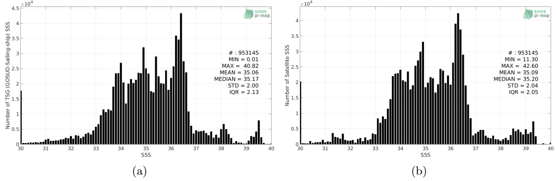
Figure 2: Histograms of SSS from TSG (GOSUD-Sailing-ship) (a) and SMOS SSS L3 v5 - 18 Days (CATDS-CECOS-LOCEAN) (b) considering all match-up pairs per bins of 0.1 over the Global Ocean Pi-MEP region and for the full satellite product period.
