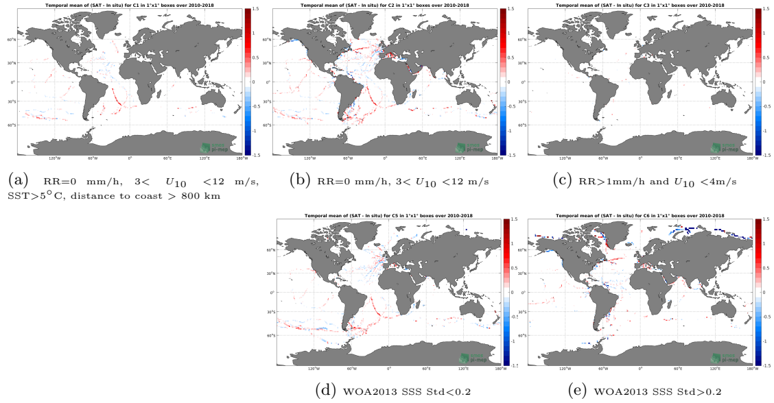
Figure 12: Temporal mean gridded over spatial boxes of size 1^\circ \times 1^\circ of \Delta SSS (SMOS SSS L3 v5 - 18 Days (CATDS-CECOS-LOCEAN) - TSG (GOSUD-Sailing-ship)) for 5 different subdatasets corresponding to:RR=0 mm/h, 3 < U_{10} < 12 m/s, SST>5°C, distance to coast > 800 km (a), RR=0 mm/h, 3 < U_{10} < 12 m/s (b), RR>1mm/h and U_{10} < 4 m/s (c), WOA2013 SSS Std<0.2 (d), WOA2013 SSS Std>0.2 (e).
