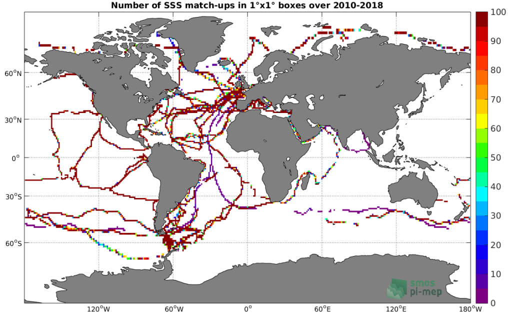
Figure 4: Number of SSS match-ups between TSG (GOSUD-Sailing-ship) SSS and the SMOS SSS L3 v5 - 18 Days (CATDS-CECOS-LOCEAN) SSS product for the Global Ocean Pi-MEP region over 1^\circ \times 1^\circ boxes and for the full satellite product period.
