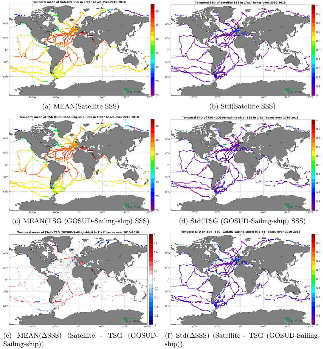
Figure 6: Temporal mean (left) and Std (right) of SSS from SMOS SSS L3 v5 - 18 Days (CATDS-CECOS-LOCEAN) (top), TSG (GOSUD-Sailing-ship) (middle), and of \Delta SSS (Satellite - TSG (GOSUD-Sailing-ship)). Only match-up pairs are used to generate these maps.
