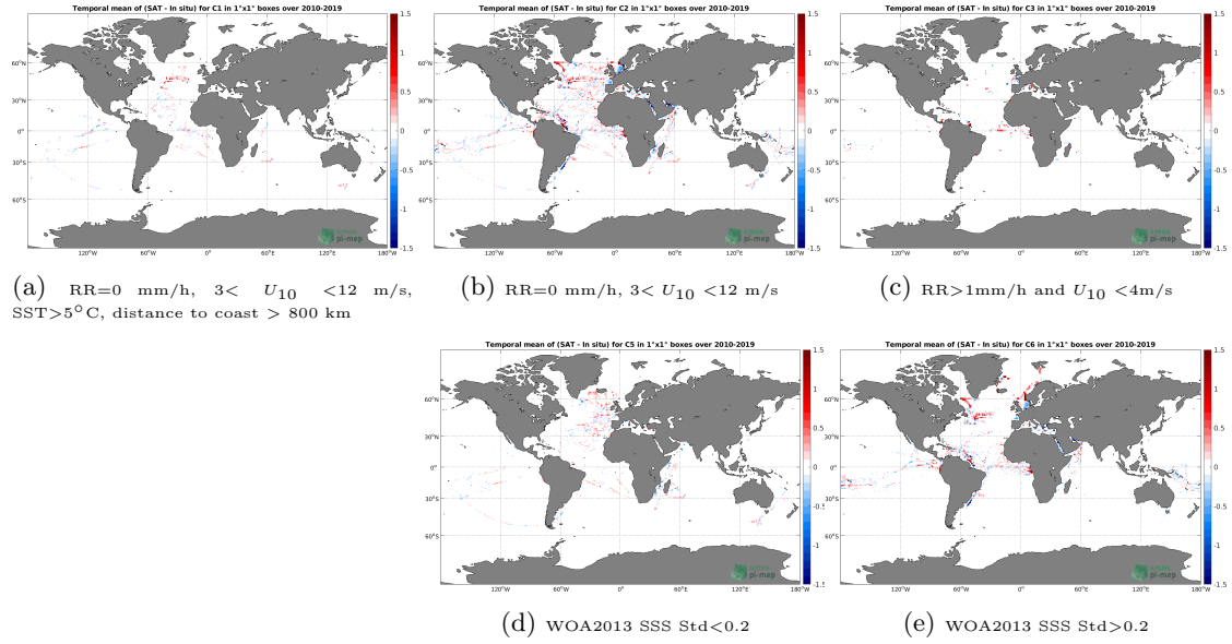
Figure 12: Temporal mean gridded over spatial boxes of size 1^\circ \times 1^\circ of \Delta SSS (SMOS SSS L3 v5 - 18 Days (CATDS-CECOS-LOCEAN) - TSG (GOSUD-Research-vessel)) for 5 different subdatasets corresponding to:RR=0 mm/h, 3 < U_{10} < 12 m/s, SST>5°C, distance to coast > 800 km (a), RR=0 mm/h, 3 < U_{10} < 12 m/s (b), RR>1mm/h and U_{10} < 4 m/s (c), WOA2013 SSS Std<0.2 (d), WOA2013 SSS Std>0.2 (e).
