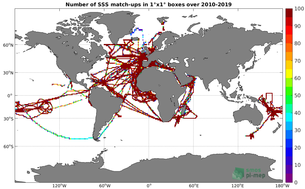
Figure 4: Number of SSS match-ups between TSG (GOSUD-Research-vessel) SSS and the SMOS SSS L3 v5 - 18 Days (CATDS-CECOS-LOCEAN) SSS product for the Global Ocean Pi-MEP region over 1^\circ \times 1^\circ boxes and for the full satellite product period.
