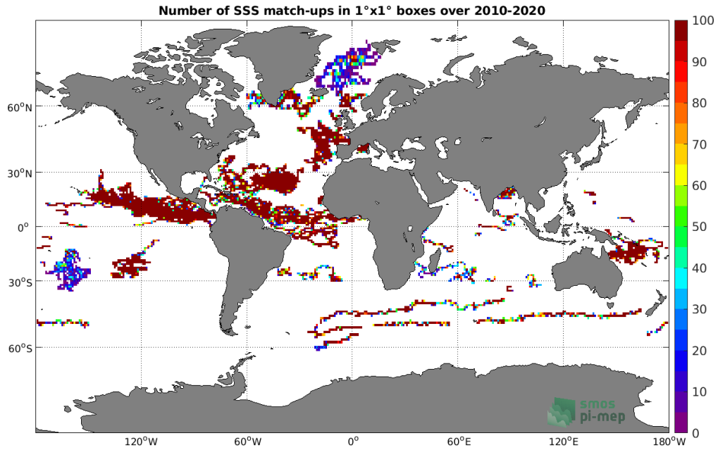
Figure 3: Number of SSS match-ups between Surface drifters SSS and the SMOS SSS L3 v5 - 18 Days (CATDS-CECOS-LOCEAN) SSS product for the Global Ocean Pi-MEP region over 1^\circ \times 1^\circ boxes and for the full satellite product period.
