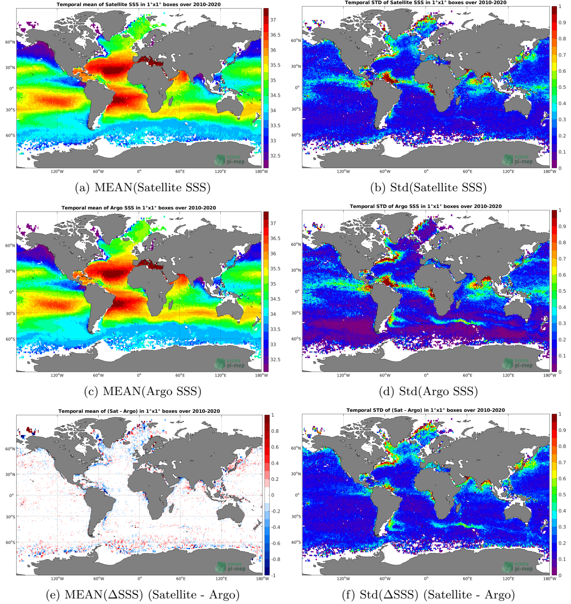
Figure 6: Temporal mean (left) and Std (right) of SSS from SMOS SSS L3 v5 - 18 Days (CATDS-CECOS-LOCEAN) (top), Argo (middle), and of \Delta SSS (Satellite - Argo). Only match-up pairs are used to generate these maps.
