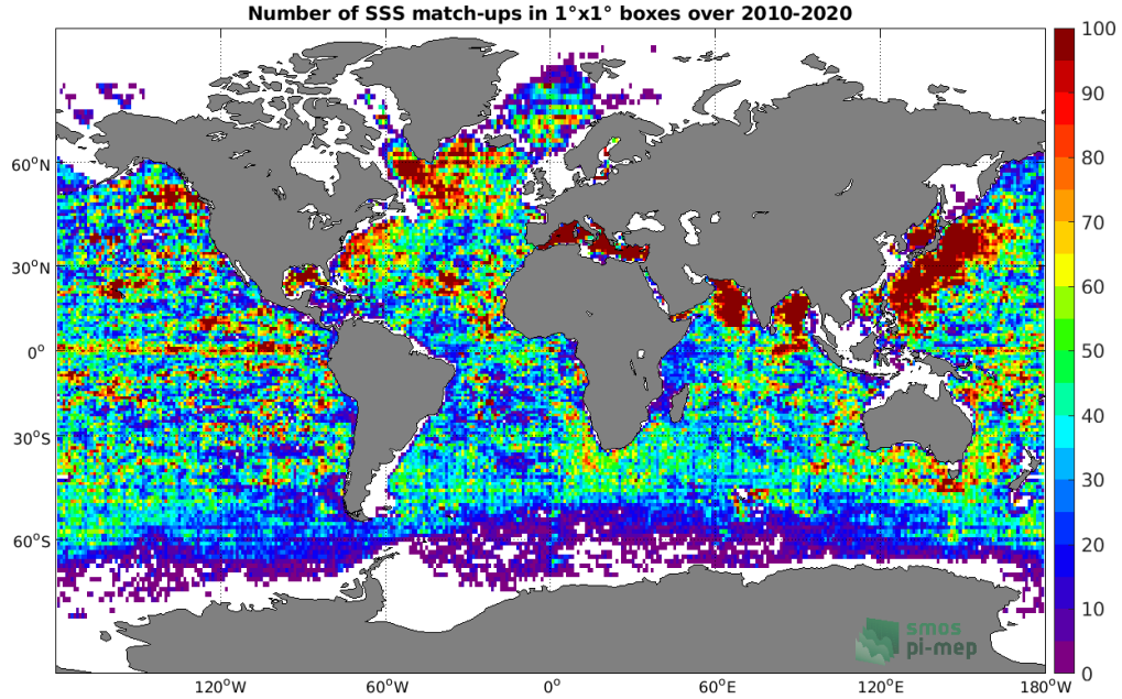
Figure 4: Number of SSS match-ups between Argo SSS and the SMOS SSS L3 v5 - 18 Days (CATDS-CECOS-LOCEAN) SSS product for the Global Ocean Pi-MEP region over 1^\circ \times 1^\circ boxes and for the full satellite product period.
