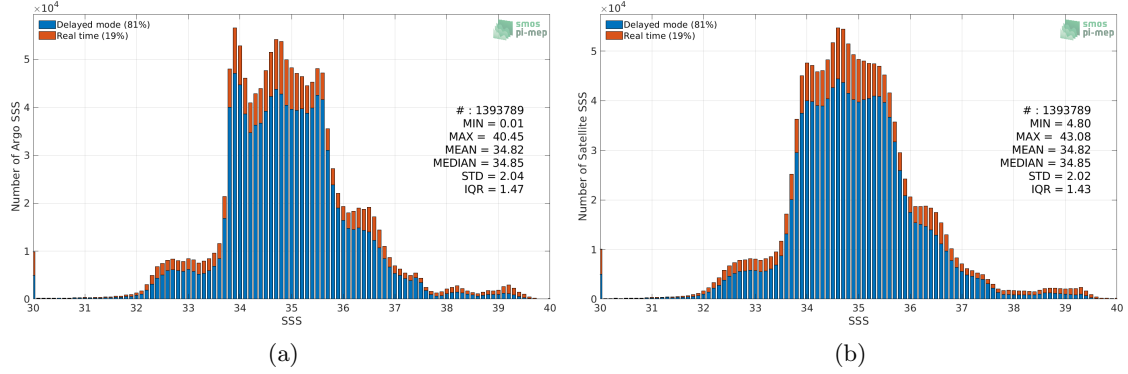
Figure 2: Histograms of SSS from Argo (a) and SMOS SSS L3 v5 - 18 Days (CATDS-CECOS-LOCEAN) (b) considering all match-up pairs per bins of 0.1 over the Global Ocean Pi-MEP region and for the full satellite product period.
