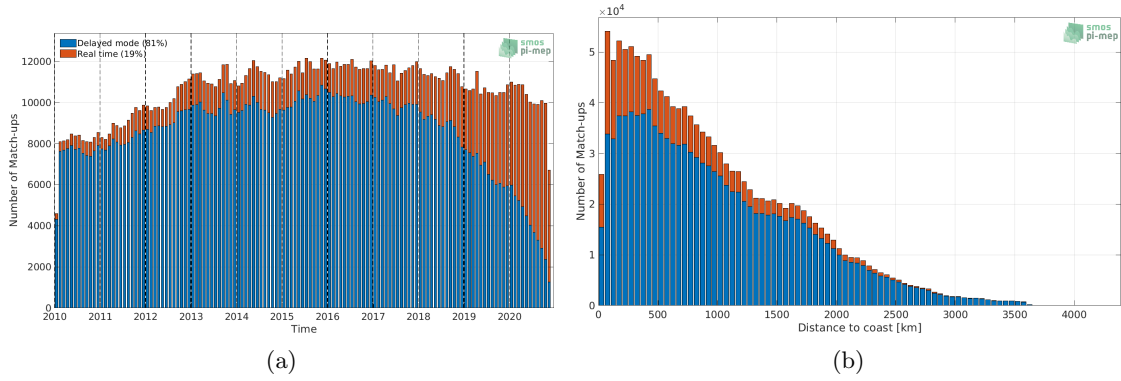
Figure 1: Number of match-ups between Argo and SMOS SSS L3 v5 - 18 Days (CATDS-CECOS-LOCEAN) SSS as a function of time (a) and as function of the distance to coast (b) over the Global Ocean Pi-MEP region and for the full satellite product period.
