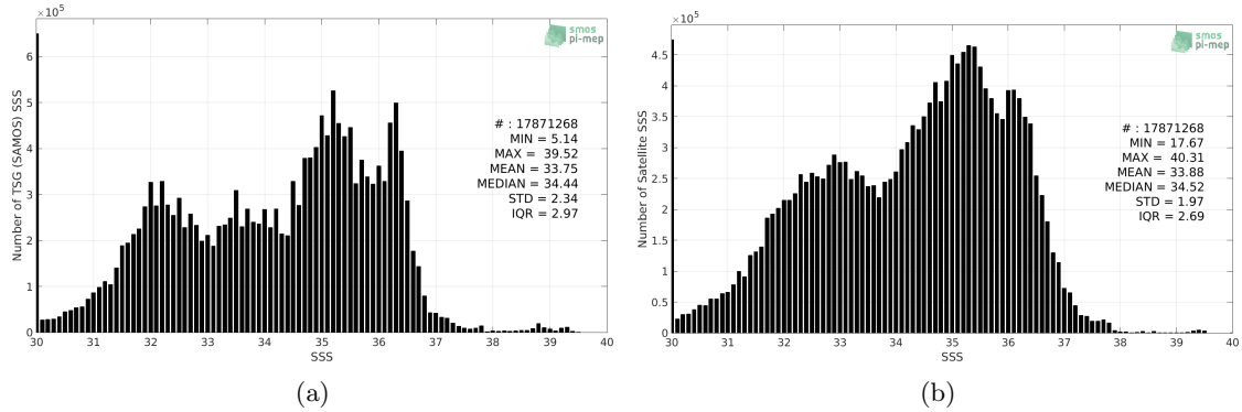
Figure 2: Histograms of SSS from TSG (SAMOS) (a) and SMOS SSS L3 v4 - 9 Days (CATDS-CECOS-LOCEAN) (b) considering all match-up pairs per bins of 0.1 over the Global Ocean Pi-MEP region and for the full satellite product period.
