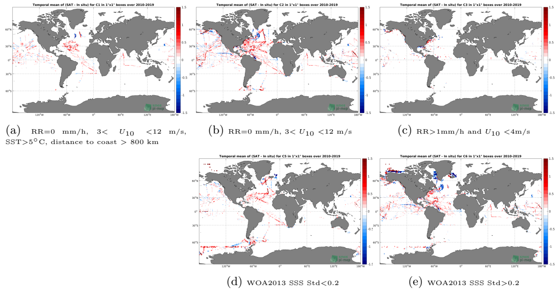
Figure 12: Temporal mean gridded over spatial boxes of size 1^\circ \times 1^\circ of \Delta SSS (SMOS SSS L3 v4 - 9 Days (CATDS-CECOS-LOCEAN) - TSG (SAMOS)) for 5 different subdatasets corresponding to: RR=0 mm/h, 3 < U_{10} < 12 m/s, SST > 5^\circ C , distance to coast > 800 km (a), RR=0 mm/h, 3 < U_{10} < 12 m/s (b), RR > 1 mm/h and U_{10} < 4 m/s (c), WOA2013 SSS Std < 0.2 (d), WOA2013 SSS Std > 0.2 (e).
