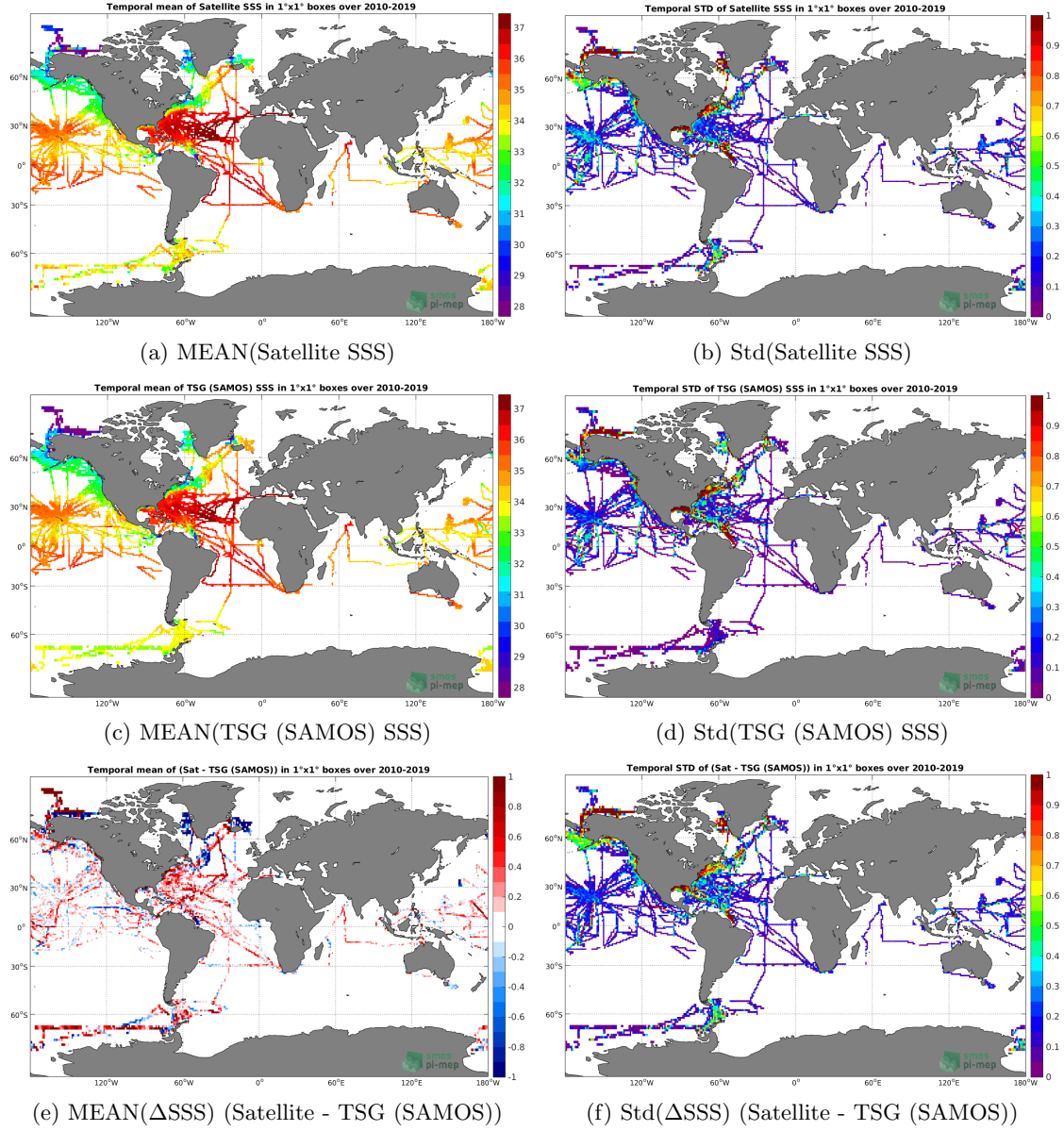
Figure 6: Temporal mean (left) and Std (right) of SSS from SMOS SSS L3 v4 - 9 Days (CATDS-CECOS-LOCEAN) (top), TSG (SAMOS) (middle), and of \Delta SSS (Satellite - TSG (SAMOS)). Only match-up pairs are used to generate these maps.
