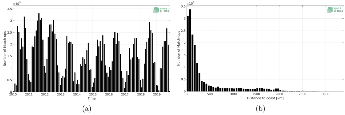
Figure 1: Number of match-ups between TSG (SAMOS) and SMOS SSS L3 v4 - 9 Days (CATDS-CECOS-LOCEAN) SSS as a function of time (a) and as function of the distance to coast (b) over the Global Ocean Pi-MEP region and for the full satellite product period.
