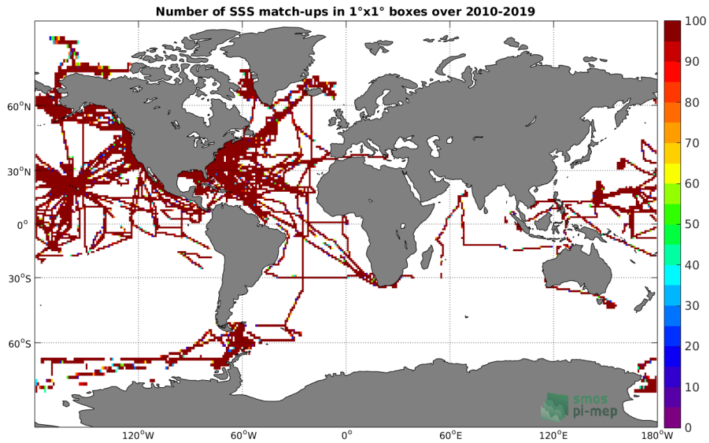
Figure 4: Number of SSS match-ups between TSG (SAMOS) SSS and the SMOS SSS L3 v4 - 9 Days (CATDS-CECOS-LOCEAN) SSS product for the Global Ocean Pi-MEP region over 1°x1° boxes and for the full satellite product period.
