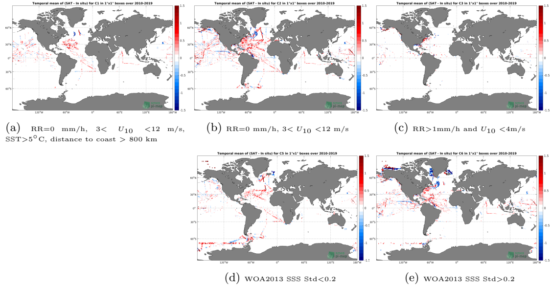
Figure 12: Temporal mean gridded over spatial boxes of size 1^\circ \times 1^\circ of \Delta SSS (SMOS-L3-CATDS-CECOS-LOCEAN-V4-9DAYS-25KM - TSG-SAMOS) for 5 different subdatasets corresponding to: RR=0 mm/h, 3 < U_{10} < 12 m/s, SST >5^\circ C, distance to coast > 800 km (a), RR=0 mm/h, 3 < U_{10} < 12 m/s (b), RR >1 mm/h and U_{10} < 4 m/s (c), WOA2013 SSS Std <0.2 (d), WOA2013 SSS Std >0.2 (e).
