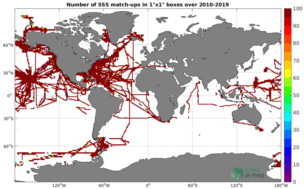
Figure 4: Number of SSS match-ups between TSG-SAMOS SSS and the SMOS-L3-CATDS-CECOS-LOCEAN-V4-9DAYS-25KM SSS product for the Global Ocean Pi-MEP region over 1°x1° boxes and for the full satellite product period.
