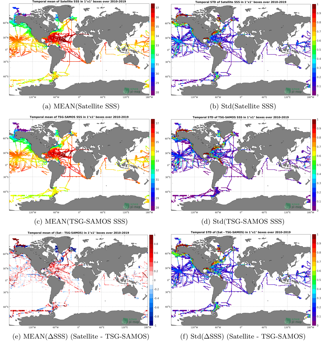
Figure 6: Temporal mean (left) and Std (right) of SSS from SMOS-L3-CATDS-CECOS-LOCEAN-V4-9DAYS-25KM (top), TSG-SAMOS (middle), and of \Delta SSS (Satellite - TSG-SAMOS). Only match-up pairs are used to generate these maps.
