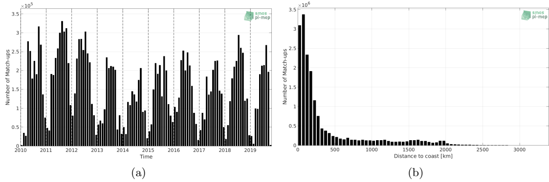
Figure 1: Number of match-ups between TSG-SAMOS and SMOS-L3-CATDS-CECOS-LOCEAN-V4-9DAYS-25KM SSS as a function of time (a) and as function of the distance to coast (b) over the Global Ocean Pi-MEP region and for the full satellite product period.
