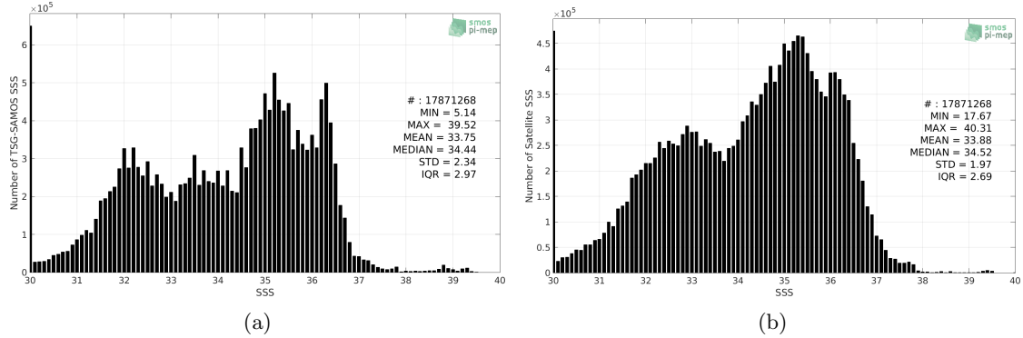
Figure 2: Histograms of SSS from TSG-SAMOS (a) and SMOS-L3-CATDS-CECOS-LOCEAN-V4-9DAYS-25KM (b) considering all match-up pairs per bins of 0.1 over the Global Ocean Pi-MEP region and for the full satellite product period.
