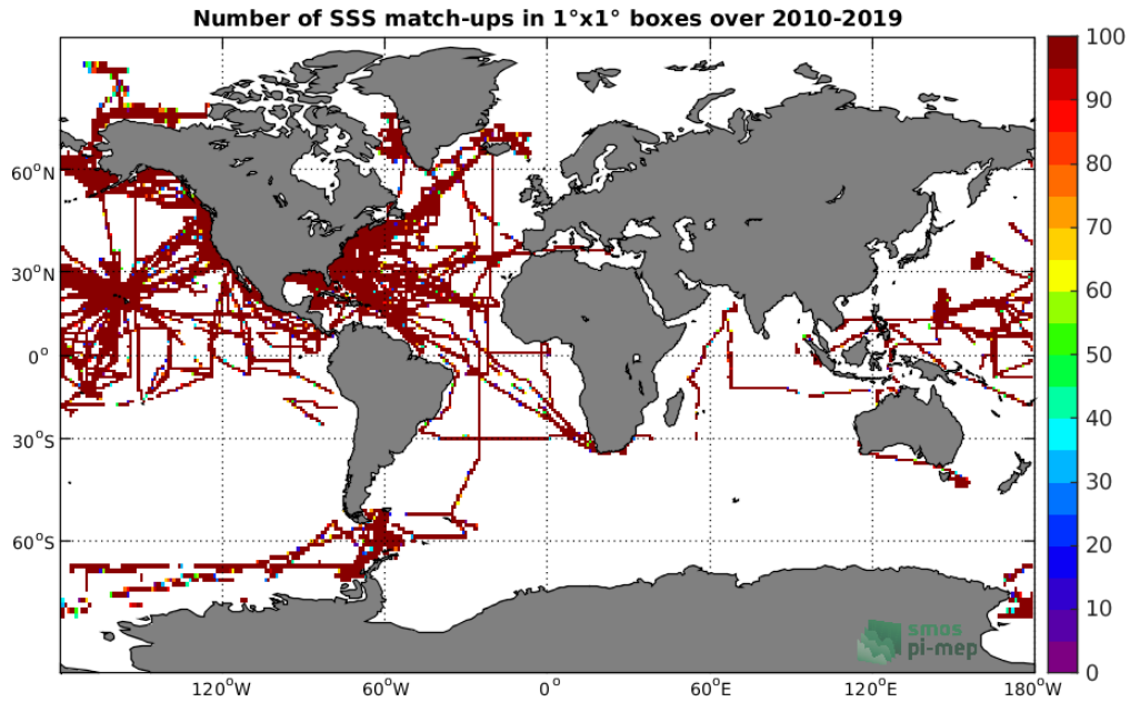
Figure 4: Number of SSS match-ups between TSG-SAMOS SSS and the SMOS-L3-CATDS-CECOS-LOCEAN-V4-9DAYS-25KM SSS product for the Global Ocean Pi-MEP region over 1^\circ \times 1^\circ boxes and for the full satellite product period.
