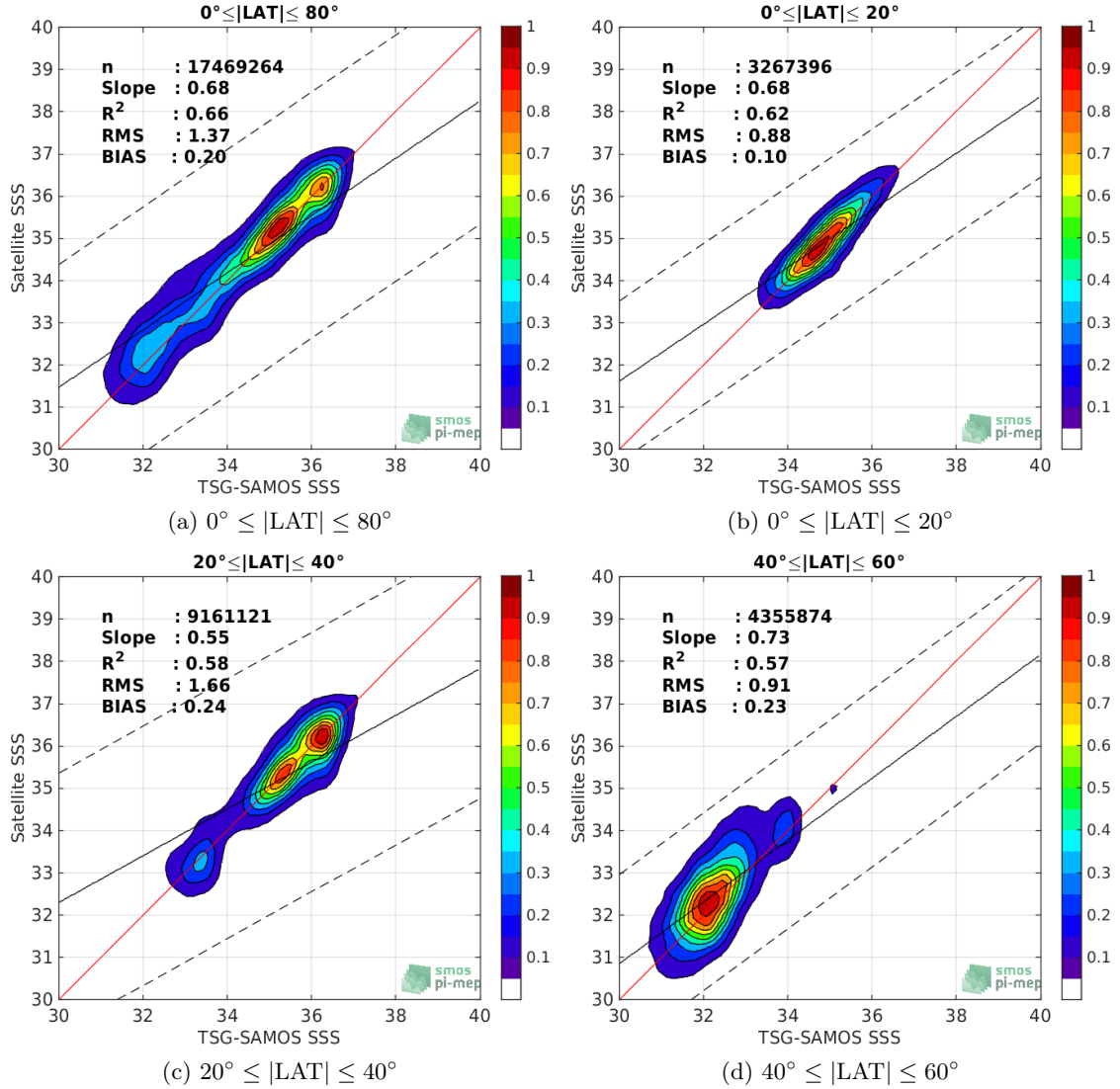
Figure 9: Contour maps of the concentration of SMOS-L3-CATDS-CECOS-LOCEAN-V4-9DAYS-25KM SSS (y-axis) versus TSG-SAMOS SSS (x-axis) at match-up pairs for different latitude bands. For each plot, the red line shows x=y . The black thin and dashed lines indicate a linear fit through the data cloud and the \pm 95\% confidence levels, respectively. The number match-up pairs n , the slope and R^2 coefficient of the linear fit, the root mean square (RMS) and the mean bias between satellite and in situ data are indicated for each latitude band in each plots.
