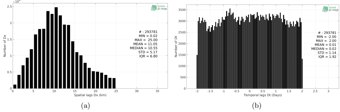
Figure 5: Histograms of the spatial (a) and temporal (b) lags between the time of the TSG (Polarstern) measurements and the date of the corresponding SMOS SSS L3 v4 - 9 Days (CATDS-CECOS-LOCEAN) SSS product.
