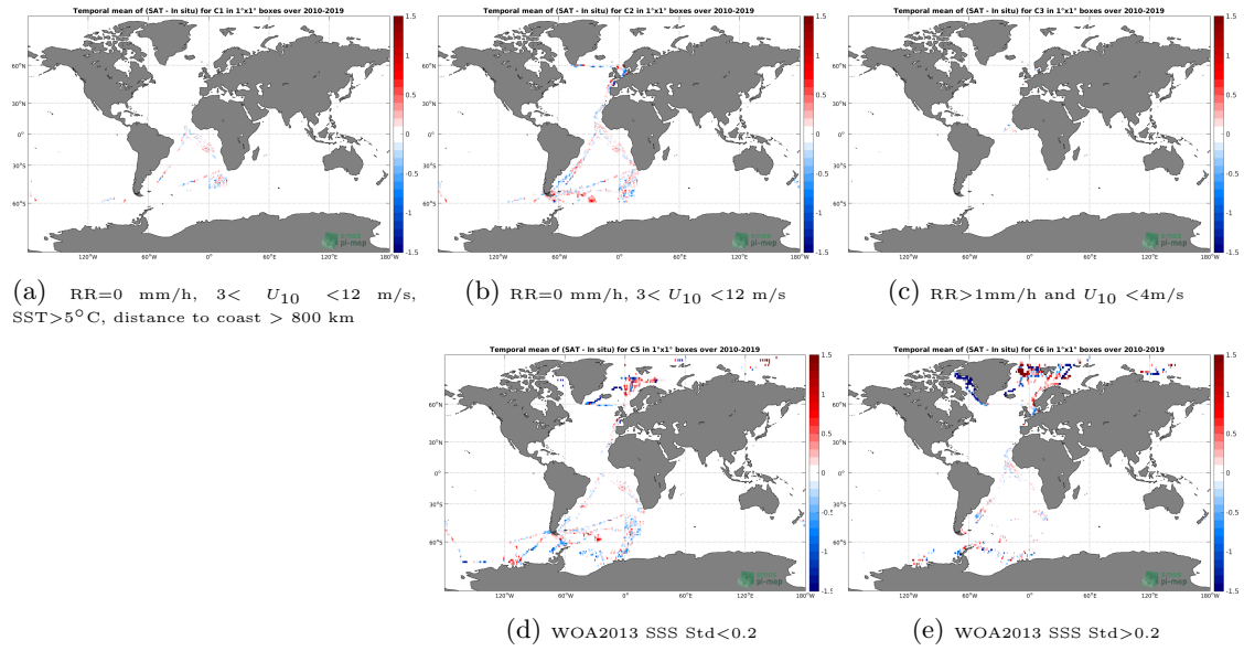
Figure 12: Temporal mean gridded over spatial boxes of size 1^\circ \times 1^\circ of \Delta SSS (SMOS SSS L3 v4 - 9 Days (CATDS-CECOS-LOCEAN) - TSG (Polarstern)) for 5 different subdatasets corresponding to: RR=0 mm/h, 3 < U_{10} < 12 m/s, SST > 5^\circ C , distance to coast > 800 km (a), RR=0 mm/h, 3 < U_{10} < 12 m/s (b), RR > 1 mm/h and U_{10} < 4 m/s (c), WOA2013 SSS Std < 0.2 (d), WOA2013 SSS Std > 0.2 (e).
