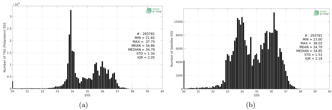
Figure 2: Histograms of SSS from TSG (Polarstern) (a) and SMOS SSS L3 v4 - 9 Days (CATDS-CECOS-LOCEAN) (b) considering all match-up pairs per bins of 0.1 over the Global Ocean Pi-MEP region and for the full satellite product period.
