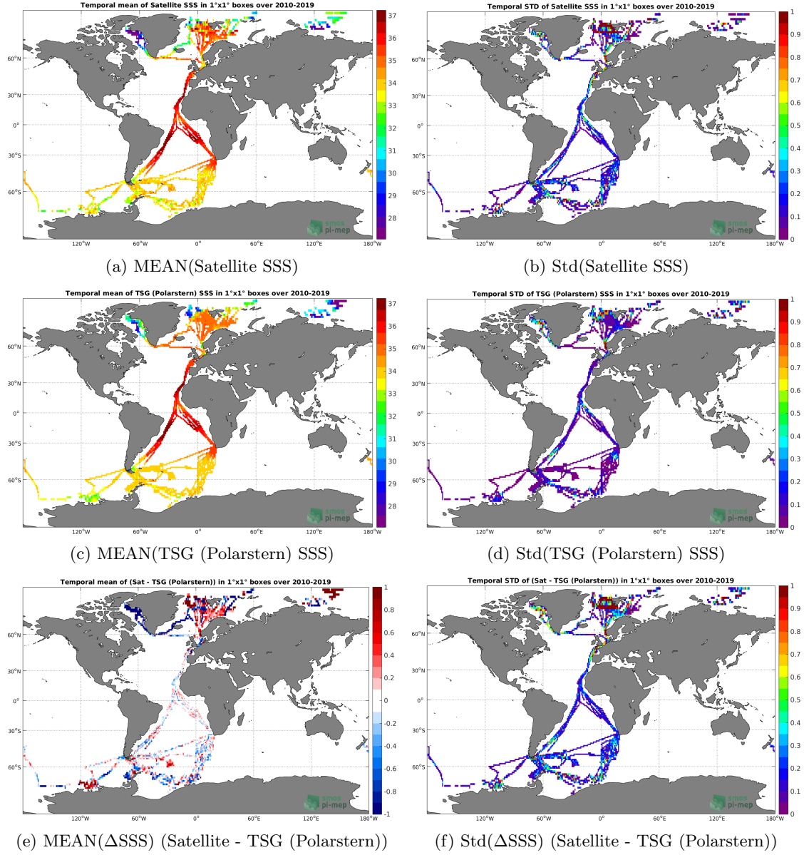
Figure 6: Temporal mean (left) and Std (right) of SSS from SMOS SSS L3 v4 - 9 Days (CATDS-CECOS-LOCEAN) (top), TSG (Polarstern) (middle), and of \Delta SSS (Satellite - TSG (Polarstern)). Only match-up pairs are used to generate these maps.
