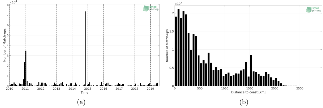
Figure 1: Number of match-ups between TSG (Polarstern) and SMOS SSS L3 v4 - 9 Days (CATDS-CECOS-LOCEAN) SSS as a function of time (a) and as function of the distance to coast (b) over the Global Ocean Pi-MEP region and for the full satellite product period.
