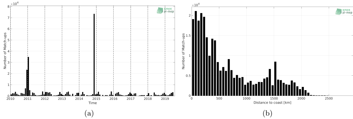
Figure 1: Number of match-ups between TSG-POLARSTERN and SMOS-L3-CATDS-CECOS-LOCEAN-V4-9DAYS-25KM SSS as a function of time (a) and as function of the distance to coast (b) over the Global Ocean Pi-MEP region and for the full satellite product period.
