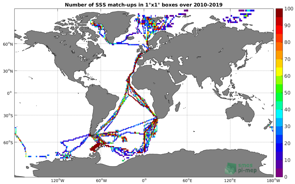
Figure 4: Number of SSS match-ups between TSG-POLARSTERN SSS and the SMOS-L3-CATDS-CECOS-LOCEAN-V4-9DAYS-25KM SSS product for the Global Ocean Pi-MEP region over 1^\circ \times 1^\circ boxes and for the full satellite product period.
