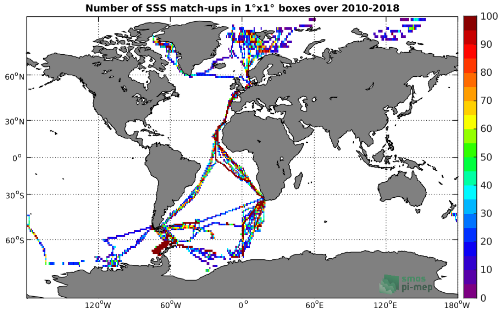
Figure 4: Number of SSS match-ups between TSG-POLARSTERN SSS and the SMOS-L3-CATDS-CECOS-LOCEAN-V4-9DAYS-25KM SSS product for the Global Ocean Pi-MEP region over 1°x1° boxes and for the full satellite product period.
