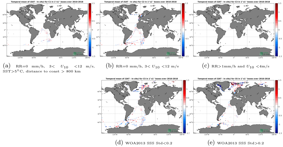
Figure 12: Temporal mean gridded over spatial boxes of size 1^\circ \times 1^\circ of \Delta SSS (SMOS-L3-CATDS-CECOS-LOCEAN-V4-9DAYS-25KM - TSG-POLARSTERN) for 5 different subdatasets corresponding to: RR=0 mm/h, 3 < U_{10} < 12 m/s, SST >5^\circ C, distance to coast > 800 km (a), RR=0 mm/h, 3 < U_{10} < 12 m/s (b), RR >1 mm/h and U_{10} < 4 m/s (c), WOA2013 SSS Std <0.2 (d), WOA2013 SSS Std >0.2 (e).
