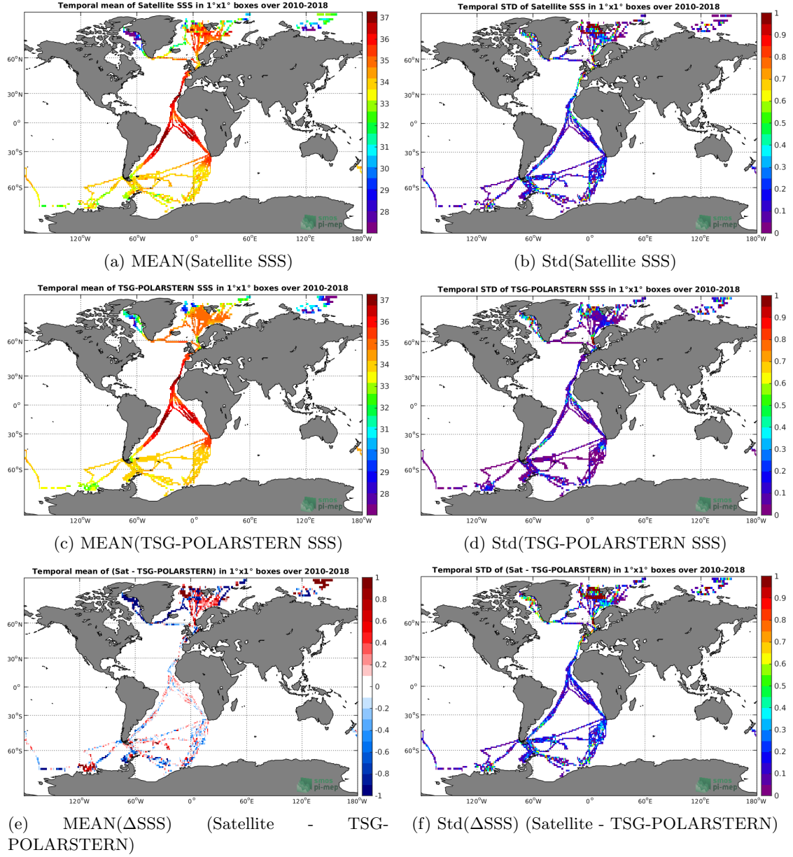
Figure 6: Temporal mean (left) and Std (right) of SSS from SMOS-L3-CATDS-CECOS-LOCEAN-V4-9DAYS-25KM (top), TSG-POLARSTERN (middle), and of \Delta SSS (Satellite - TSG-POLARSTERN). Only match-up pairs are used to generate these maps.
