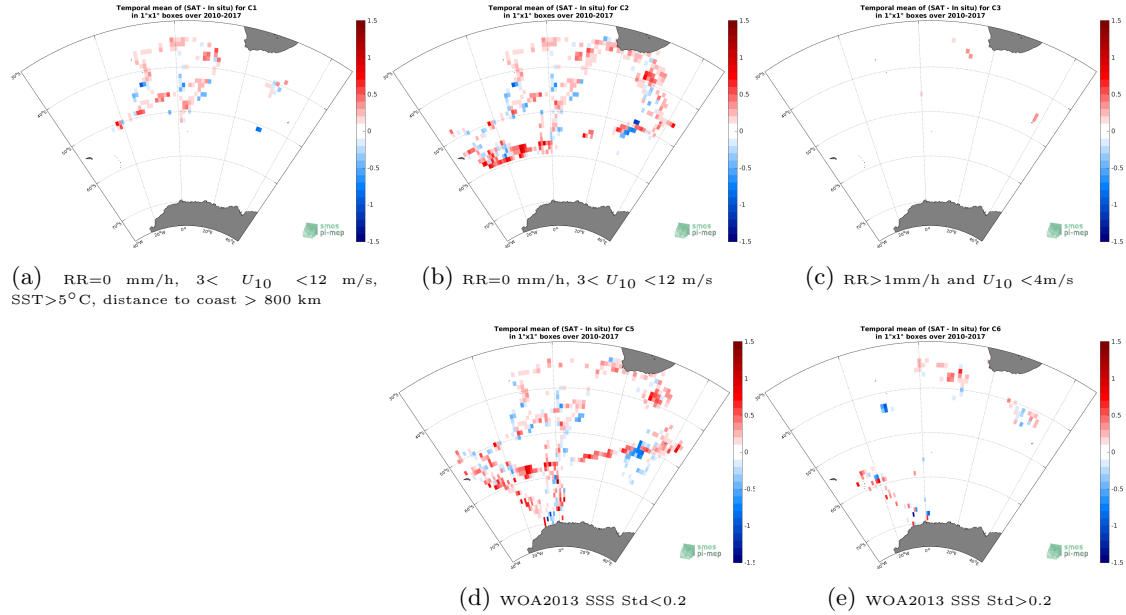
Figure 12: Temporal mean gridded over spatial boxes of size 1^{\circ}\times 1^{\circ} of \Delta\text{SSS} (SMOS SSS L3 v4 - 9 Days (CATDS-CECOS-LOCEAN) - TSG (NCEI-0170743)) for 5 different subdatasets corresponding to: RR=0 mm/h, 3 < U_{10} < 12 m/s, SST > 5^{\circ}\text{C} , distance to coast > 800 km (a), RR=0 mm/h, 3 < U_{10} < 12 m/s (b), RR > 1 mm/h and U_{10} < 4 m/s (c), WOA2013 SSS Std < 0.2 (d), WOA2013 SSS Std > 0.2 (e).
