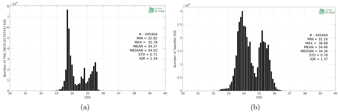
Figure 2: Histograms of SSS from TSG (NCEI-0170743) (a) and SMOS SSS L3 v4 - 9 Days (CATDS-CECOS-LOCEAN) (b) considering all match-up pairs per bins of 0.1 over the Global Ocean Pi-MEP region and for the full satellite product period.
