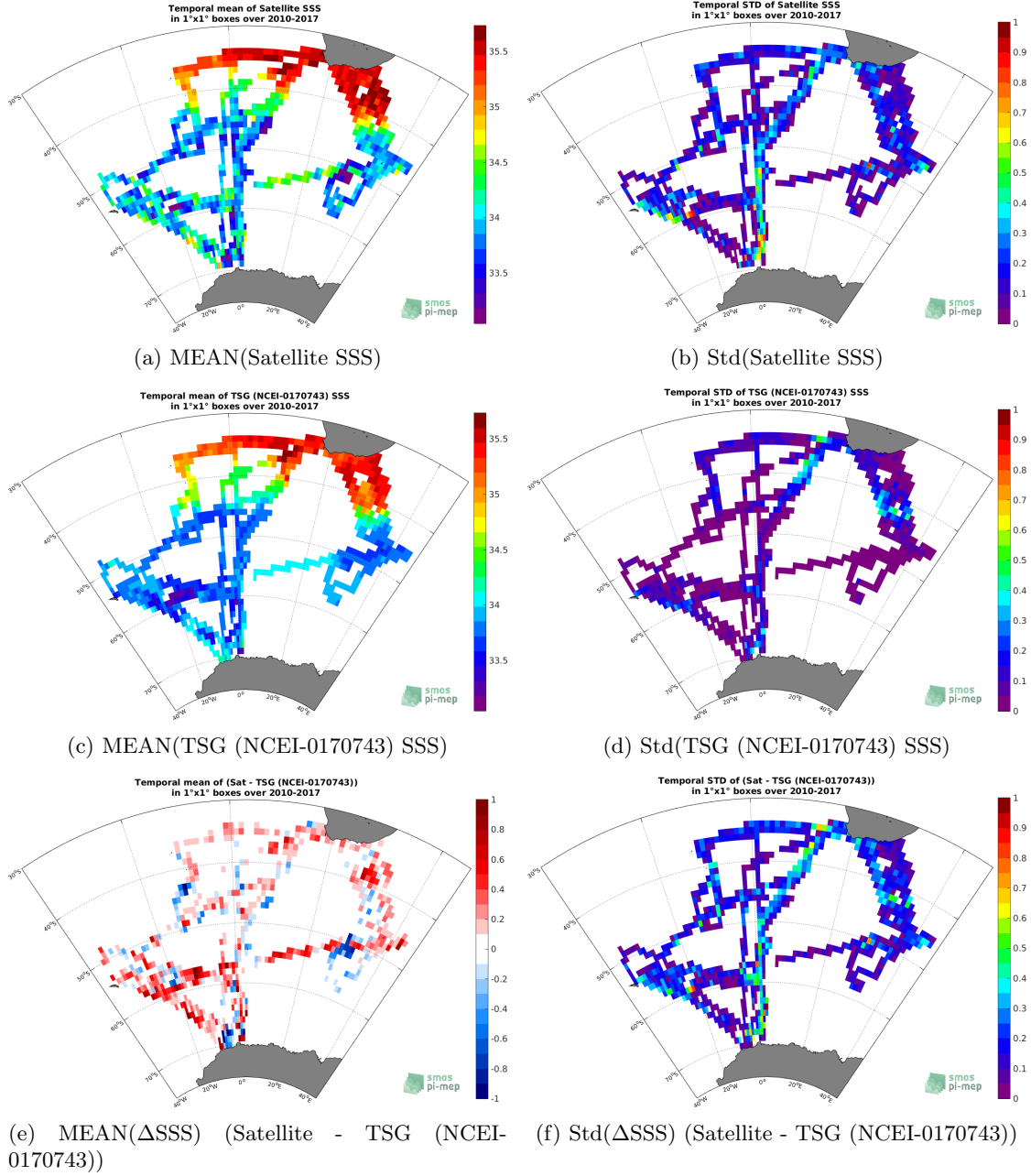
Figure 6: Temporal mean (left) and Std (right) of SSS from SMOS SSS L3 v4 - 9 Days (CATDS-CECOS-LOCEAN) (top), TSG (NCEI-0170743) (middle), and of \Delta SSS (Satellite - TSG (NCEI-0170743)). Only match-up pairs are used to generate these maps.
