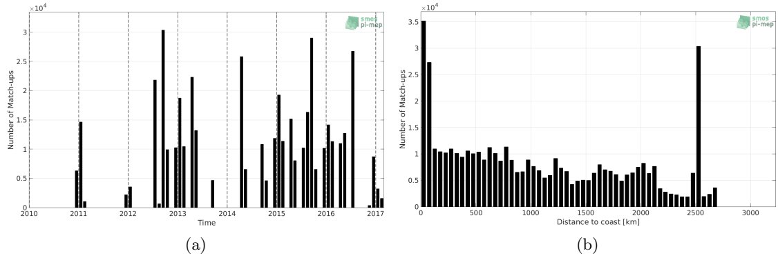
Figure 1: Number of match-ups between TSG (NCEI-0170743) and SMOS SSS L3 v4 - 9 Days (CATDS-CECOS-LOCEAN) SSS as a function of time (a) and as function of the distance to coast (b) over the Global Ocean Pi-MEP region and for the full satellite product period.
