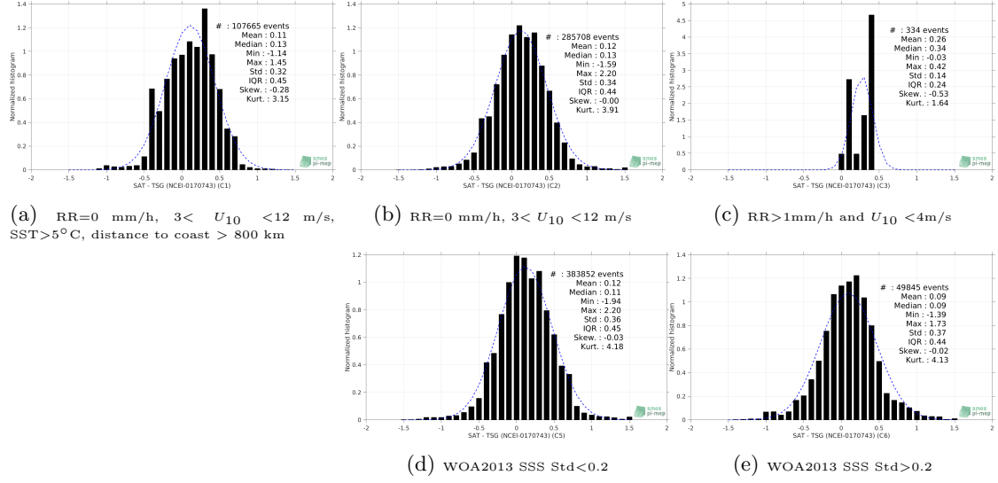
Figure 13: Normalized histogram of \Delta SSS (SMOS SSS L3 v4 - 9 Days (CATDS-CECOS-LOCEAN) - TSG (NCEI-0170743)) for 5 different subdatasets corresponding to: RR=0 mm/h, 3 < U_{10} < 12 m/s, SST>5°C, distance to coast > 800 km (a), RR=0 mm/h, 3 < U_{10} < 12 m/s (b), RR>1mm/h and U_{10} < 4 m/s (c), WOA2013 SSS Std<0.2 (d), WOA2013 SSS Std>0.2 (e).
