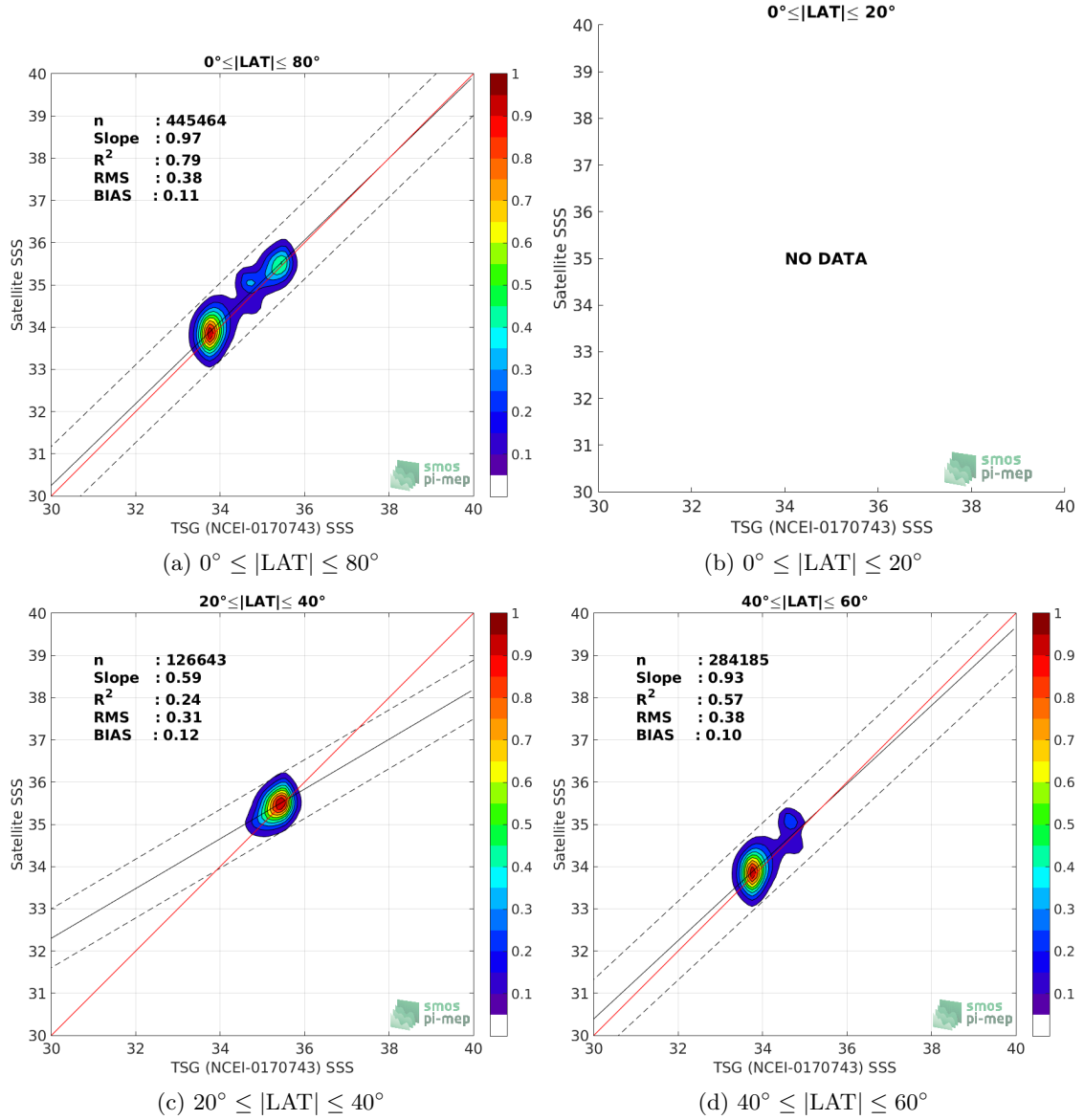
Figure 9: Contour maps of the concentration of SMOS SSS L3 v4 - 9 Days (CATDS-CECOS-LOCEAN) SSS (y-axis) versus TSG (NCEI-0170743) SSS (x-axis) at match-up pairs for different latitude bands. For each plot, the red line shows x=y . The black thin and dashed lines indicate a linear fit through the data cloud and the \pm 95\% confidence levels, respectively. The number match-up pairs n , the slope and R^2 coefficient of the linear fit, the root mean square (RMS) and the mean bias between satellite and in situ data are indicated for each latitude band in each plots.
