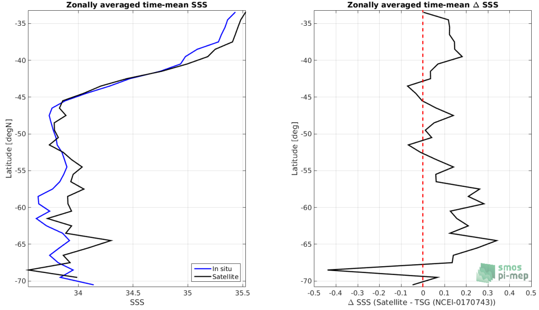
Figure 8: Left panel: Zonal mean SSS from SMOS SSS L3 v4 - 9 Days (CATDS-CECOS-LOCEAN) satellite product (black) and from TSG (NCEI-0170743) (blue). Right panel: Zonal mean of \Delta SSS (Satellite - TSG (NCEI-0170743)) for all the collected Pi-MEP match-up pairs estimated over the full satellite product period.
