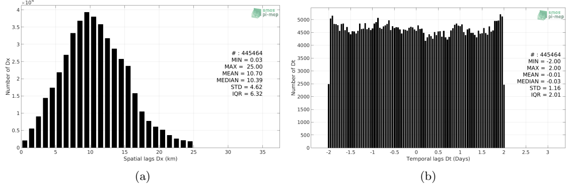
Figure 5: Histograms of the spatial (a) and temporal (b) lags between the time of the TSG (NCEI-0170743) measurements and the date of the corresponding SMOS SSS L3 v4 - 9 Days (CATDS-CECOS-LOCEAN) SSS product.
