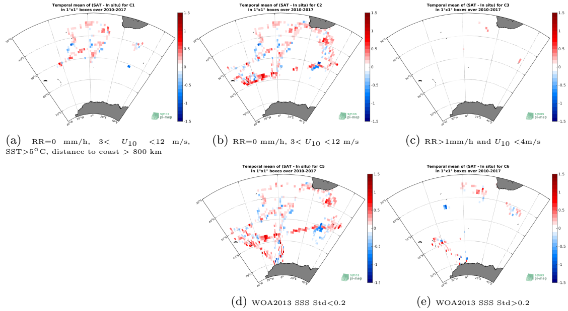
Figure 12: Temporal mean gridded over spatial boxes of size 1^\circ \times 1^\circ of \Delta SSS (SMOS-L3-CATDS-CECOS-LOCEAN-V4-9DAYS-25KM - TSG-NCEI-0170743) for 5 different subdatasets corresponding to:RR=0 mm/h, 3 < U_{10} < 12 m/s, SST >5^\circ C, distance to coast > 800 km (a), RR=0 mm/h, 3 < U_{10} < 12 m/s (b), RR >1 mm/h and U_{10} < 4 m/s (c), WOA2013 SSS Std <0.2 (d), WOA2013 SSS Std >0.2 (e).
