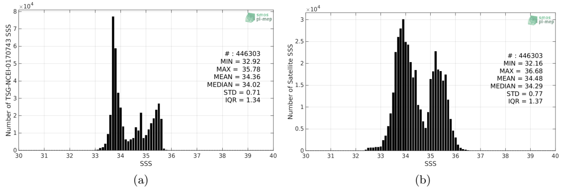
Figure 2: Histograms of SSS from TSG-NCEI-0170743 (a) and SMOS-L3-CATDS-CECOS-LOCEAN-V4-9DAYS-25KM (b) considering all match-up pairs per bins of 0.1 over the Global Ocean Pi-MEP region and for the full satellite product period.
