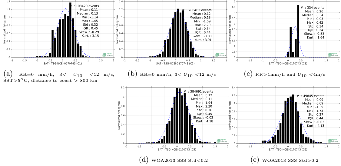
Figure 13: Normalized histogram of \Delta SSS (SMOS-L3-CATDS-CECOS-LOCEAN-V4-9DAYS-25KM - TSG-NCEI-0170743) for 5 different subdatasets corresponding to: RR=0 mm/h, 3 < U_{10} < 12 m/s, SST > 5°C, distance to coast > 800 km (a), RR=0 mm/h, 3 < U_{10} < 12 m/s (b), RR > 1mm/h and U_{10} < 4 m/s (c), WOA2013 SSS Std < 0.2 (d), WOA2013 SSS Std > 0.2 (e).
