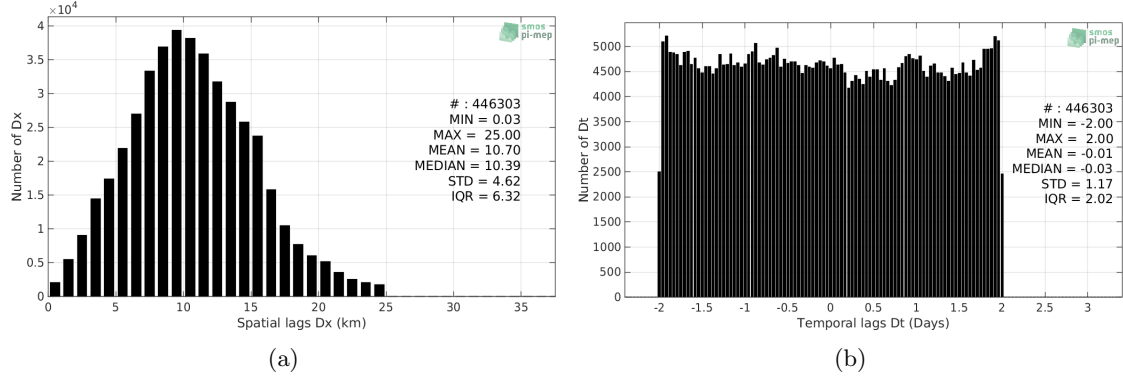
Figure 5: Histograms of the spatial (a) and temporal (b) lags between the time of the TSG-NCEI-0170743 measurements and the date of the corresponding SMOS-L3-CATDS-CECOS-LOCEAN-V4-9DAYS-25KM SSS product.
