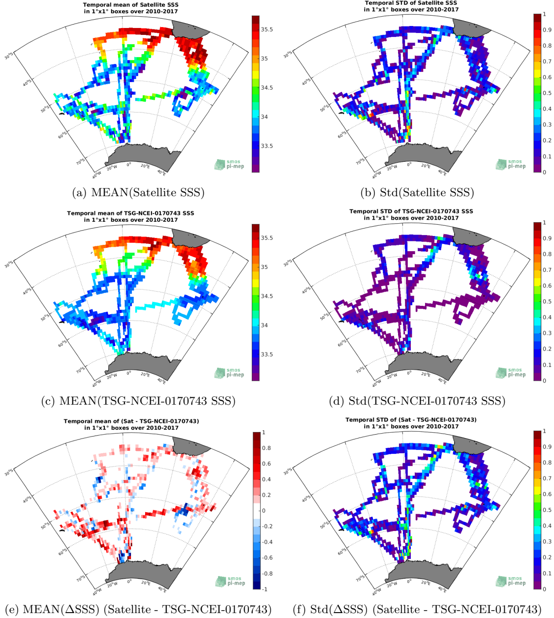
Figure 6: Temporal mean (left) and Std (right) of SSS from SMOS-L3-CATDS-CECOS-LOCEAN-V4-9DAYS-25KM (top), TSG-NCEI-0170743 (middle), and of \Delta SSS (Satellite - TSG-NCEI-0170743). Only match-up pairs are used to generate these maps.
