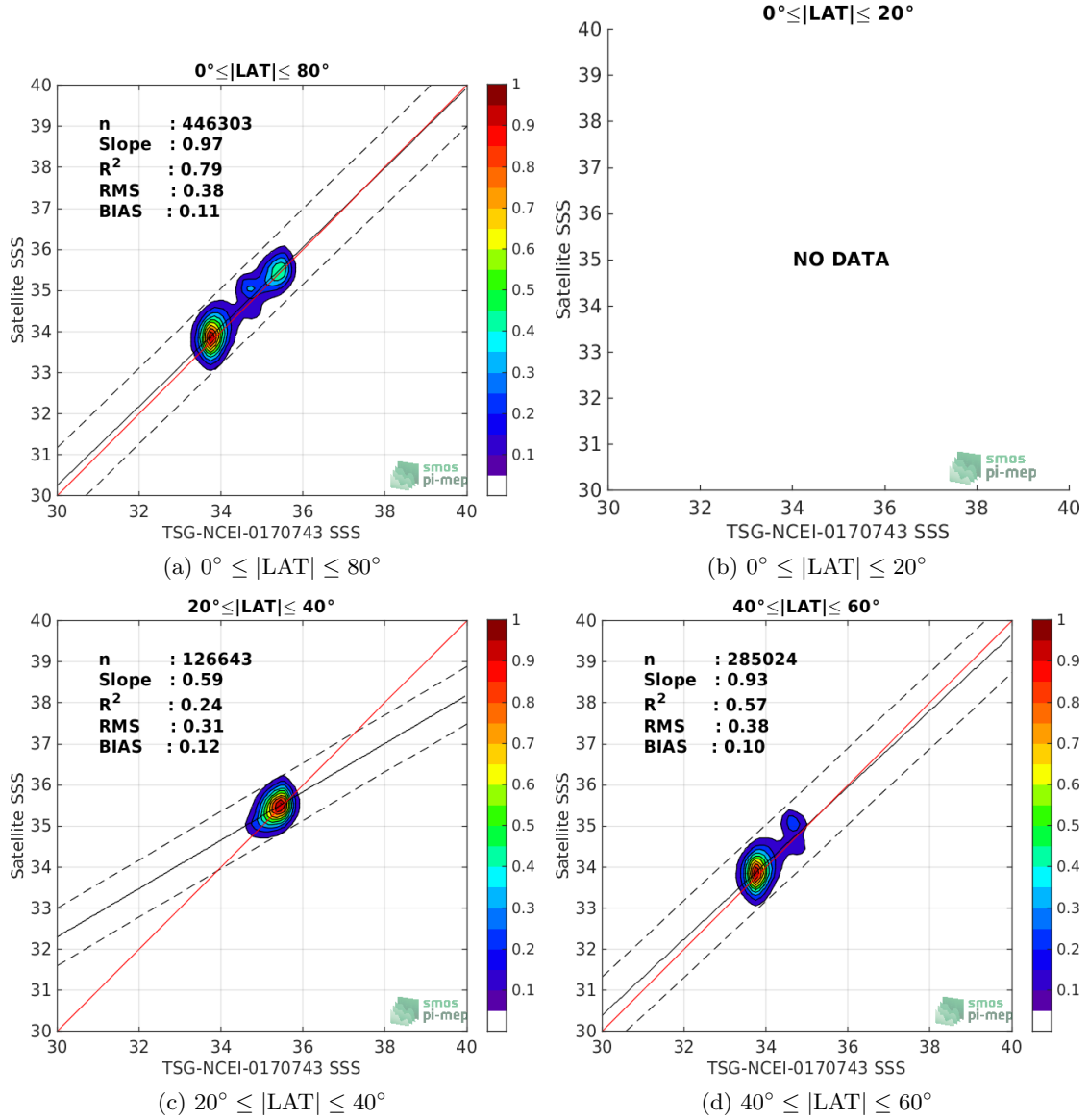
Figure 9: Contour maps of the concentration of SMOS-L3-CATDS-CECOS-LOCEAN-V4-9DAYS-25KM SSS (y-axis) versus TSG-NCEI-0170743 SSS (x-axis) at match-up pairs for different latitude bands. For each plot, the red line shows x=y . The black thin and dashed lines indicate a linear fit through the data cloud and the \pm 95\% confidence levels, respectively. The number match-up pairs n , the slope and R^2 coefficient of the linear fit, the root mean square (RMS) and the mean bias between satellite and in situ data are indicated for each latitude band in each plots.
