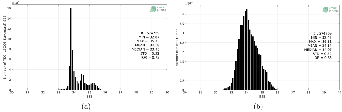
Figure 2: Histograms of SSS from TSG (LEGOS-Survostral) (a) and SMOS SSS L3 v4 - 9 Days (CATDS-CECOS-LOCEAN) (b) considering all match-up pairs per bins of 0.1 over the Global Ocean Pi-MEP region and for the full satellite product period.
