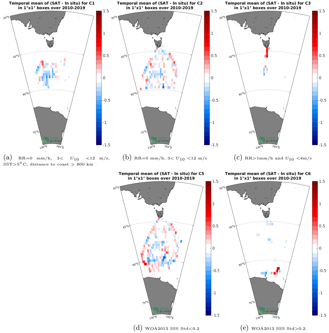
Figure 12: Temporal mean gridded over spatial boxes of size 1°x1° of \Delta\text{SSS} (SMOS SSS L3 v4 - 9 Days (CATDS-CECOS-LOCEAN) - TSG (LEGOS-Survostral)) for 5 different subdatasets corresponding to: RR=0 mm/h, 3 < U_{10} < 12 m/s, SST > 5^\circ\text{C} , distance to coast > 800 km (a), RR=0 mm/h, 3 < U_{10} < 12 m/s (b), RR > 1 mm/h and U_{10} < 4 m/s (c), WOA2013 SSS Std < 0.2 (d), WOA2013 SSS Std > 0.2 (e).
