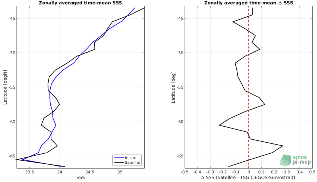
Figure 8: Left panel: Zonal mean SSS from SMOS SSS L3 v4 - 9 Days (CATDS-CECOS-LOCEAN) satellite product (black) and from TSG (LEGOS-Survostral) (blue). Right panel: Zonal mean of \Delta SSS (Satellite - TSG (LEGOS-Survostral)) for all the collected Pi-MEP match-up pairs estimated over the full satellite product period.
