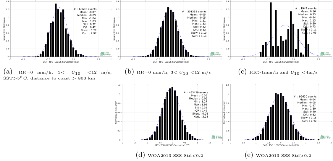
Figure 13: Normalized histogram of \Delta SSS (SMOS SSS L3 v4 - 9 Days (CATDS-CECOS-LOCEAN) - TSG (LEGOS-Survostral)) for 5 different subdatasets corresponding to: RR=0 mm/h, 3 < U_{10} < 12 m/s, SST>5°C, distance to coast > 800 km (a), RR=0 mm/h, 3 < U_{10} < 12 m/s (b), RR>1mm/h and U_{10} < 4 m/s (c), WOA2013 SSS Std<0.2 (d), WOA2013 SSS Std>0.2 (e).
