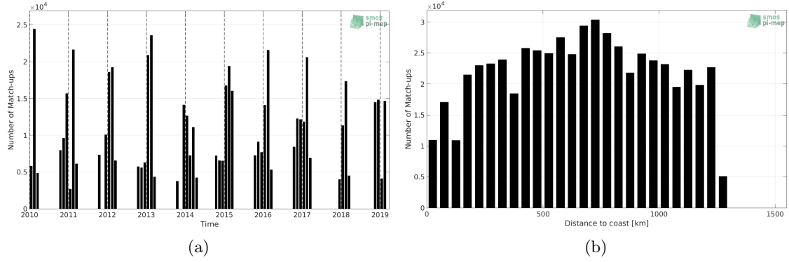
Figure 1: Number of match-ups between TSG (LEGOS-Survostral) and SMOS SSS L3 v4 - 9 Days (CATDS-CECOS-LOCEAN) SSS as a function of time (a) and as function of the distance to coast (b) over the Global Ocean Pi-MEP region and for the full satellite product period.
