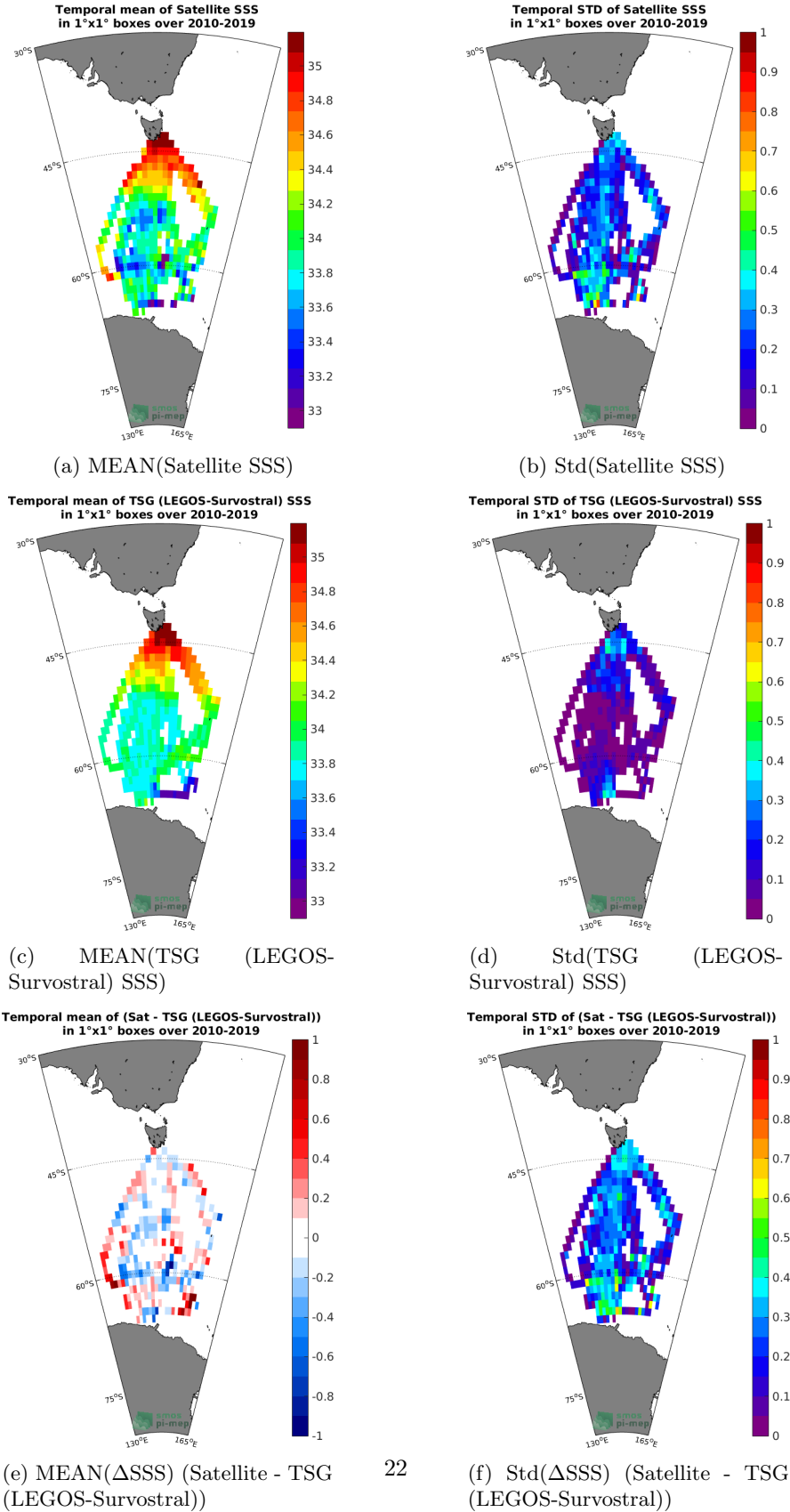
Figure 6: Temporal mean (left) and Std (right) of SSS from SMOS SSS L3 v4 - 9 Days (CATDS-CECOS-LOCEAN) (top), TSG (LEGOS-Survostral) (middle), and of \Delta SSS (Satellite - TSG (LEGOS-Survostral)). Only match-up pairs are used to generate these maps.
