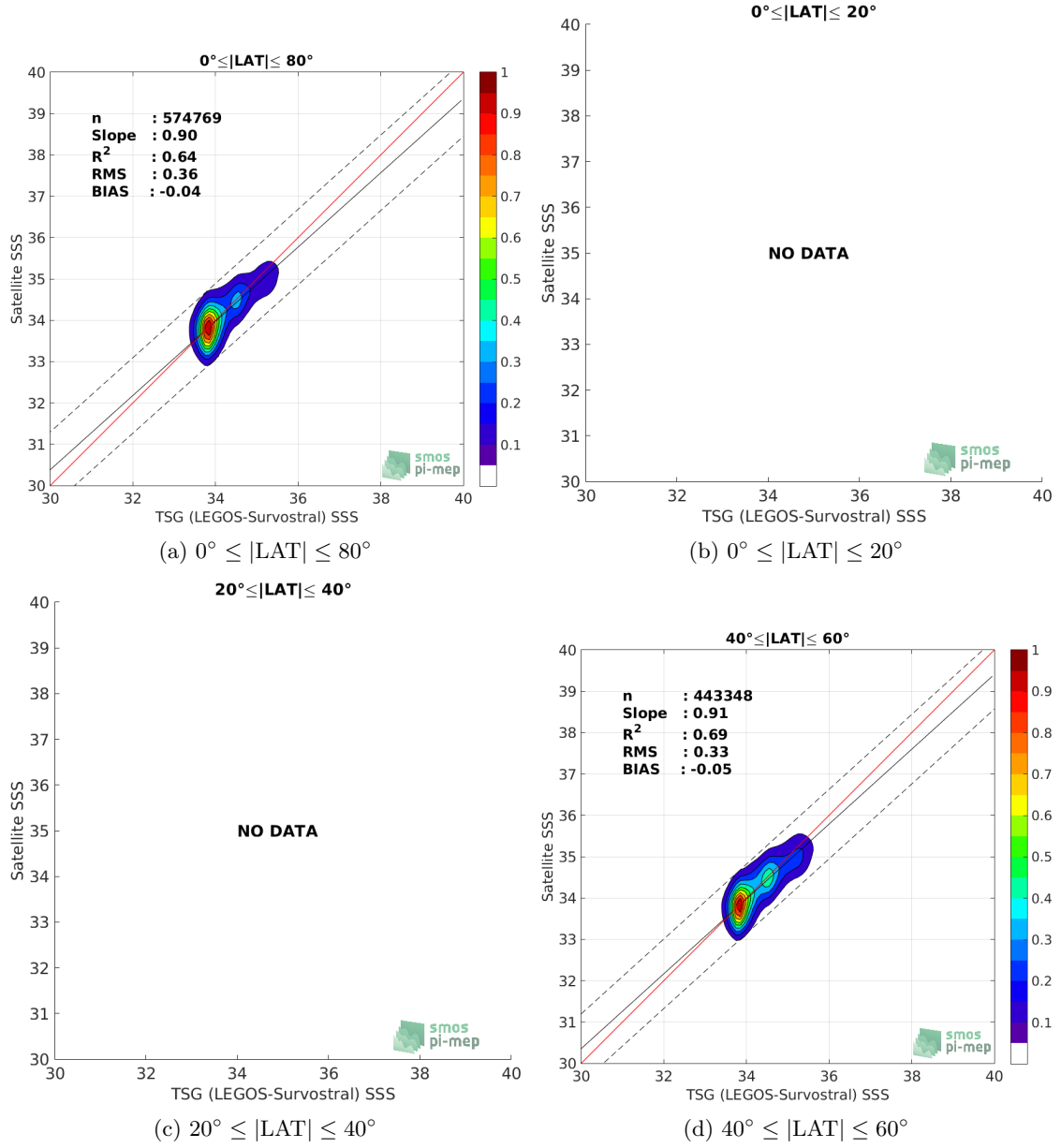
Figure 9: Contour maps of the concentration of SMOS SSS L3 v4 - 9 Days (CATDS-CECOS-LOCEAN) SSS (y-axis) versus TSG (LEGOS-Survostral) SSS (x-axis) at match-up pairs for different latitude bands. For each plot, the red line shows x=y . The black thin and dashed lines indicate a linear fit through the data cloud and the \pm 95\% confidence levels, respectively. The number match-up pairs n , the slope and R^2 coefficient of the linear fit, the root mean square (RMS) and the mean bias between satellite and in situ data are indicated for each latitude band in each plots.
