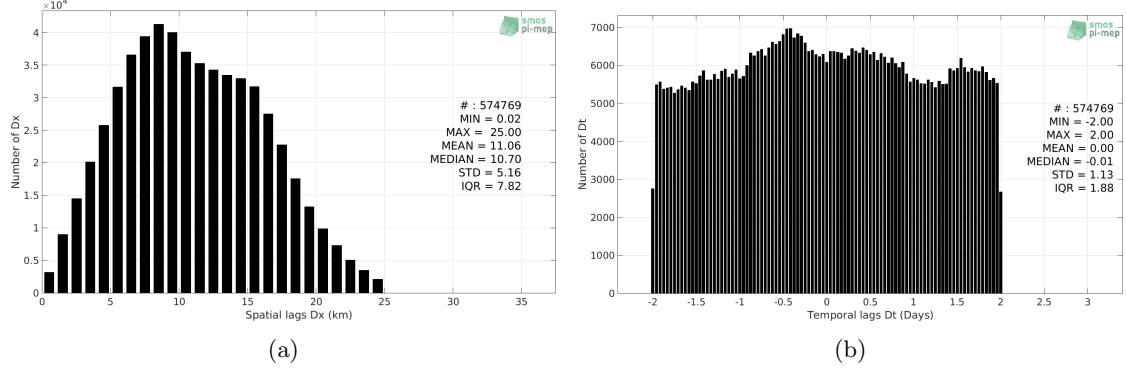
Figure 5: Histograms of the spatial (a) and temporal (b) lags between the time of the TSG (LEGOS-Survostral) measurements and the date of the corresponding SMOS SSS L3 v4 - 9 Days (CATDS-CECOS-LOCEAN) SSS product.
