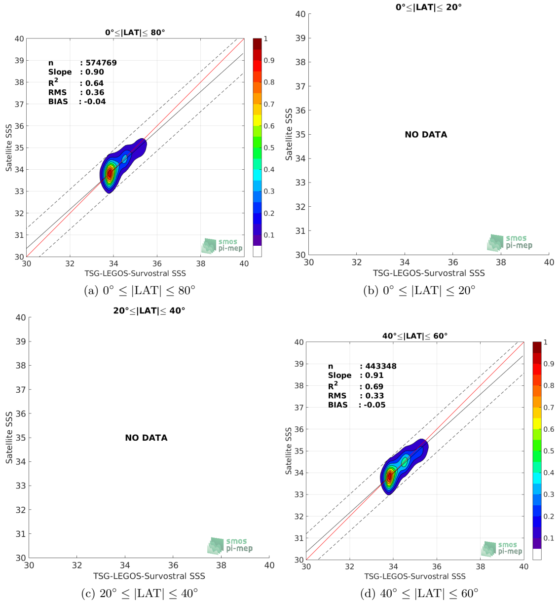
Figure 9: Contour maps of the concentration of SMOS-L3-CATDS-CECOS-LOCEAN-V4-9DAYS-25KM SSS (y-axis) versus TSG-LEGOS-Survostral SSS (x-axis) at match-up pairs for different latitude bands. For each plot, the red line shows x=y . The black thin and dashed lines indicate a linear fit through the data cloud and the \pm 95\% confidence levels, respectively. The number match-up pairs n , the slope and R^2 coefficient of the linear fit, the root mean square (RMS) and the mean bias between satellite and in situ data are indicated for each latitude band in each plots.
