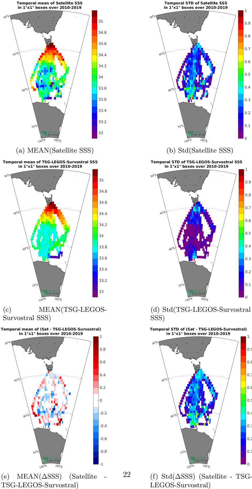
Figure 6: Temporal mean (left) and Std (right) of SSS from SMOS-L3-CATDS-CECOS-LOCEAN-V4-9DAYS-25KM (top), TSG-LEGOS-Survostral (middle), and of \Delta SSS (Satellite - TSG-LEGOS-Survostral). Only match-up pairs are used to generate these maps.
