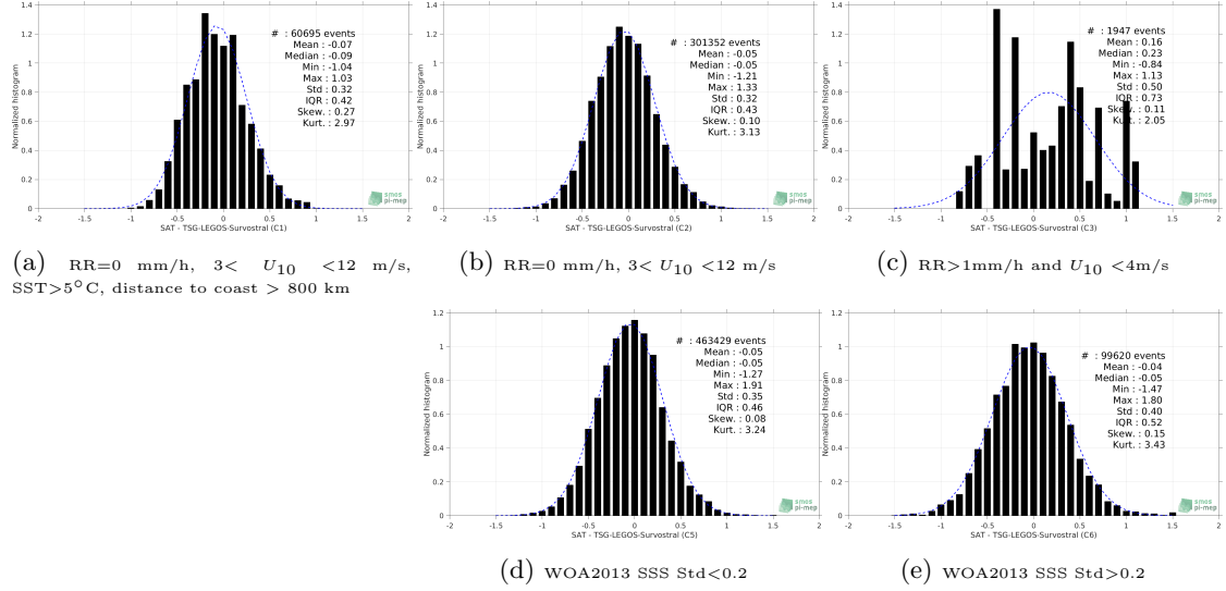
Figure 13: Normalized histogram of \Delta SSS (SMOS-L3-CATDS-CECOS-LOCEAN-V4-9DAYS-25KM - TSG-LEGOS-Survostral) for 5 different subdatasets corresponding to: RR=0 mm/h, 3 < U_{10} < 12 m/s, SST>5°C, distance to coast > 800 km (a), RR=0 mm/h, 3 < U_{10} < 12 m/s (b), RR>1mm/h and U_{10} < 4 m/s (c), WOA2013 SSS Std<0.2 (d), WOA2013 SSS Std>0.2 (e).
