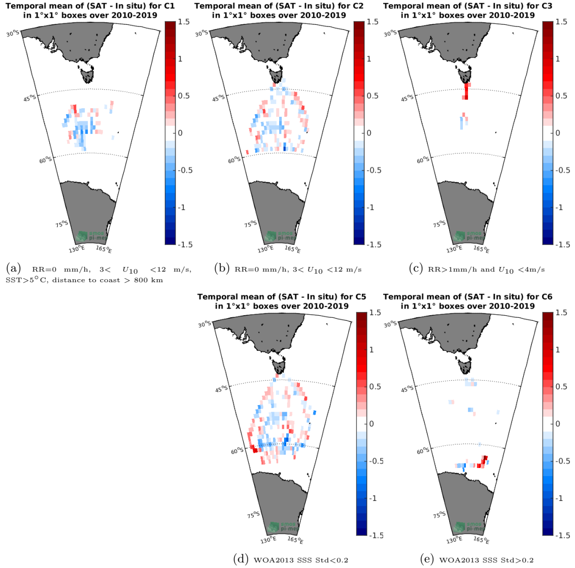
Figure 12: Temporal mean gridded over spatial boxes of size 1°x1° of \Delta\text{SSS} (SMOS-L3-CATDS-CECOS-LOCEAN-V4-9DAYS-25KM - TSG-LEGOS-Survostral) for 5 different subdatasets corresponding to: RR=0 mm/h, 3 < U_{10} < 12 m/s, SST > 5^\circ\text{C} , distance to coast > 800 km (a), RR=0 mm/h, 3 < U_{10} < 12 m/s (b), RR > 1 mm/h and U_{10} < 4 m/s (c), WOA2013 SSS Std < 0.2 (d), WOA2013 SSS Std > 0.2 (e).
