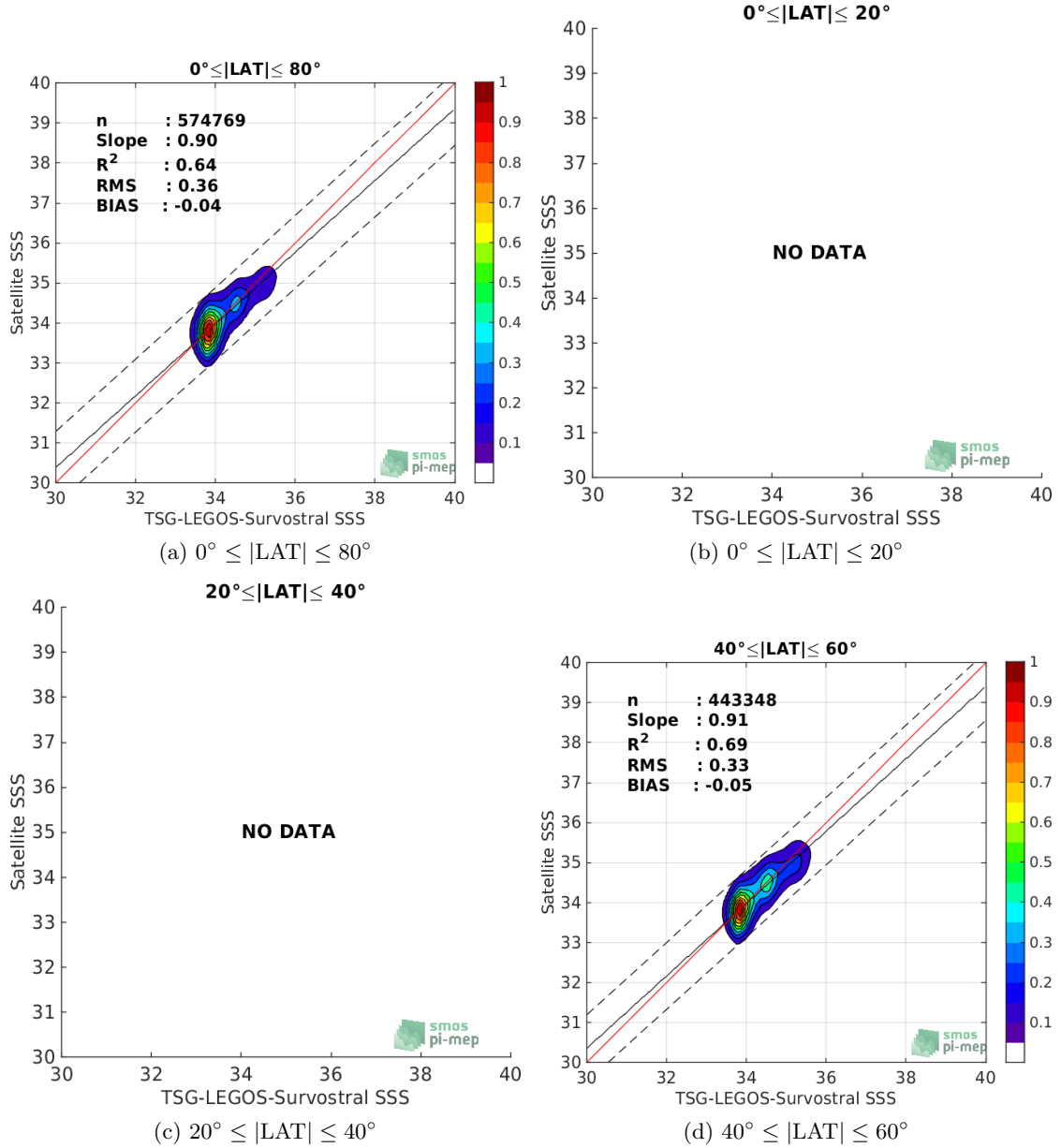
Figure 9: Contour maps of the concentration of SMOS-L3-CATDS-CECOS-LOCEAN-V4-9DAYS-25KM SSS (y-axis) versus TSG-LEGOS-Survostral SSS (x-axis) at match-up pairs for different latitude bands. For each plot, the red line shows x=y . The black thin and dashed lines indicate a linear fit through the data cloud and the \pm 95\% confidence levels, respectively. The number match-up pairs n , the slope and R^2 coefficient of the linear fit, the root mean square (RMS) and the mean bias between satellite and in situ data are indicated for each latitude band in each plots.
