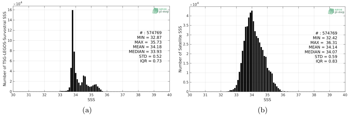
Figure 2: Histograms of SSS from TSG-LEGOS-Survostral (a) and SMOS-L3-CATDS-CECOS-LOCEAN-V4-9DAYS-25KM (b) considering all match-up pairs per bins of 0.1 over the Global Ocean Pi-MEP region and for the full satellite product period.
