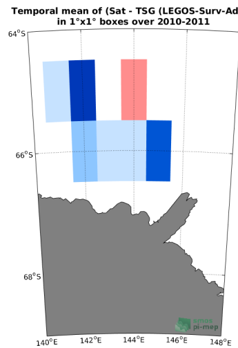
(e) MEAN( \Delta SSS) (Satellite - TSG (LEGOS-Surv-Adel))
