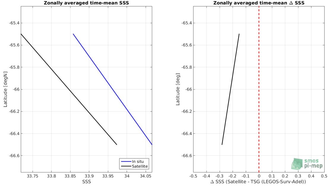
Figure 8: Left panel: Zonal mean SSS from SMOS SSS L3 v4 - 9 Days (CATDS-CECOS-LOCEAN) satellite product (black) and from TSG (LEGOS-Surv-Adel) (blue). Right panel: Zonal mean of \Delta SSS (Satellite - TSG (LEGOS-Surv-Adel)) for all the collected Pi-MEP match-up pairs estimated over the full satellite product period.
