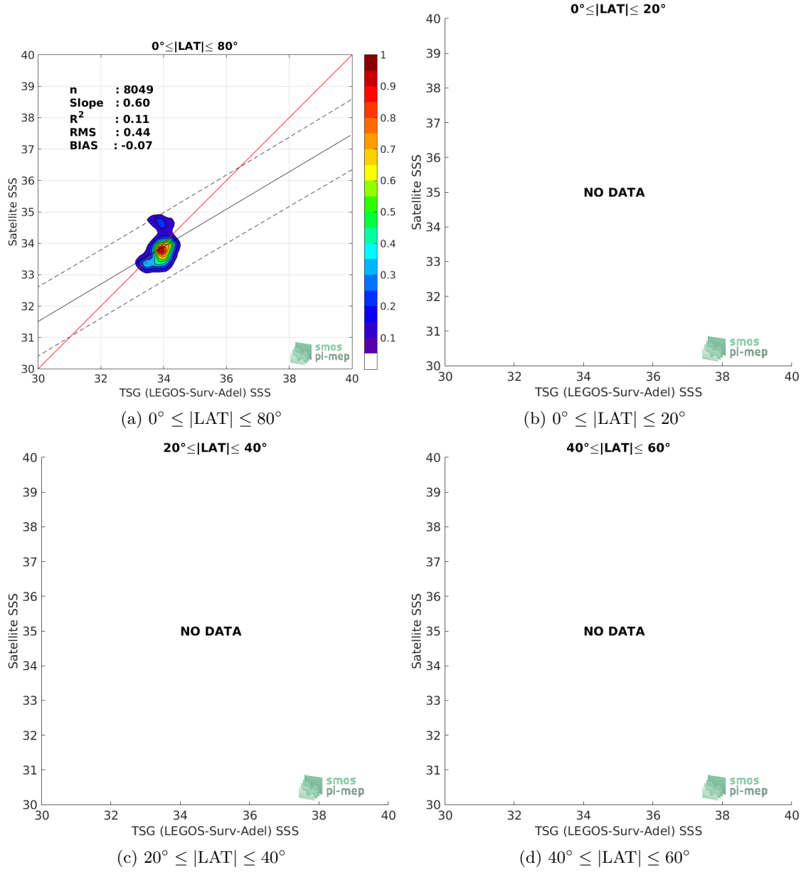
Figure 9: Contour maps of the concentration of SMOS SSS L3 v4 - 9 Days (CATDS-CECOS-LOCEAN) SSS (y-axis) versus TSG (LEGOS-Surv-Adel) SSS (x-axis) at match-up pairs for different latitude bands. For each plot, the red line shows x=y . The black thin and dashed lines indicate a linear fit through the data cloud and the \pm 95\% confidence levels, respectively. The number match-up pairs n , the slope and R^2 coefficient of the linear fit, the root mean square (RMS) and the mean bias between satellite and in situ data are indicated for each latitude band in each plots.
