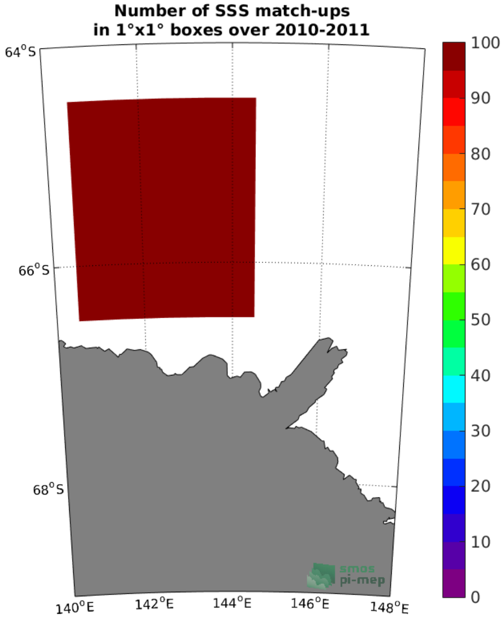
Figure 4: Number of SSS match-ups between TSG (LEGOS-Surv-Adel) SSS and the SMOS SSS L3 v4 - 9 Days (CATDS-CECOS-LOCEAN) SSS product for the Global Ocean Pi-MEP region over 1°x1° boxes and for the full satellite product period.
