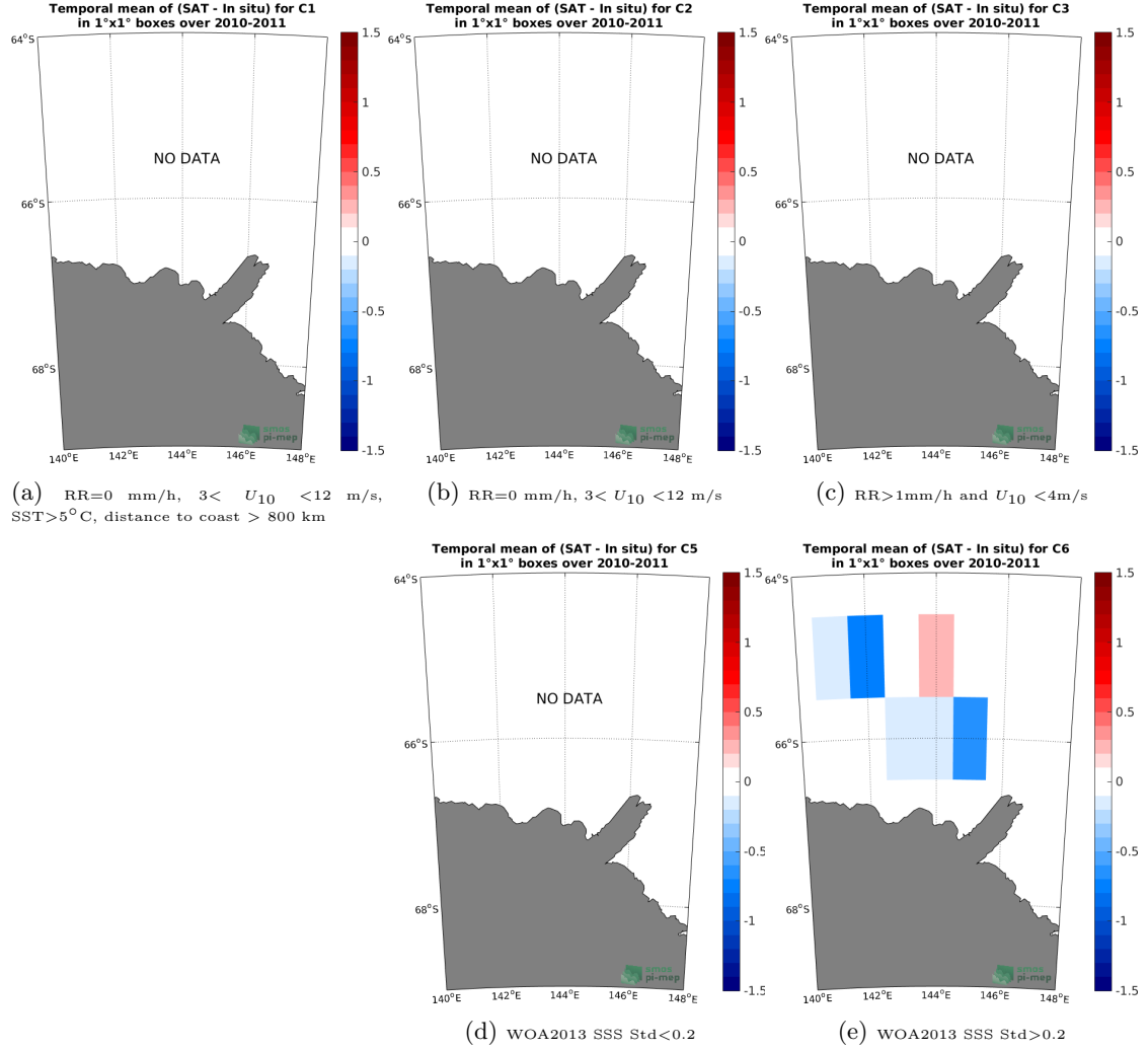
Figure 12: Temporal mean gridded over spatial boxes of size 1°x1° of \Delta\text{SSS} (SMOS SSS L3 v4 - 9 Days (CATDS-CECOS-LOCEAN) - TSG (LEGOS-Surv-Adel)) for 5 different subdatasets corresponding to: RR=0 mm/h, 3 < U_{10} < 12 m/s, SST > 5^\circ\text{C} , distance to coast > 800 km (a), RR=0 mm/h, 3 < U_{10} < 12 m/s (b), RR > 1 mm/h and U_{10} < 4 m/s (c), WOA2013 SSS Std < 0.2 (d), WOA2013 SSS Std > 0.2 (e).
