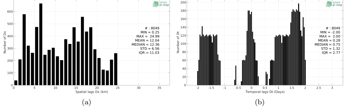
Figure 5: Histograms of the spatial (a) and temporal (b) lags between the time of the TSG (LEGOS-Surv-Adel) measurements and the date of the corresponding SMOS SSS L3 v4 - 9 Days (CATDS-CECOS-LOCEAN) SSS product.
