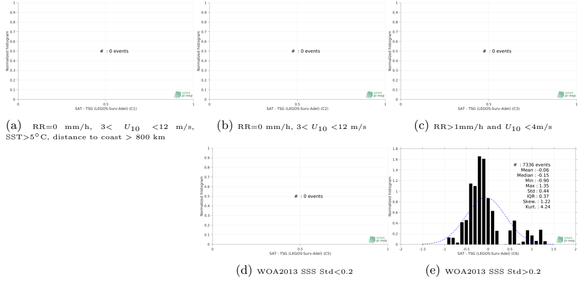
Figure 13: Normalized histogram of \Delta\text{SSS} (SMOS SSS L3 v4 - 9 Days (CATDS-CECOS-LOCEAN) - TSG (LEGOS-Surv-Adel)) for 5 different subdatasets corresponding to: RR=0 mm/h, 3 < U_{10} < 12 m/s, SST > 5^\circ\text{C} , distance to coast > 800 km (a), RR=0 mm/h, 3 < U_{10} < 12 m/s (b), RR > 1 mm/h and U_{10} < 4 m/s (c), WOA2013 SSS Std < 0.2 (d), WOA2013 SSS Std > 0.2 (e).
