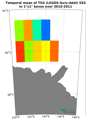
(c) MEAN(TSG (LEGOS-Surv-Adel) SSS)
