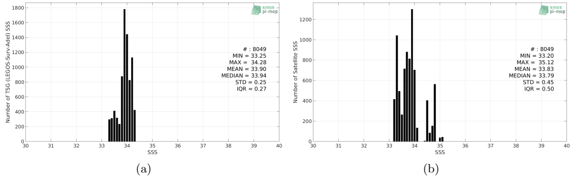
Figure 2: Histograms of SSS from TSG (LEGOS-Surv-Adel) (a) and SMOS SSS L3 v4 - 9 Days (CATDS-CECOS-LOCEAN) (b) considering all match-up pairs per bins of 0.1 over the Global Ocean Pi-MEP region and for the full satellite product period.
