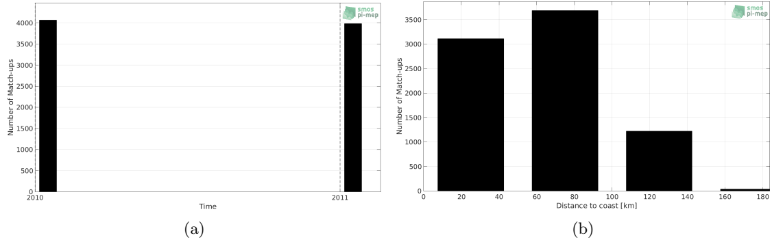
Figure 1: Number of match-ups between TSG (LEGOS-Surv-Adel) and SMOS SSS L3 v4 - 9 Days (CATDS-CECOS-LOCEAN) SSS as a function of time (a) and as function of the distance to coast (b) over the Global Ocean Pi-MEP region and for the full satellite product period.
