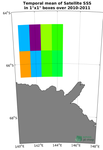
(a) MEAN(Satellite SSS)
