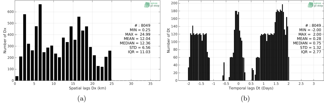
Figure 5: Histograms of the spatial (a) and temporal (b) lags between the time of the TSG-LEGOS-Surv-Adel measurements and the date of the corresponding SMOS-L3-CATDS-CECOS-LOCEAN-V4-9DAYS-25KM SSS product.
