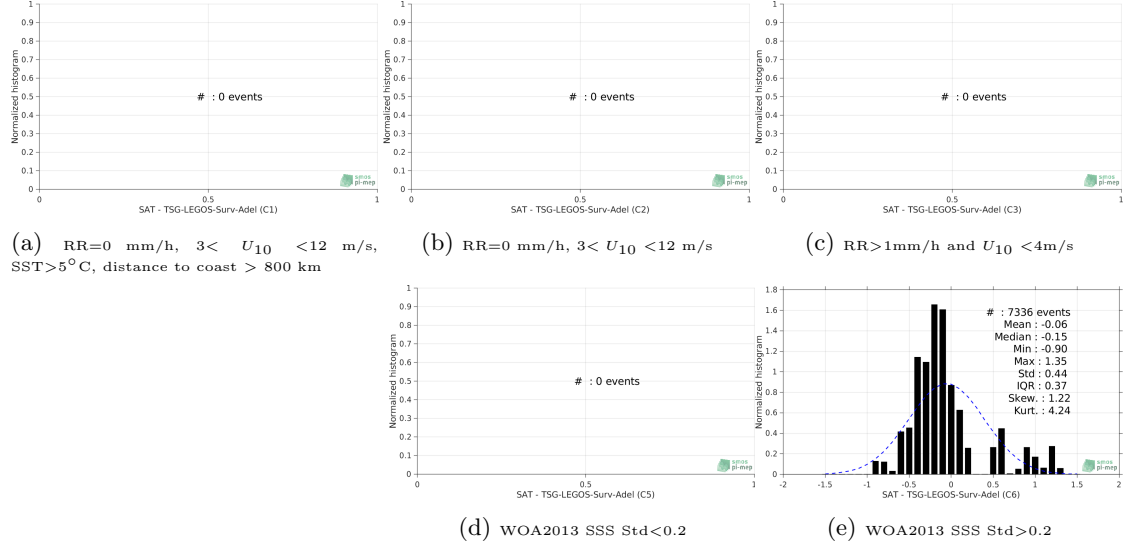
Figure 13: Normalized histogram of \Delta\text{SSS} (SMOS-L3-CATDS-CECOS-LOCEAN-V4-9DAYS-25KM - TSG-LEGOS-Surv-Adel) for 5 different subdatasets corresponding to: RR=0 mm/h, 3 < U_{10} < 12 m/s, SST > 5^\circ\text{C} , distance to coast > 800 km (a), RR=0 mm/h, 3 < U_{10} < 12 m/s (b), RR > 1\text{mm/h} and U_{10} < 4\text{m/s} (c), WOA2013 SSS Std < 0.2 (d), WOA2013 SSS Std > 0.2 (e).
