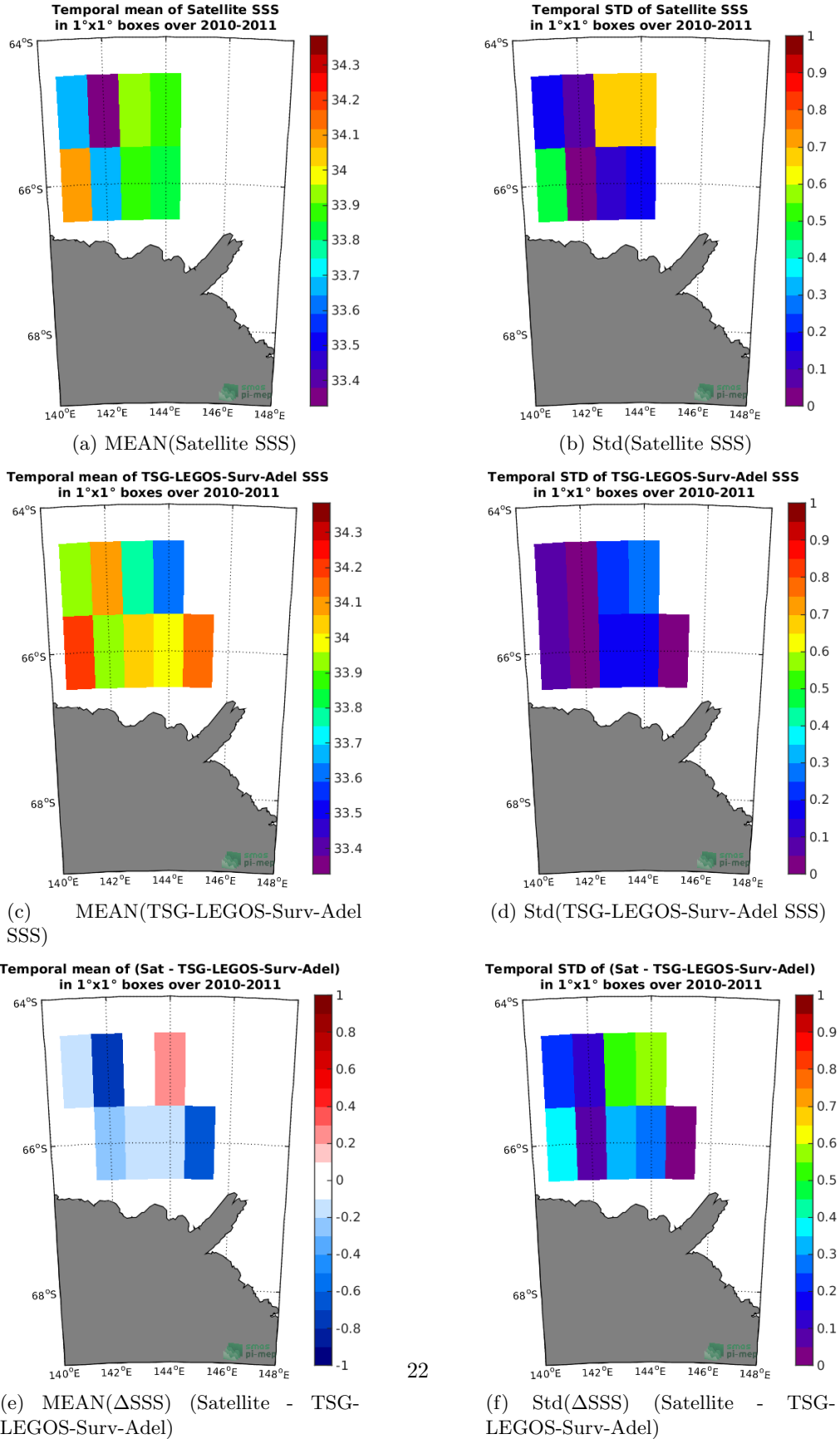
Figure 6: Temporal mean (left) and Std (right) of SSS from SMOS-L3-CATDS-CECOS-LOCEAN-V4-9DAYS-25KM (top), TSG-LEGOS-Surv-Adel (middle), and of \Delta SSS (Satellite - TSG-LEGOS-Surv-Adel). Only match-up pairs are used to generate these maps.
