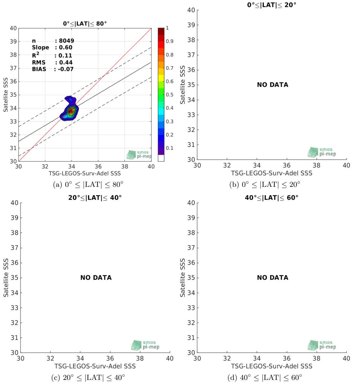
Figure 9: Contour maps of the concentration of SMOS-L3-CATDS-CECOS-LOCEAN-V4-9DAYS-25KM SSS (y-axis) versus TSG-LEGOS-Surv-Adel SSS (x-axis) at match-up pairs for different latitude bands. For each plot, the red line shows x=y . The black thin and dashed lines indicate a linear fit through the data cloud and the \pm 95\% confidence levels, respectively. The number match-up pairs n , the slope and R^2 coefficient of the linear fit, the root mean square (RMS) and the mean bias between satellite and in situ data are indicated for each latitude band in each plots.
