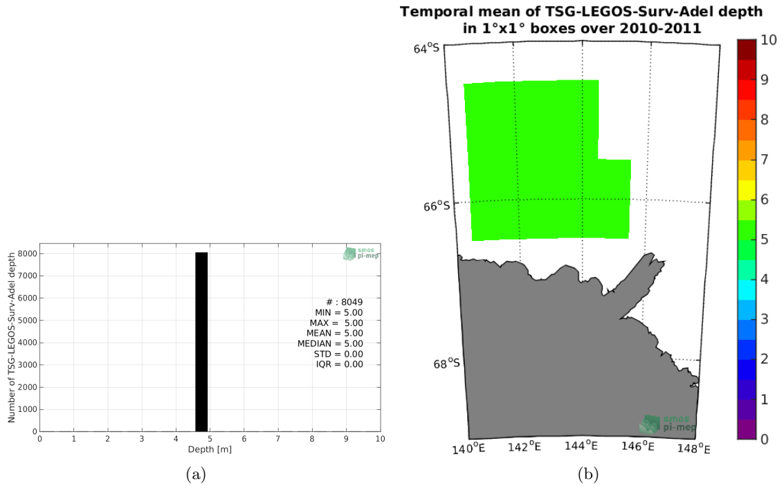
Figure 3: Histograms of the depth of the upper level SSS measurements from TSG-LEGOS-Surv-Adel in the Match-up DataBase for the Global Ocean Pi-MEP region (a) and temporal mean spatial distribution of pressure of the in situ SSS data over 1°x1° boxes and for the full satellite product period (b).
