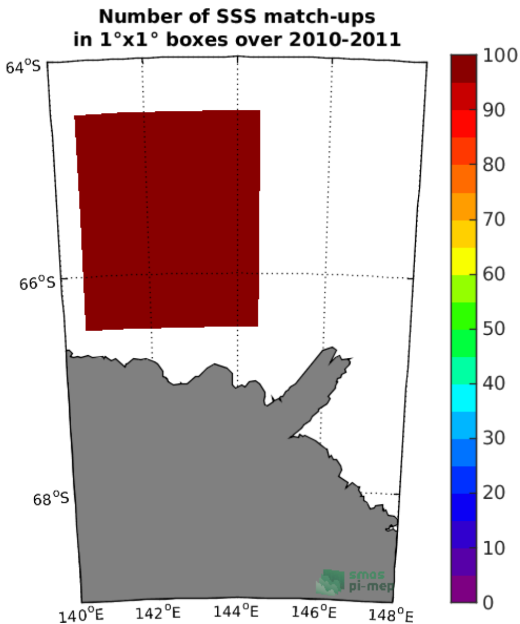
Figure 4: Number of SSS match-ups between TSG-LEGOS-Surv-Adel SSS and the SMOS-L3-CATDS-CECOS-LOCEAN-V4-9DAYS-25KM SSS product for the Global Ocean Pi-MEP region over 1°x1° boxes and for the full satellite product period.
