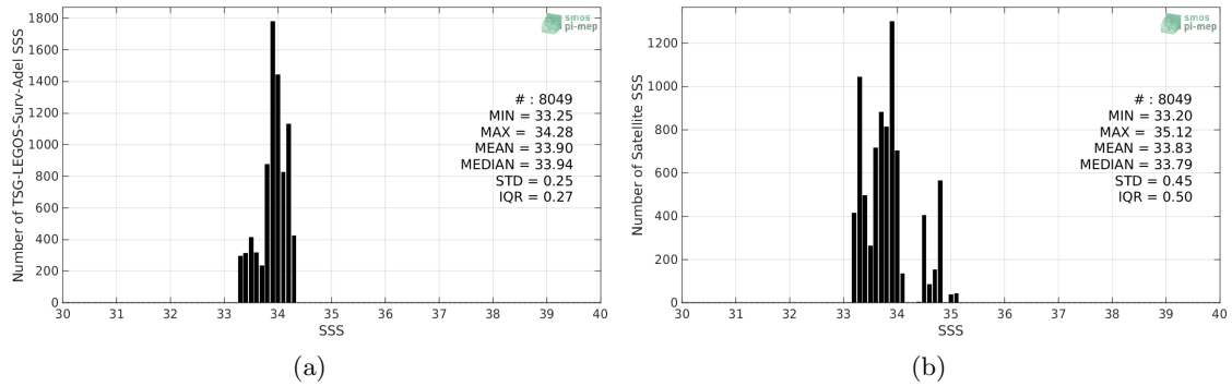
Figure 2: Histograms of SSS from TSG-LEGOS-Surv-Adel (a) and SMOS-L3-CATDS-CECOS-LOCEAN-V4-9DAYS-25KM (b) considering all match-up pairs per bins of 0.1 over the Global Ocean Pi-MEP region and for the full satellite product period.
