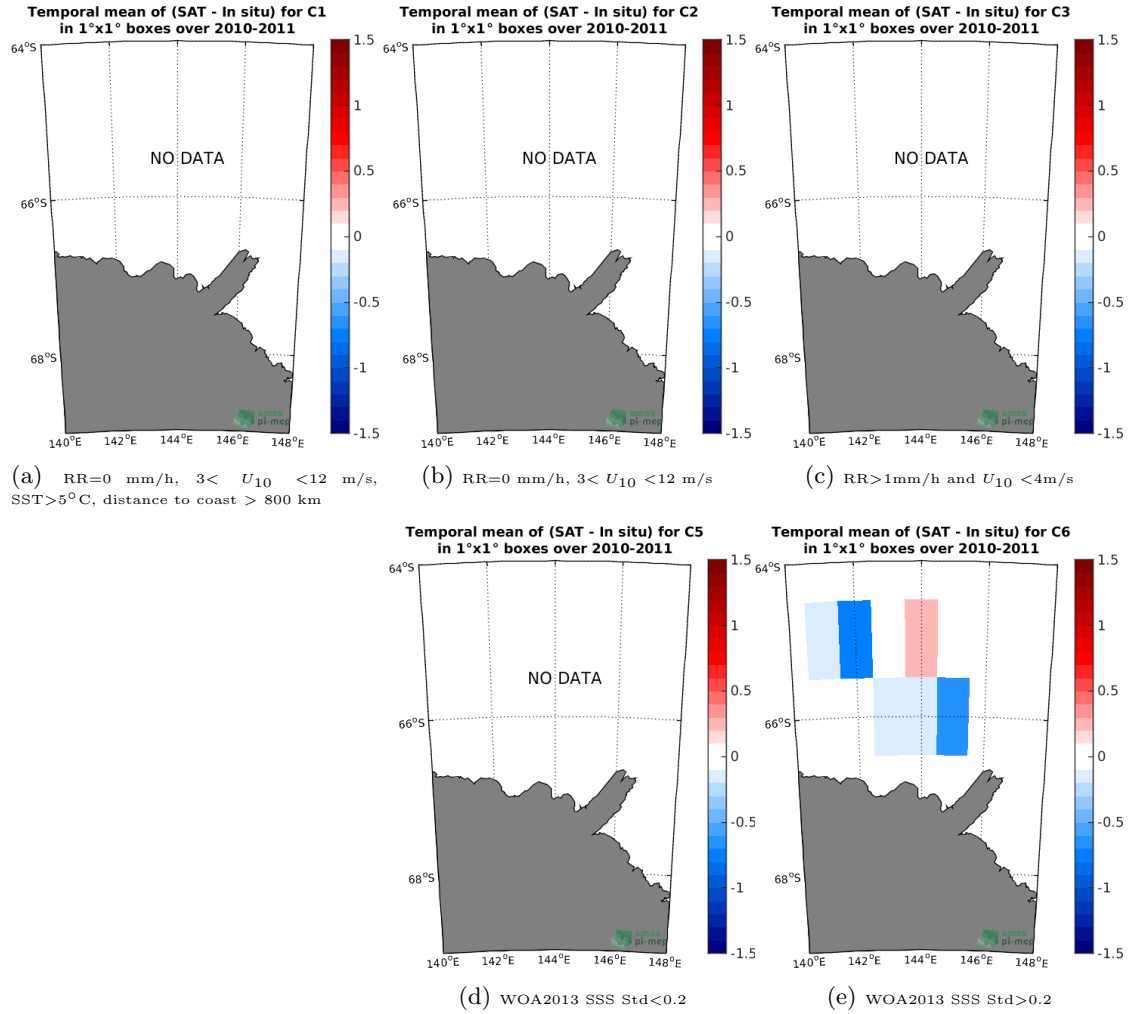
Figure 12: Temporal mean gridded over spatial boxes of size 1^\circ \times 1^\circ of \Delta SSS (SMOS-L3-CATDS-CECOS-LOCEAN-V4-9DAYS-25KM - TSG-LEGOS-Surv-Adel) for 5 different subdatasets corresponding to: RR=0 mm/h, 3 < U_{10} < 12 m/s, SST >5^\circ C, distance to coast > 800 km (a), RR=0 mm/h, 3 < U_{10} < 12 m/s (b), RR >1 mm/h and U_{10} < 4 m/s (c), WOA2013 SSS Std <0.2 (d), WOA2013 SSS Std >0.2 (e).
