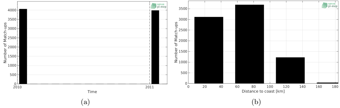
Figure 1: Number of match-ups between TSG-LEGOS-Surv-Adel and SMOS-L3-CATDS-CECOS-LOCEAN-V4-9DAYS-25KM SSS as a function of time (a) and as function of the distance to coast (b) over the Global Ocean Pi-MEP region and for the full satellite product period.
