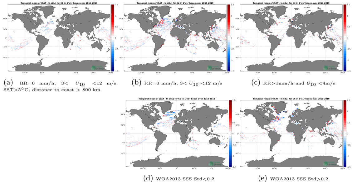
Figure 12: Temporal mean gridded over spatial boxes of size 1^\circ \times 1^\circ of \Delta SSS (SMOS SSS L3 v4 - 9 Days (CATDS-CECOS-LOCEAN) - TSG (LEGOS-DM)) for 5 different subdatasets corresponding to: RR=0 mm/h, 3 < U_{10} < 12 m/s, SST>5°C, distance to coast > 800 km (a), RR=0 mm/h, 3 < U_{10} < 12 m/s (b), RR>1mm/h and U_{10} < 4 m/s (c), WOA2013 SSS Std<0.2 (d), WOA2013 SSS Std>0.2 (e).
