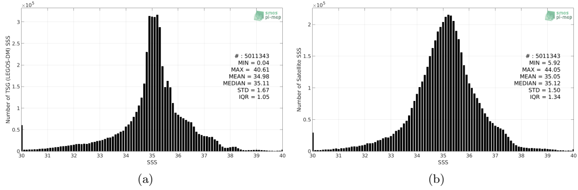
Figure 2: Histograms of SSS from TSG (LEGOS-DM) (a) and SMOS SSS L3 v4 - 9 Days (CATDS-CECOS-LOCEAN) (b) considering all match-up pairs per bins of 0.1 over the Global Ocean Pi-MEP region and for the full satellite product period.
