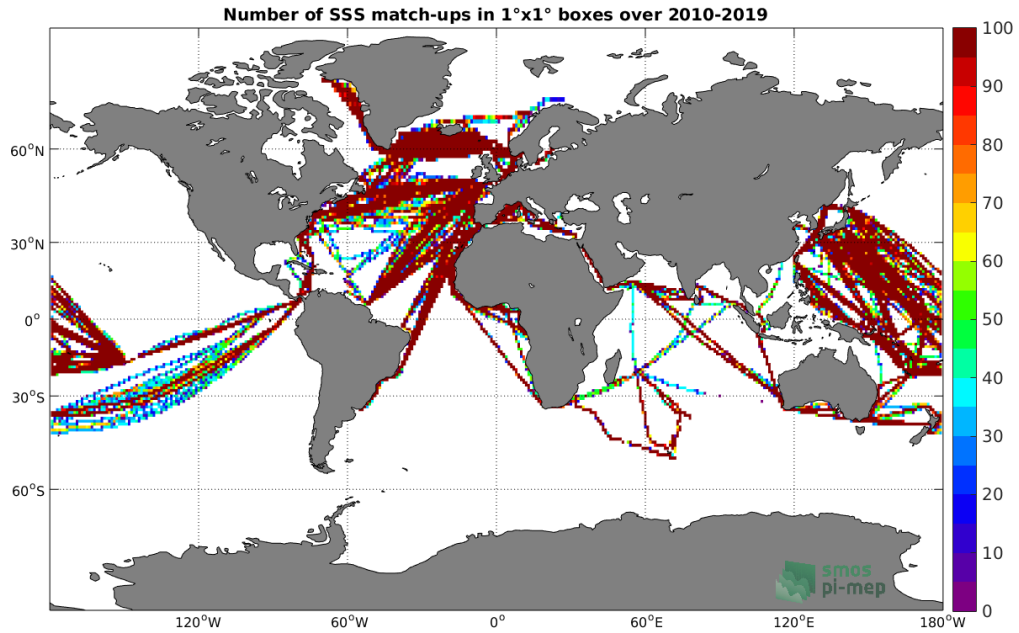
Figure 4: Number of SSS match-ups between TSG (LEGOS-DM) SSS and the SMOS SSS L3 v4 - 9 Days (CATDS-CECOS-LOCEAN) SSS product for the Global Ocean Pi-MEP region over 1^\circ \times 1^\circ boxes and for the full satellite product period.
