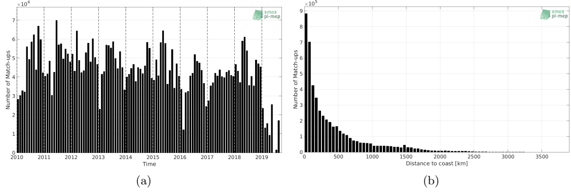
Figure 1: Number of match-ups between TSG (LEGOS-DM) and SMOS SSS L3 v4 - 9 Days (CATDS-CECOS-LOCEAN) SSS as a function of time (a) and as function of the distance to coast (b) over the Global Ocean Pi-MEP region and for the full satellite product period.
