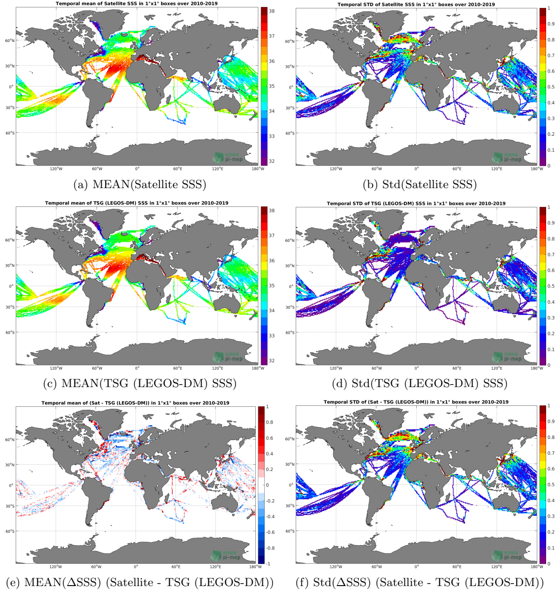
Figure 6: Temporal mean (left) and Std (right) of SSS from SMOS SSS L3 v4 - 9 Days (CATDS-CECOS-LOCEAN) (top), TSG (LEGOS-DM) (middle), and of \Delta SSS (Satellite - TSG (LEGOS-DM)). Only match-up pairs are used to generate these maps.
