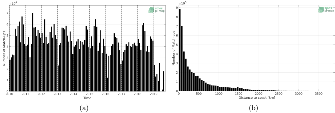
Figure 1: Number of match-ups between TSG-LEGOS-DM and SMOS-L3-CATDS-CECOS-LOCEAN-V4-9DAYS-25KM SSS as a function of time (a) and as function of the distance to coast (b) over the Global Ocean Pi-MEP region and for the full satellite product period.
