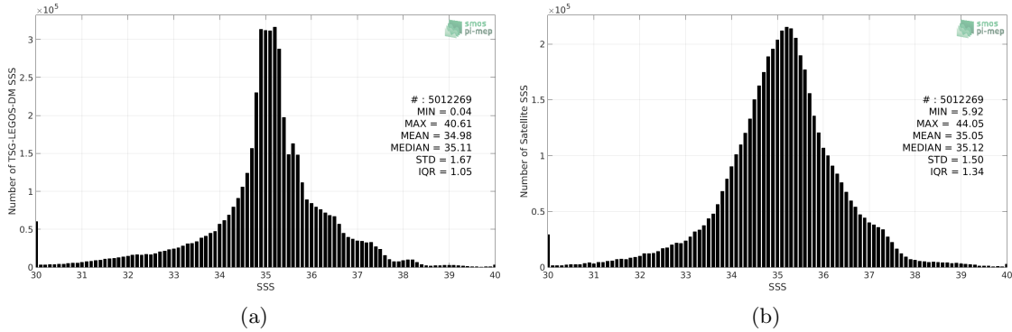
Figure 2: Histograms of SSS from TSG-LEGOS-DM (a) and SMOS-L3-CATDS-CECOS-LOCEAN-V4-9DAYS-25KM (b) considering all match-up pairs per bins of 0.1 over the Global Ocean Pi-MEP region and for the full satellite product period.
