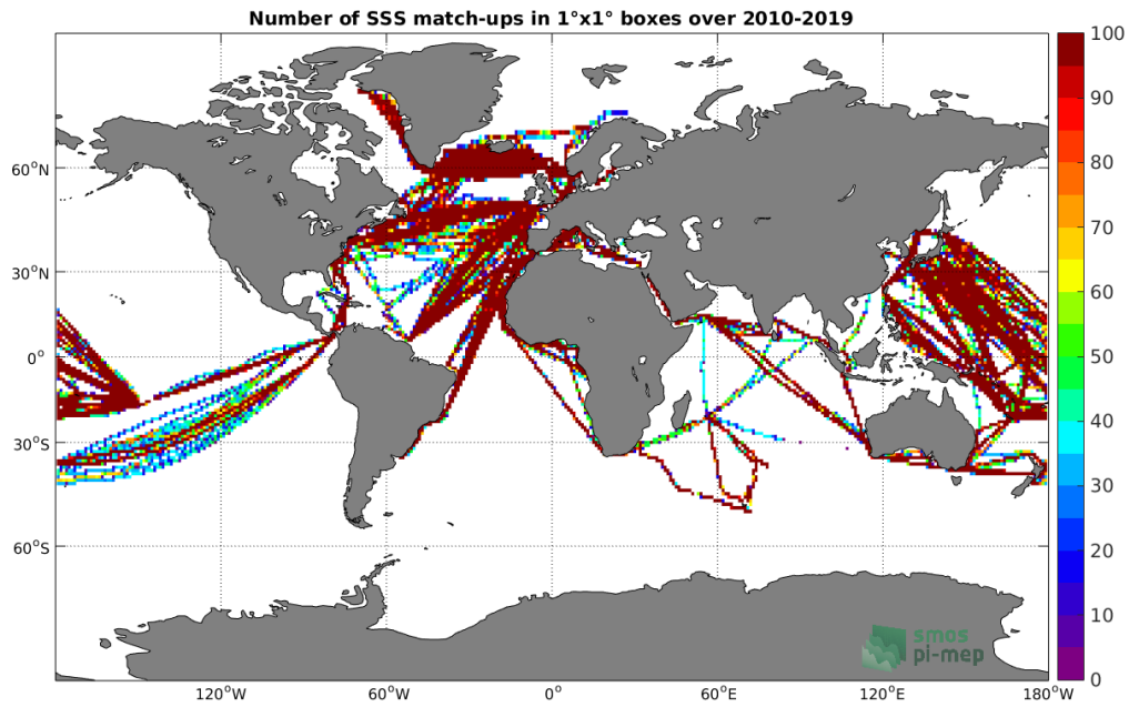
Figure 4: Number of SSS match-ups between TSG-LEGOS-DM SSS and the SMOS-L3-CATDS-CECOS-LOCEAN-V4-9DAYS-25KM SSS product for the Global Ocean Pi-MEP region over 1°x1° boxes and for the full satellite product period.
