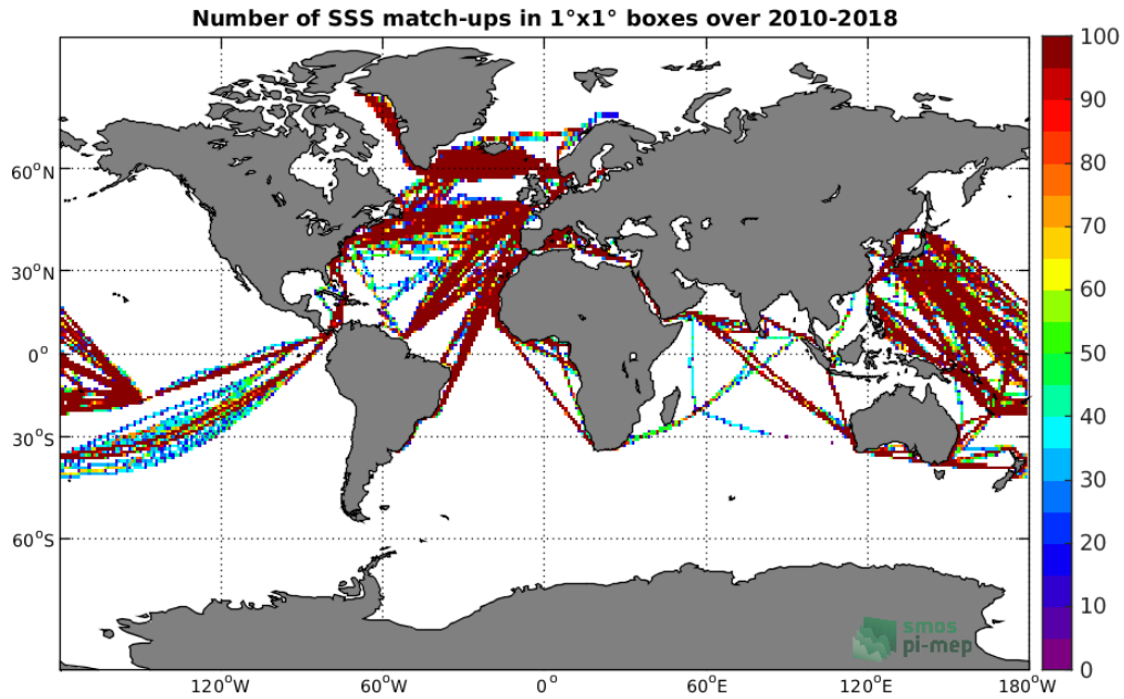
Figure 4: Number of SSS match-ups between TSG-LEGOS-DM SSS and the SMOS-L3-CATDS-CECOS-LOCEAN-V4-9DAYS-25KM SSS product for the Global Ocean Pi-MEP region over 1°x1° boxes and for the full satellite product period.
