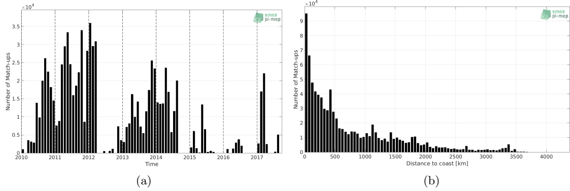
Figure 1: Number of match-ups between TSG (GOSUD-Sailing-ship) and SMOS SSS L3 v4 - 9 Days (CATDS-CECOS-LOCEAN) SSS as a function of time (a) and as function of the distance to coast (b) over the Global Ocean Pi-MEP region and for the full satellite product period.
