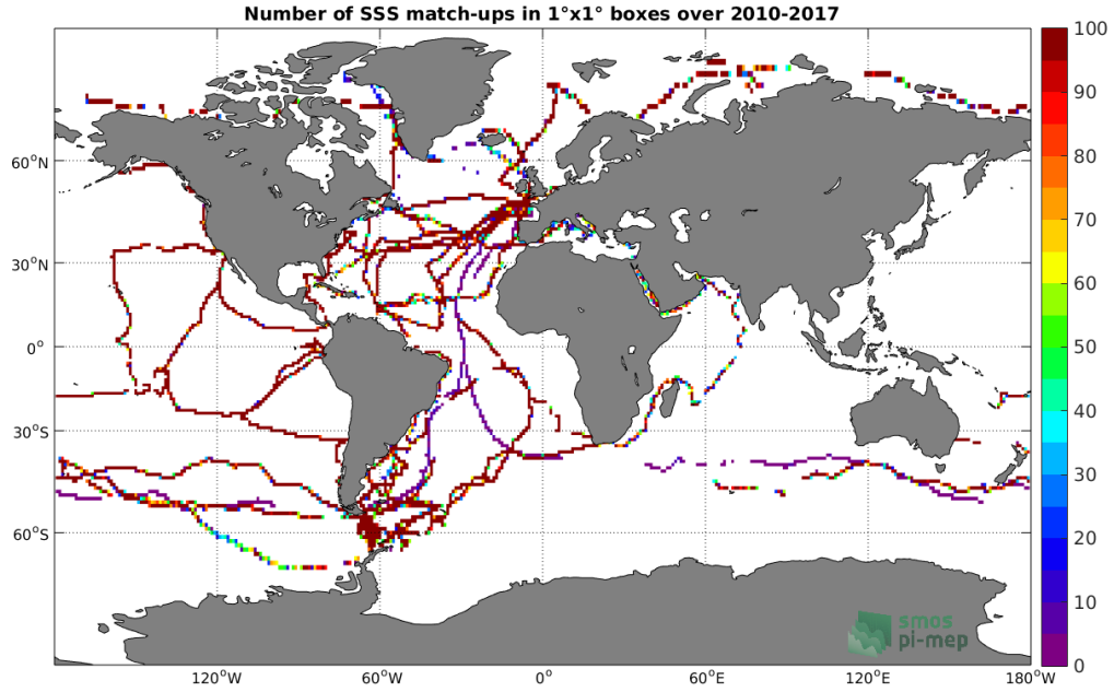
Figure 4: Number of SSS match-ups between TSG (GOSUD-Sailing-ship) SSS and the SMOS SSS L3 v4 - 9 Days (CATDS-CECOS-LOCEAN) SSS product for the Global Ocean Pi-MEP region over 1^\circ \times 1^\circ boxes and for the full satellite product period.
