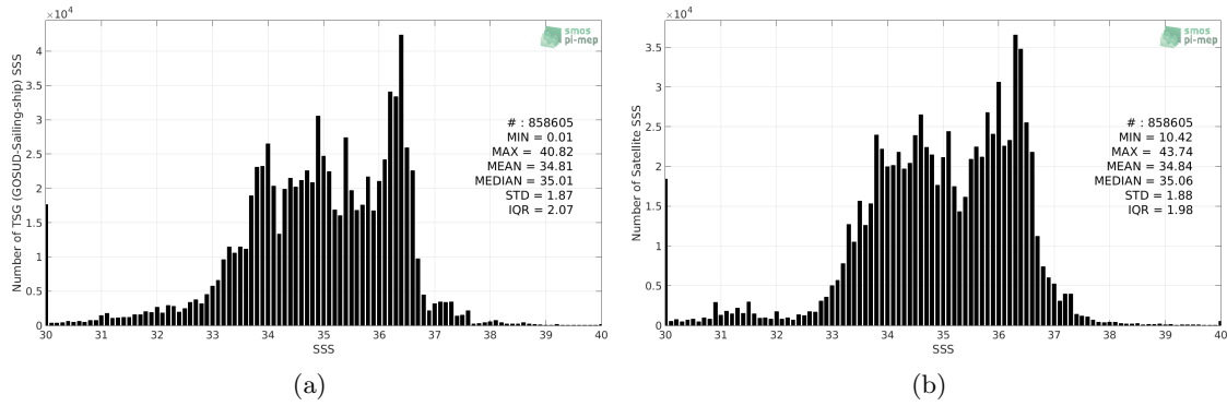
Figure 2: Histograms of SSS from TSG (GOSUD-Sailing-ship) (a) and SMOS SSS L3 v4 - 9 Days (CATDS-CECOS-LOCEAN) (b) considering all match-up pairs per bins of 0.1 over the Global Ocean Pi-MEP region and for the full satellite product period.
