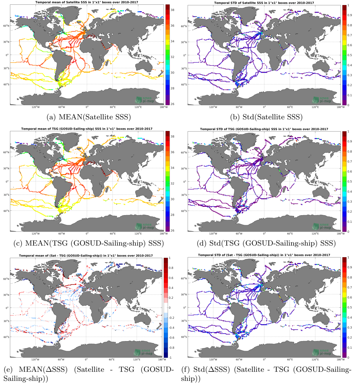
Figure 6: Temporal mean (left) and Std (right) of SSS from SMOS SSS L3 v4 - 9 Days (CATDS-CECOS-LOCEAN) (top), TSG (GOSUD-Sailing-ship) (middle), and of \Delta SSS (Satellite - TSG (GOSUD-Sailing-ship)). Only match-up pairs are used to generate these maps.
