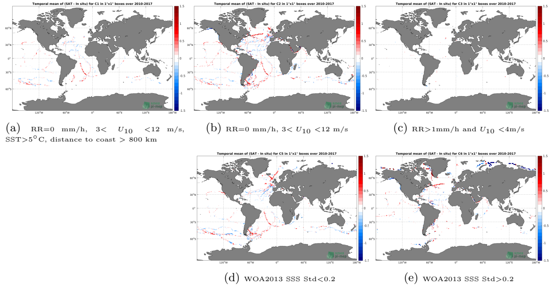
Figure 12: Temporal mean gridded over spatial boxes of size 1^\circ \times 1^\circ of \Delta SSS (SMOS SSS L3 v4 - 9 Days (CATDS-CECOS-LOCEAN) - TSG (GOSUD-Sailing-ship)) for 5 different subdatasets corresponding to: RR=0 mm/h, 3 < U_{10} < 12 m/s, SST >5^\circ\text{C} , distance to coast > 800 km (a), RR=0 mm/h, 3 < U_{10} < 12 m/s (b), RR >1 mm/h and U_{10} < 4 m/s (c), WOA2013 SSS Std <0.2 (d), WOA2013 SSS Std >0.2 (e).
