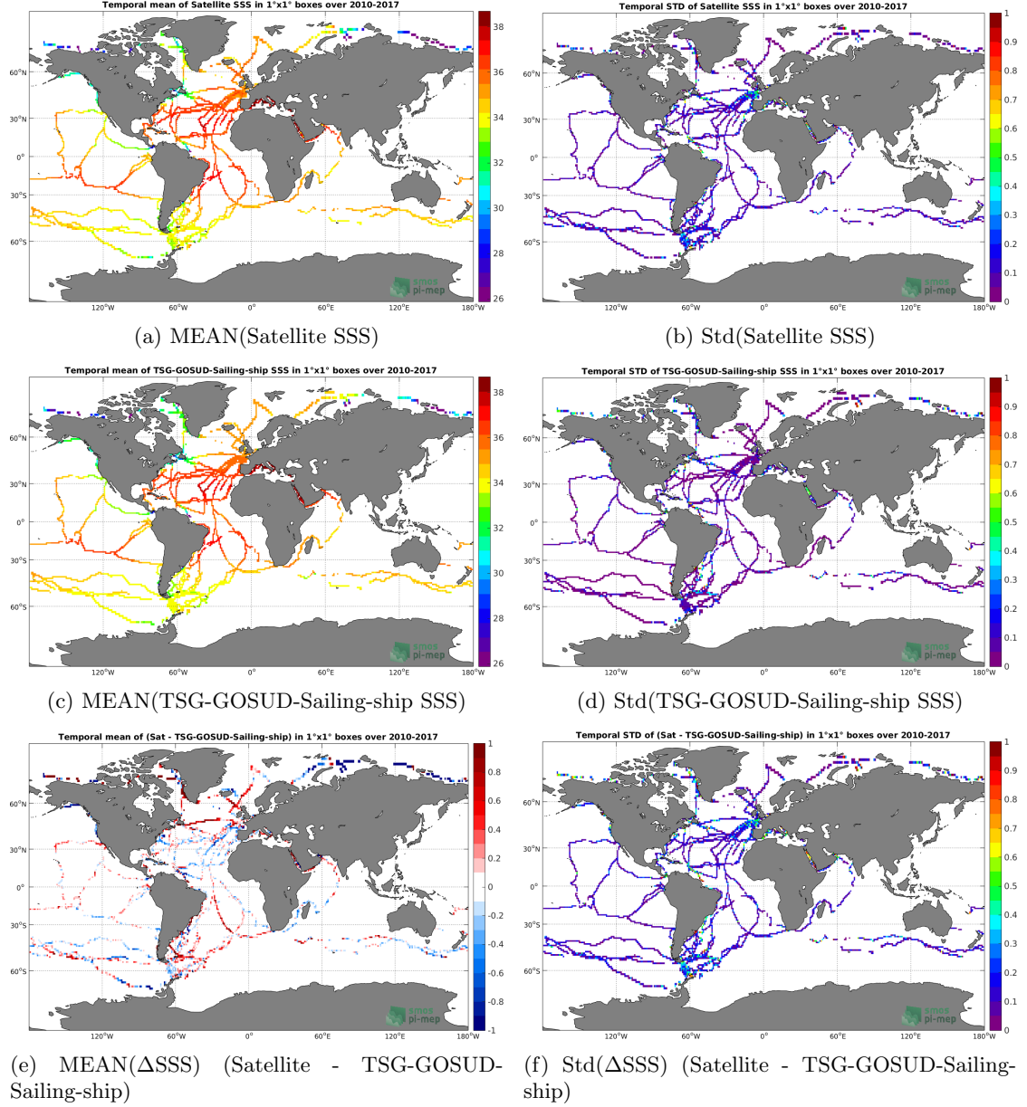
Figure 6: Temporal mean (left) and Std (right) of SSS from SMOS-L3-CATDS-CECOS-LOCEAN-V4-9DAYS-25KM (top), TSG-GOSUD-Sailing-ship (middle), and of \Delta SSS (Satellite - TSG-GOSUD-Sailing-ship). Only match-up pairs are used to generate these maps.
