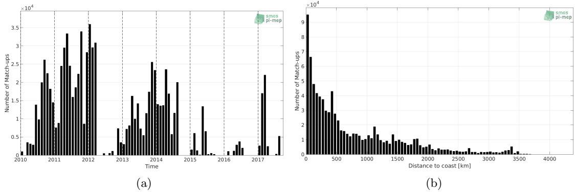
Figure 1: Number of match-ups between TSG-GOSUD-Sailing-ship and SMOS-L3-CATDS-CECOS-LOCEAN-V4-9DAYS-25KM SSS as a function of time (a) and as function of the distance to coast (b) over the Global Ocean Pi-MEP region and for the full satellite product period.
