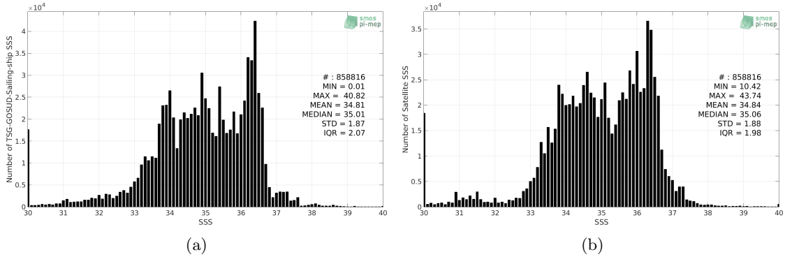
Figure 2: Histograms of SSS from TSG-GOSUD-Sailing-ship (a) and SMOS-L3-CATDS-CECOS-LOCEAN-V4-9DAYS-25KM (b) considering all match-up pairs per bins of 0.1 over the Global Ocean Pi-MEP region and for the full satellite product period.
