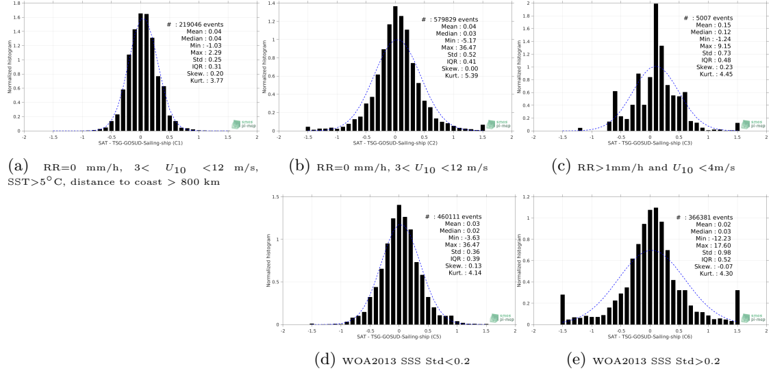
Figure 13: Normalized histogram of \Delta\text{SSS} (SMOS-L3-CATDS-CECOS-LOCEAN-V4-9DAYS-25KM - TSG-GOSUD-Sailing-ship) for 5 different subdatasets corresponding to: RR=0 mm/h, 3 < U_{10} < 12 m/s, SST > 5^\circ\text{C} , distance to coast > 800 km (a), RR=0 mm/h, 3 < U_{10} < 12 m/s (b), RR > 1\text{mm/h} and U_{10} < 4\text{m/s} (c), WOA2013 SSS \text{Std} < 0.2 (d), WOA2013 SSS \text{Std} > 0.2 (e).
