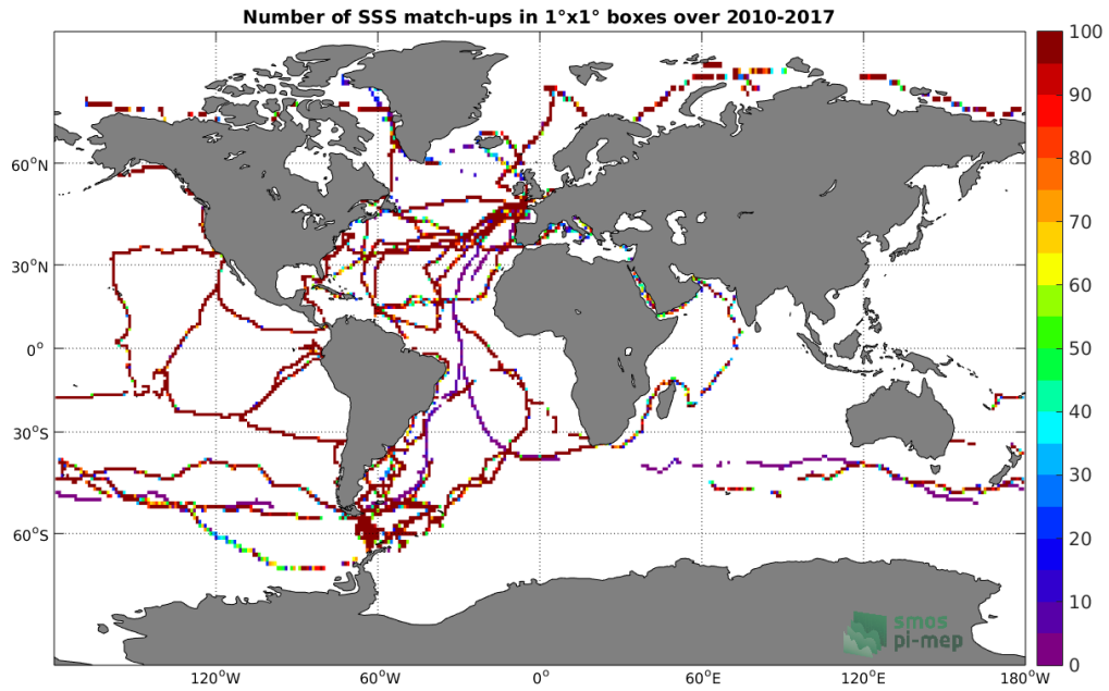
Figure 4: Number of SSS match-ups between TSG-GOSUD-Sailing-ship SSS and the SMOS-L3-CATDS-CECOS-LOCEAN-V4-9DAYS-25KM SSS product for the Global Ocean Pi-MEP region over 1°x1° boxes and for the full satellite product period.
