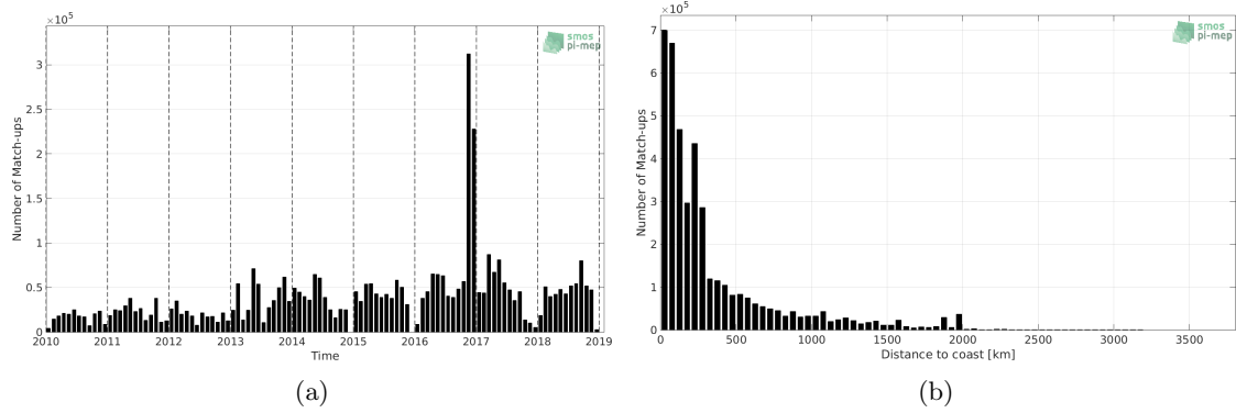
Figure 1: Number of match-ups between TSG (GOSUD-Research-vessel) and SMOS SSS L3 v4 - 9 Days (CATDS-CECOS-LOCEAN) SSS as a function of time (a) and as function of the distance to coast (b) over the Global Ocean Pi-MEP region and for the full satellite product period.
