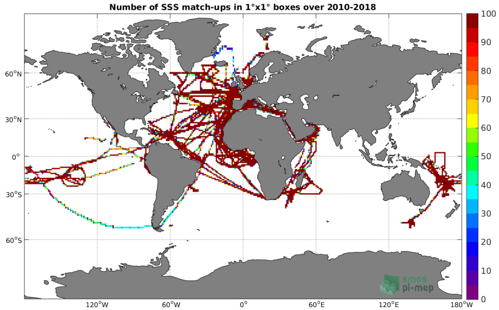
Figure 4: Number of SSS match-ups between TSG (GOSUD-Research-vessel) SSS and the SMOS SSS L3 v4 - 9 Days (CATDS-CECOS-LOCEAN) SSS product for the Global Ocean Pi-MEP region over 1^\circ \times 1^\circ boxes and for the full satellite product period.
