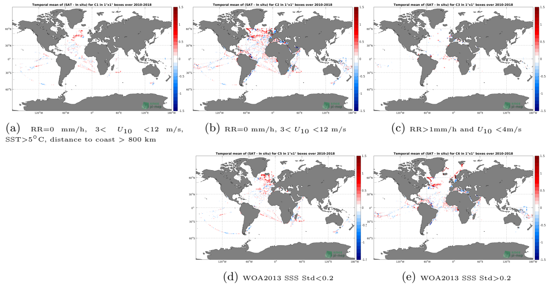
Figure 12: Temporal mean gridded over spatial boxes of size 1^\circ \times 1^\circ of \Delta SSS (SMOS SSS L3 v4 - 9 Days (CATDS-CECOS-LOCEAN) - TSG (GOSUD-Research-vessel)) for 5 different subdatasets corresponding to: RR=0 mm/h, 3 < U_{10} < 12 m/s, SST > 5^\circ C , distance to coast > 800 km (a), RR=0 mm/h, 3 < U_{10} < 12 m/s (b), RR > 1 mm/h and U_{10} < 4 m/s (c), WOA2013 SSS Std < 0.2 (d), WOA2013 SSS Std > 0.2 (e).
