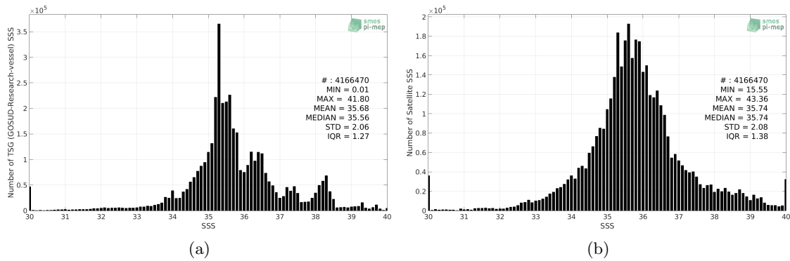
Figure 2: Histograms of SSS from TSG (GOSUD-Research-vessel) (a) and SMOS SSS L3 v4 - 9 Days (CATDS-CECOS-LOCEAN) (b) considering all match-up pairs per bins of 0.1 over the Global Ocean Pi-MEP region and for the full satellite product period.
