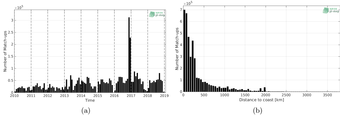
Figure 1: Number of match-ups between TSG-GOSUD-Research-vessel and SMOS-L3-CATDS-CECOS-LOCEAN-V4-9DAYS-25KM SSS as a function of time (a) and as function of the distance to coast (b) over the Global Ocean Pi-MEP region and for the full satellite product period.
