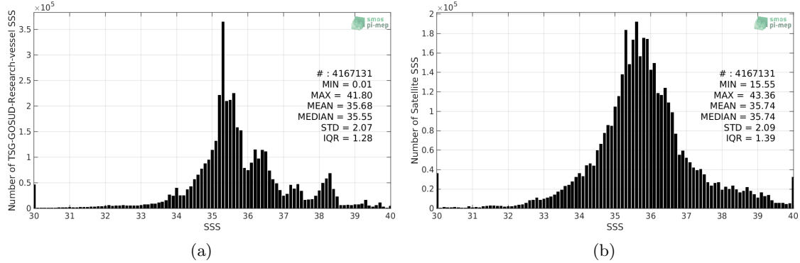
Figure 2: Histograms of SSS from TSG-GOSUD-Research-vessel (a) and SMOS-L3-CATDS-CECOS-LOCEAN-V4-9DAYS-25KM (b) considering all match-up pairs per bins of 0.1 over the Global Ocean Pi-MEP region and for the full satellite product period.
