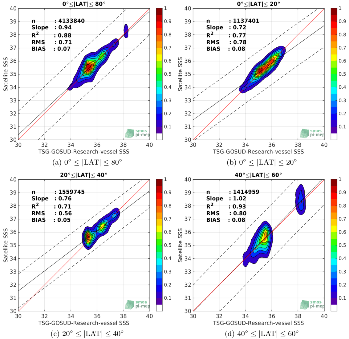
Figure 9: Contour maps of the concentration of SMOS-L3-CATDS-CECOS-LOCEAN-V4-9DAYS-25KM SSS (y-axis) versus TSG-GOSUD-Research-vessel SSS (x-axis) at match-up pairs for different latitude bands. For each plot, the red line shows x=y . The black thin and dashed lines indicate a linear fit through the data cloud and the \pm 95\% confidence levels, respectively. The number match-up pairs n , the slope and R^2 coefficient of the linear fit, the root mean square (RMS) and the mean bias between satellite and in situ data are indicated for each latitude band in each plots.
