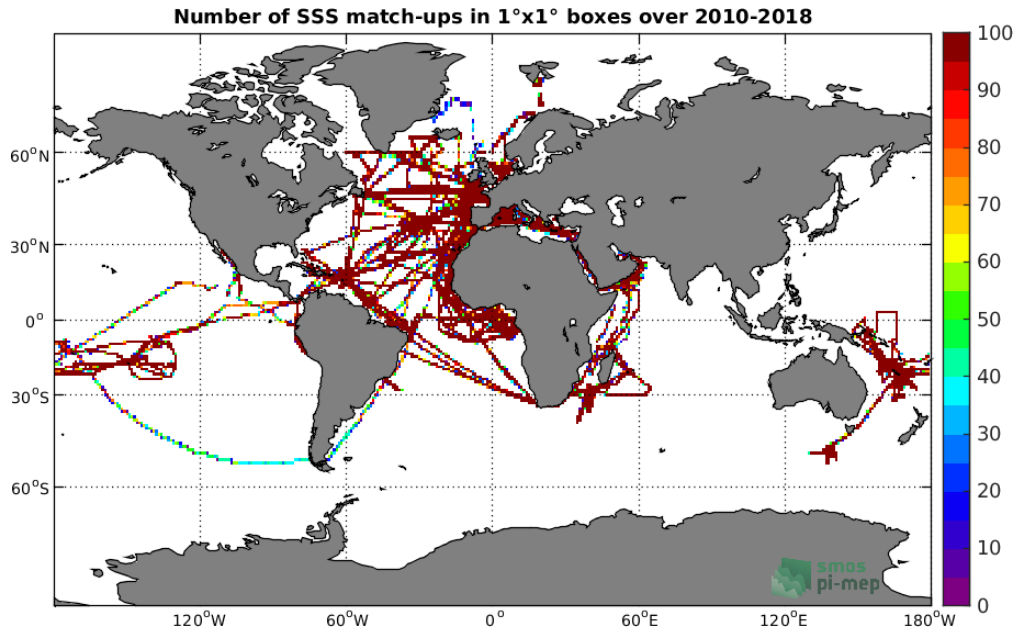
Figure 4: Number of SSS match-ups between TSG-GOSUD-Research-vessel SSS and the SMOS-L3-CATDS-CECOS-LOCEAN-V4-9DAYS-25KM SSS product for the Global Ocean Pi-MEP region over 1^\circ \times 1^\circ boxes and for the full satellite product period.
