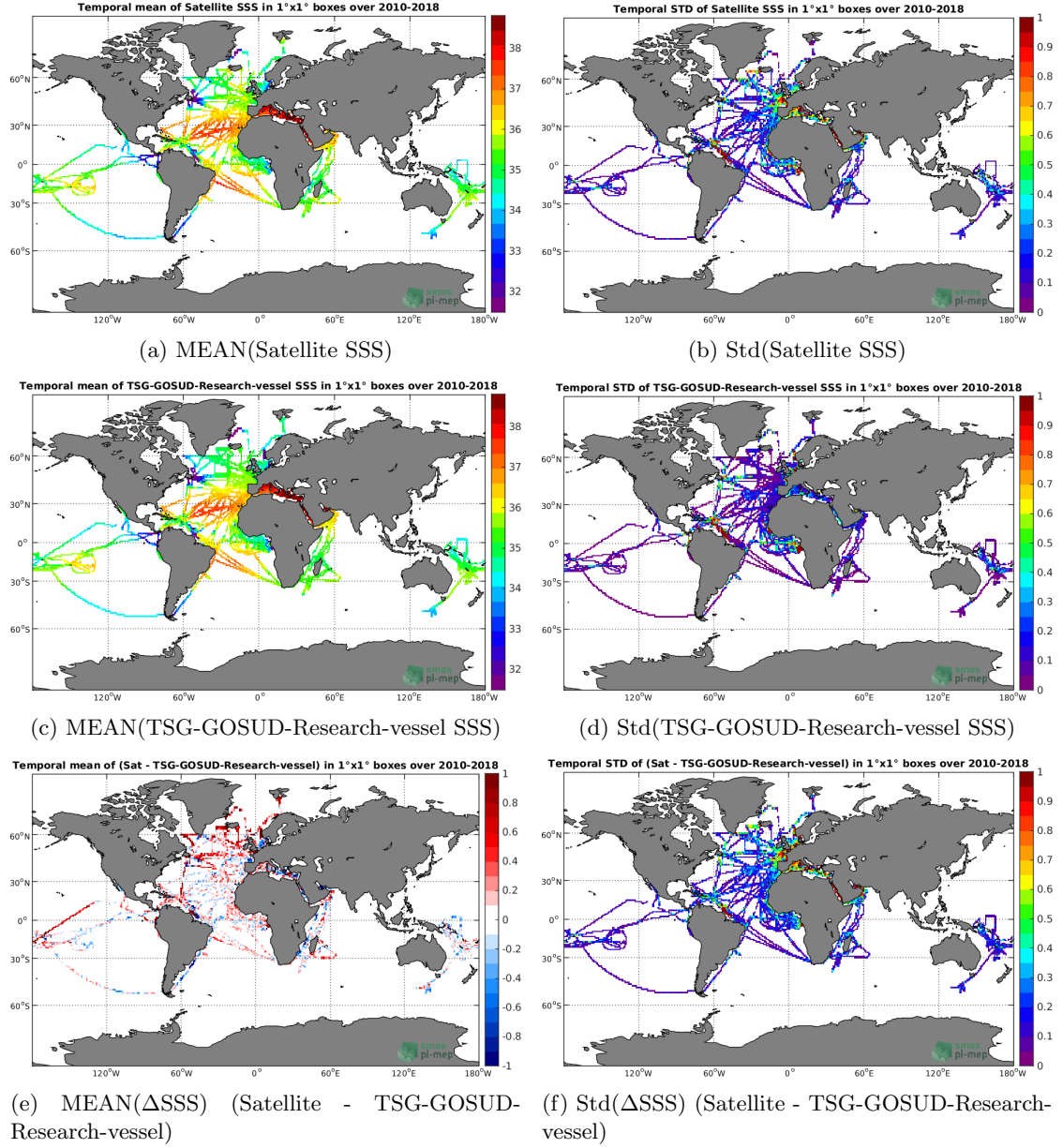
Figure 6: Temporal mean (left) and Std (right) of SSS from SMOS-L3-CATDS-CECOS-LOCEAN-V4-9DAYS-25KM (top), TSG-GOSUD-Research-vessel (middle), and of \Delta SSS (Satellite - TSG-GOSUD-Research-vessel). Only match-up pairs are used to generate these maps.
