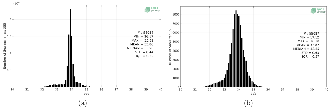
Figure 2: Histograms of SSS from Sea mammals (a) and SMOS SSS L3 v4 - 9 Days (CATDS-CECOS-LOCEAN) (b) considering all match-up pairs per bins of 0.1 over the Global Ocean Pi-MEP region and for the full satellite product period.
