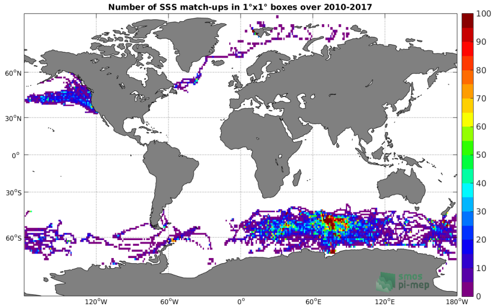
Figure 4: Number of SSS match-ups between Sea mammals SSS and the SMOS SSS L3 v4 - 9 Days (CATDS-CECOS-LOCEAN) SSS product for the Global Ocean Pi-MEP region over 1^\circ \times 1^\circ boxes and for the full satellite product period.
