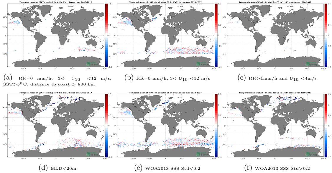
Figure 12: Temporal mean gridded over spatial boxes of size 1^\circ \times 1^\circ of \Delta SSS (SMOS SSS L3 v4 - 9 Days (CATDS-CECOS-LOCEAN) - Sea mammals) for 6 different subdatasets corresponding to: RR=0 mm/h, 3 < U_{10} < 12 m/s, SST > 5^\circ C , distance to coast > 800 km (a), RR=0 mm/h, 3 < U_{10} < 12 m/s (b), RR > 1 mm/h and U_{10} < 4 m/s (c), MLD < 20 m (d), WOA2013 SSS Std < 0.2 (e), WOA2013 SSS Std > 0.2 (f).
