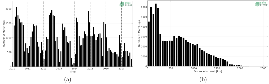
Figure 1: Number of match-ups between Sea mammals and SMOS SSS L3 v4 - 9 Days (CATDS-CECOS-LOCEAN) SSS as a function of time (a) and as function of the distance to coast (b) over the Global Ocean Pi-MEP region and for the full satellite product period.
