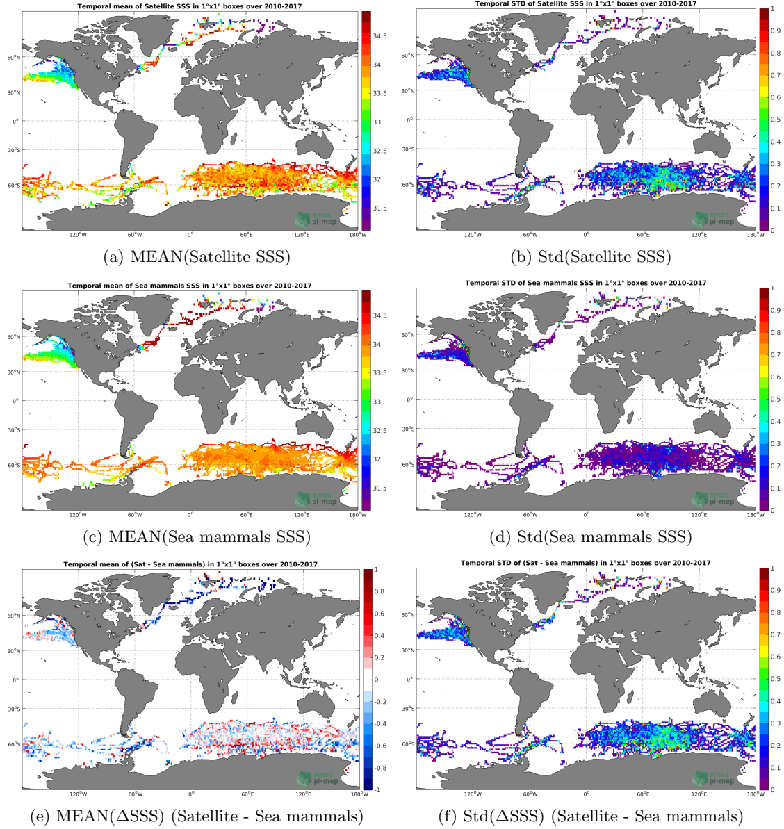
Figure 6: Temporal mean (left) and Std (right) of SSS from SMOS SSS L3 v4 - 9 Days (CATDS-CECOS-LOCEAN) (top), Sea mammals (middle), and of \Delta SSS (Satellite - Sea mammals). Only match-up pairs are used to generate these maps.
