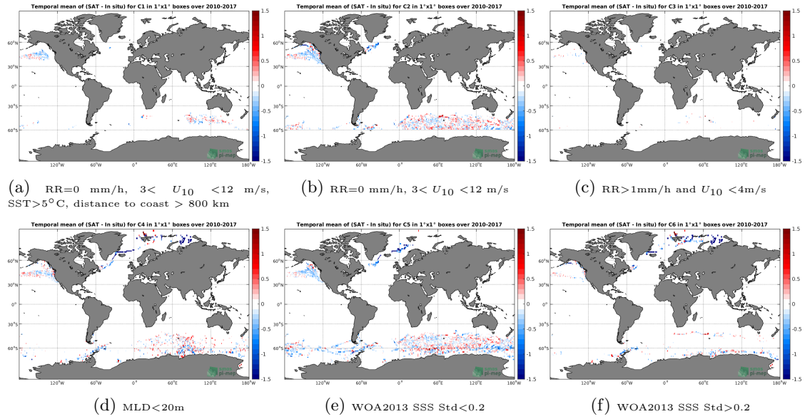
Figure 12: Temporal mean gridded over spatial boxes of size 1^\circ \times 1^\circ of \Delta SSS (SMOS-L3-CATDS-CECOS-LOCEAN-V4-9DAYS-25KM - Sea mammals) for 6 different subdatasets corresponding to: RR=0 mm/h, 3 < U_{10} < 12 m/s, SST >5^\circ C, distance to coast > 800 km (a), RR=0 mm/h, 3 < U_{10} < 12 m/s (b), RR >1 mm/h and U_{10} < 4 m/s (c),MLD <20 m (d),WOA2013 SSS Std <0.2 (e),WOA2013 SSS Std >0.2 (f).
