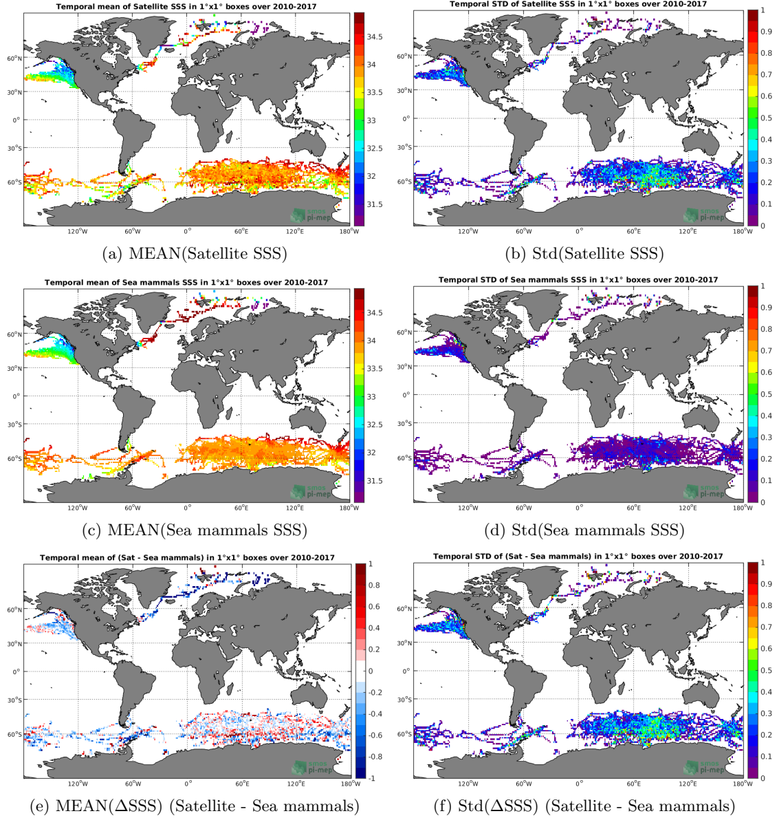
Figure 6: Temporal mean (left) and Std (right) of SSS from SMOS-L3-CATDS-CECOS-LOCEAN-V4-9DAYS-25KM (top), Sea mammals (middle), and of \Delta SSS (Satellite - Sea mammals). Only match-up pairs are used to generate these maps.
