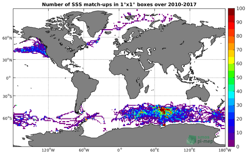
Figure 4: Number of SSS match-ups between Sea mammals SSS and the SMOS-L3-CATDS-CECOS-LOCEAN-V4-9DAYS-25KM SSS product for the Global Ocean Pi-MEP region over 1°x1° boxes and for the full satellite product period.
