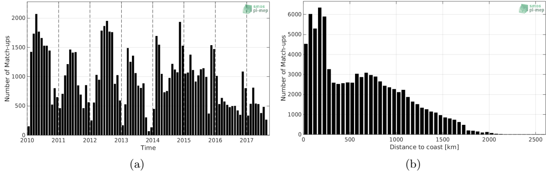
Figure 1: Number of match-ups between Sea mammals and SMOS-L3-CATDS-CECOS-LOCEAN-V4-9DAYS-25KM SSS as a function of time (a) and as function of the distance to coast (b) over the Global Ocean Pi-MEP region and for the full satellite product period.
