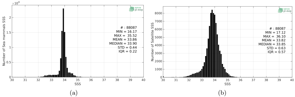
Figure 2: Histograms of SSS from Sea mammals (a) and SMOS-L3-CATDS-CECOS-LOCEAN-V4-9DAYS-25KM (b) considering all match-up pairs per bins of 0.1 over the Global Ocean Pi-MEP region and for the full satellite product period.
