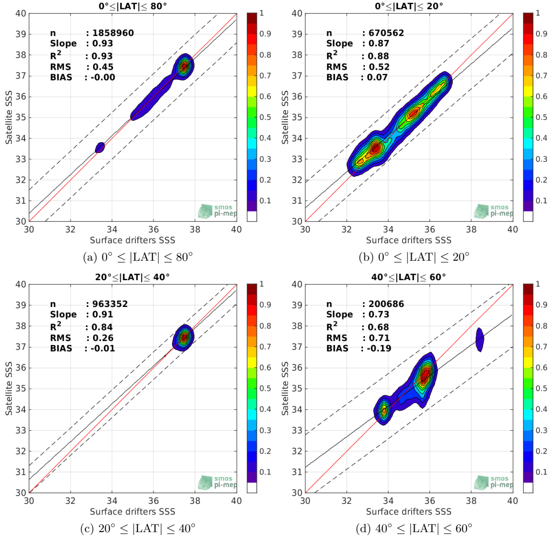
Figure 8: Contour maps of the concentration of SMOS-L3-CATDS-CECOS-LOCEAN-V4-9DAYS-25KM SSS (y-axis) versus Surface drifters SSS (x-axis) at match-up pairs for different latitude bands. For each plot, the red line shows x=y . The black thin and dashed lines indicate a linear fit through the data cloud and the \pm 95\% confidence levels, respectively. The number match-up pairs n , the slope and R^2 coefficient of the linear fit, the root mean square (RMS) and the mean bias between satellite and in situ data are indicated for each latitude band in each plots.
