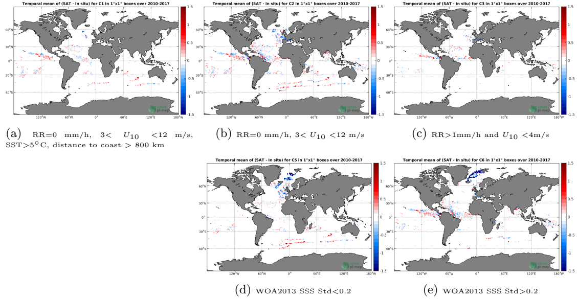
Figure 11: Temporal mean gridded over spatial boxes of size 1^\circ \times 1^\circ of \Delta SSS (SMOS-L3-CATDS-CECOS-LOCEAN-V4-9DAYS-25KM - Surface drifters) for 5 different subdatasets corresponding to: RR=0 mm/h, 3 < U_{10} < 12 m/s, SST >5^\circ C, distance to coast > 800 km (a), RR=0 mm/h, 3 < U_{10} < 12 m/s (b), RR >1 mm/h and U_{10} < 4 m/s (c), WOA2013 SSS Std <0.2 (d), WOA2013 SSS Std >0.2 (e).
