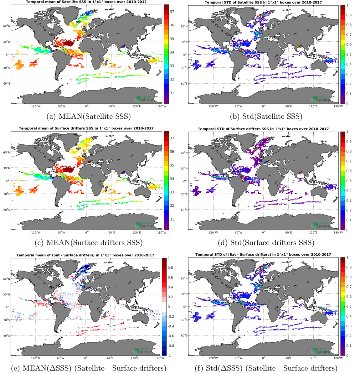
Figure 5: Temporal mean (left) and Std (right) of SSS from SMOS-L3-CATDS-CECOS-LOCEAN-V4-9DAYS-25KM (top), Surface drifters (middle), and of \Delta SSS (Satellite - Surface drifters). Only match-up pairs are used to generate these maps.
