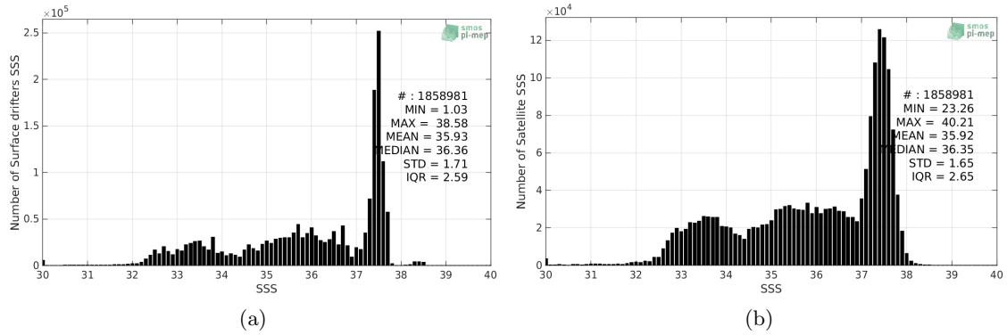
Figure 2: Histograms of SSS from Surface drifters (a) and SMOS-L3-CATDS-CECOS-LOCEAN-V4-9DAYS-25KM (b) considering all match-up pairs per bins of 0.1 over the Global Ocean Pi-MEP region and for the full satellite product period.
