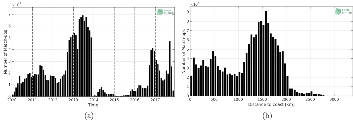
Figure 1: Number of match-ups between Surface drifters and SMOS-L3-CATDS-CECOS-LOCEAN-V4-9DAYS-25KM SSS as a function of time (a) and as function of the distance to coast (b) over the Global Ocean Pi-MEP region and for the full satellite product period.
