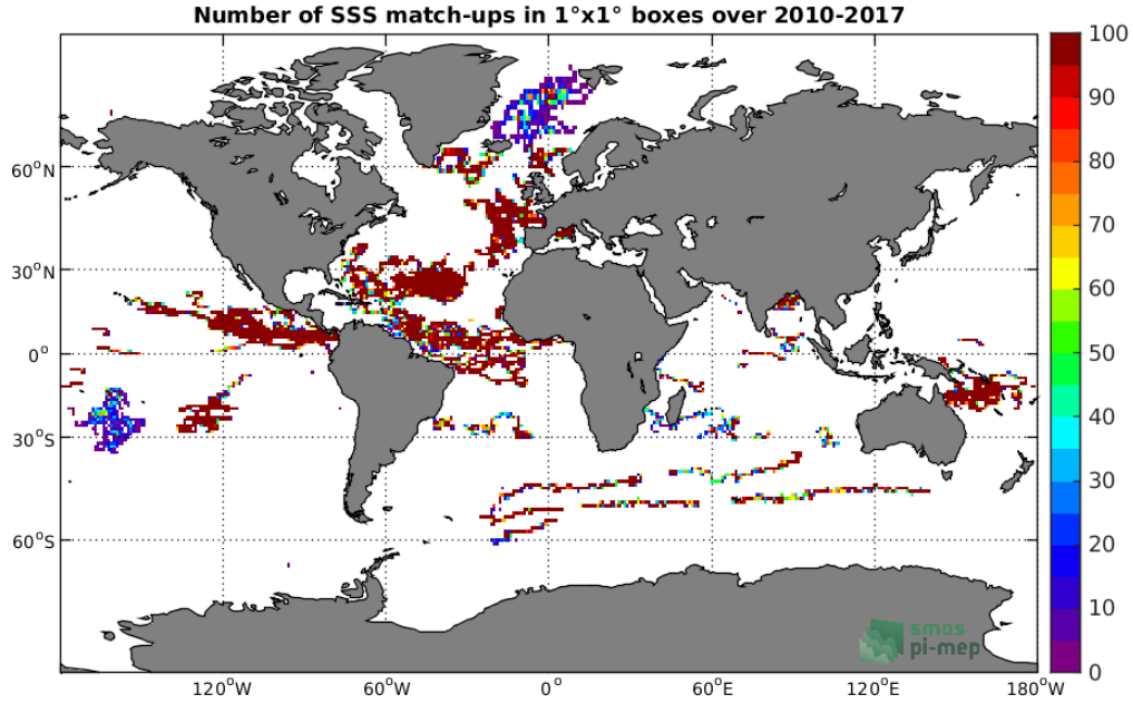
Figure 3: Number of SSS match-ups between Surface drifters SSS and the SMOS-L3-CATDS-CECOS-LOCEAN-V4-9DAYS-25KM SSS product for the Global Ocean Pi-MEP region over 1^\circ \times 1^\circ boxes and for the full satellite product period.
