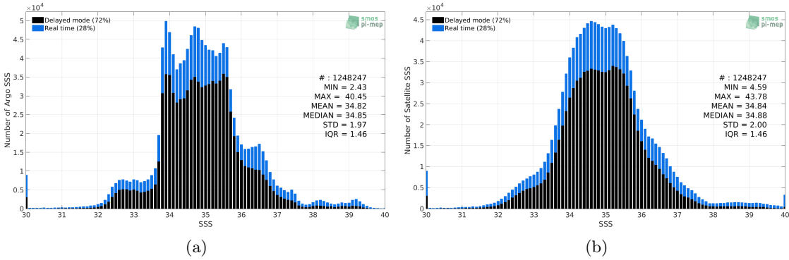
Figure 2: Histograms of SSS from Argo (a) and SMOS-L3-CATDS-CECOS-LOCEAN-V4-9DAYS-25KM (b) considering all match-up pairs per bins of 0.1 over the Global Ocean Pi-MEP region and for the full satellite product period.
