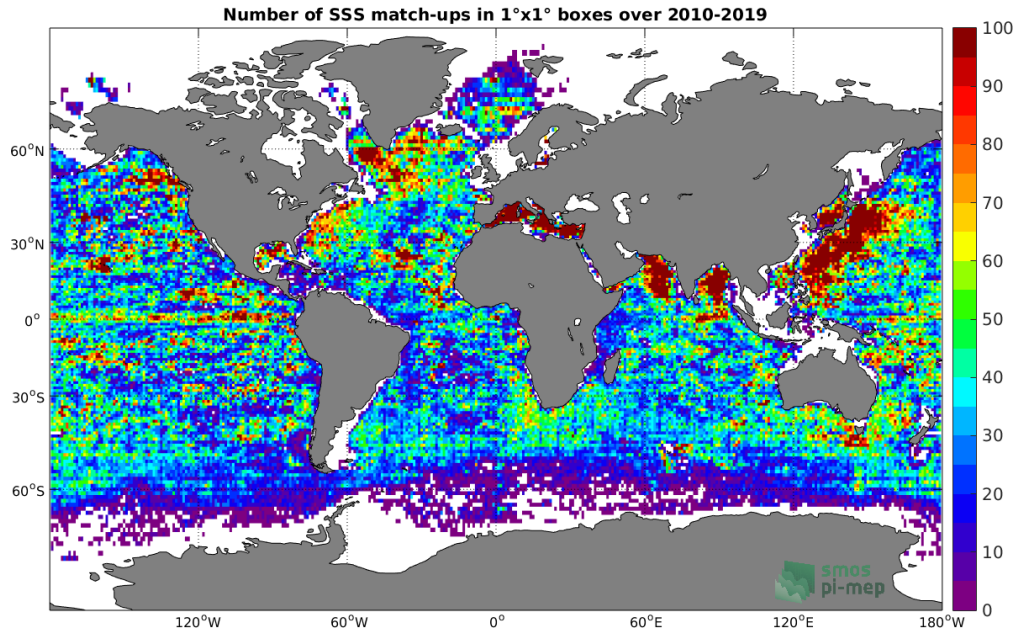
Figure 4: Number of SSS match-ups between Argo SSS and the SMOS-L3-CATDS-CECOS-LOCEAN-V4-9DAYS-25KM SSS product for the Global Ocean Pi-MEP region over 1^\circ \times 1^\circ boxes and for the full satellite product period.
