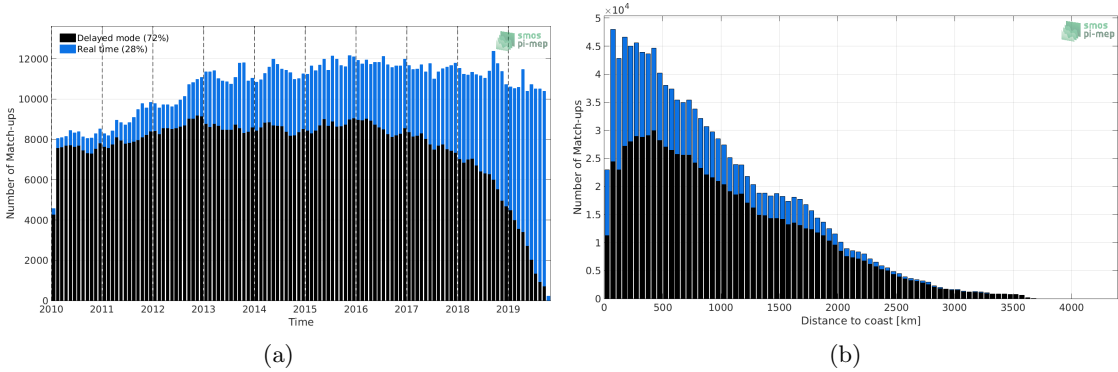
Figure 1: Number of match-ups between Argo and SMOS-L3-CATDS-CECOS-LOCEAN-V4-9DAYS-25KM SSS as a function of time (a) and as function of the distance to coast (b) over the Global Ocean Pi-MEP region and for the full satellite product period.
