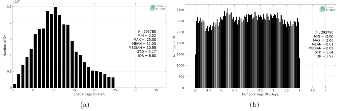
Figure 5: Histograms of the spatial (a) and temporal (b) lags between the time of the TSG (Polarstern) measurements and the date of the corresponding SMOS SSS L3 v4 - 18 Days (CATDS-CECOS-LOCEAN) SSS product.
