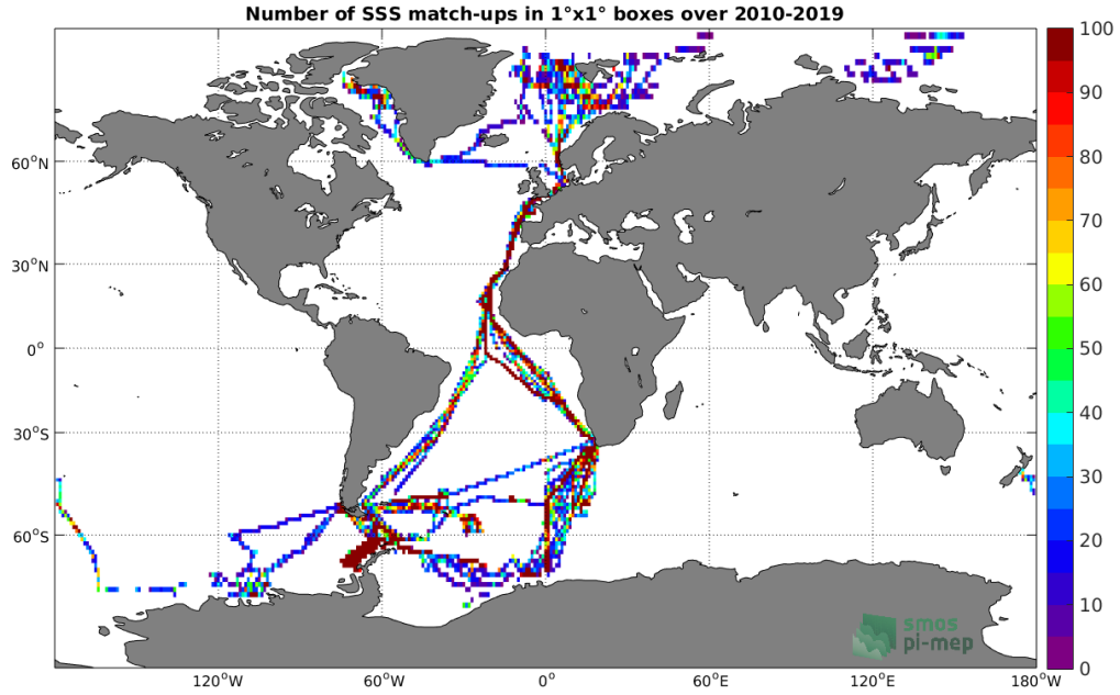
Figure 4: Number of SSS match-ups between TSG (Polarstern) SSS and the SMOS SSS L3 v4 - 18 Days (CATDS-CECOS-LOCEAN) SSS product for the Global Ocean Pi-MEP region over 1^\circ \times 1^\circ boxes and for the full satellite product period.
