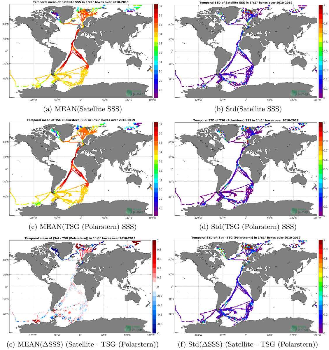
Figure 6: Temporal mean (left) and Std (right) of SSS from SMOS SSS L3 v4 - 18 Days (CATDS-CECOS-LOCEAN) (top), TSG (Polarstern) (middle), and of \Delta SSS (Satellite - TSG (Polarstern)). Only match-up pairs are used to generate these maps.
