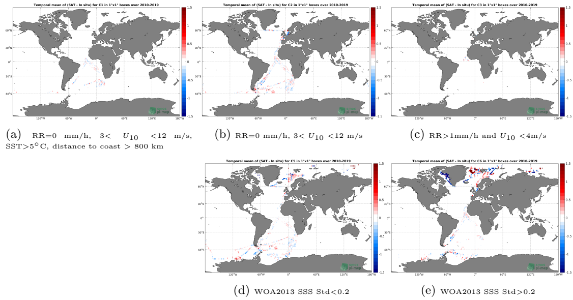
Figure 12: Temporal mean gridded over spatial boxes of size 1^\circ \times 1^\circ of \Delta SSS (SMOS SSS L3 v4 - 18 Days (CATDS-CECOS-LOCEAN) - TSG (Polarstern)) for 5 different subdatasets corresponding to: RR=0 mm/h, 3 < U_{10} < 12 m/s, SST > 5^\circ C , distance to coast > 800 km (a), RR=0 mm/h, 3 < U_{10} < 12 m/s (b), RR > 1 mm/h and U_{10} < 4 m/s (c), WOA2013 SSS Std < 0.2 (d), WOA2013 SSS Std > 0.2 (e).
