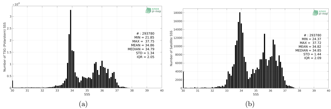
Figure 2: Histograms of SSS from TSG (Polarstern) (a) and SMOS SSS L3 v4 - 18 Days (CATDS-CECOS-LOCEAN) (b) considering all match-up pairs per bins of 0.1 over the Global Ocean Pi-MEP region and for the full satellite product period.
