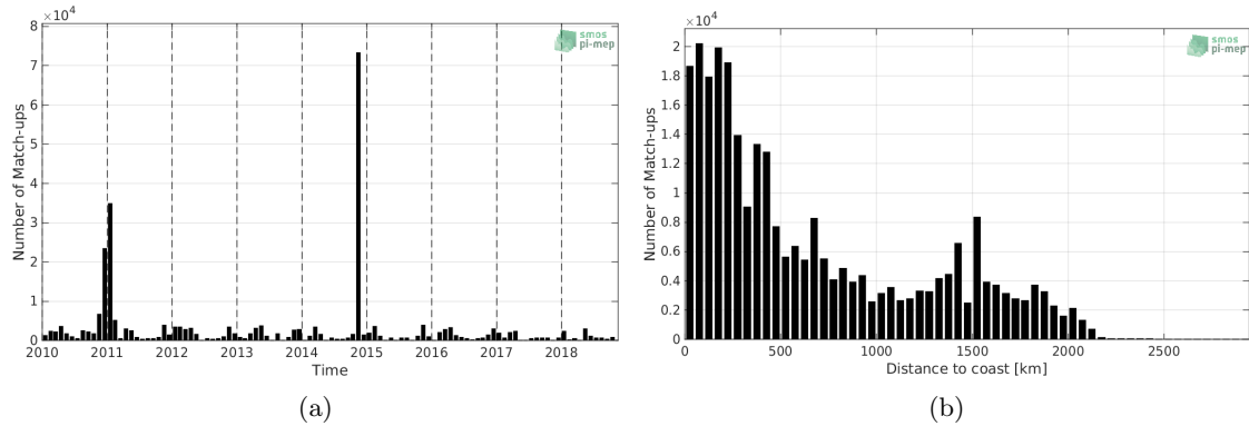
Figure 1: Number of match-ups between TSG-POLARSTERN and SMOS-L3-CATDS-CECOS-LOCEAN-V4-18DAYS-25KM SSS as a function of time (a) and as function of the distance to coast (b) over the Global Ocean Pi-MEP region and for the full satellite product period.
