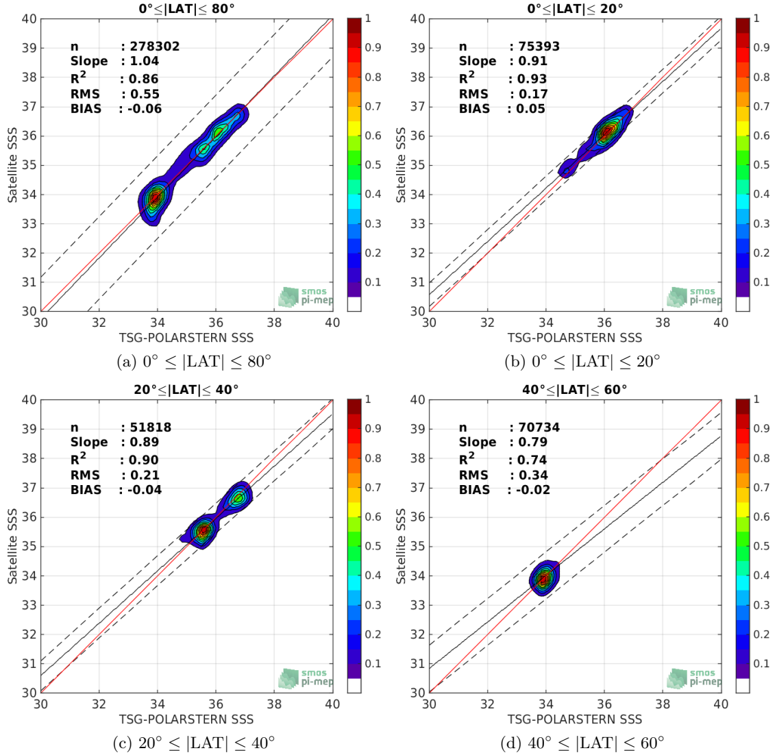
Figure 9: Contour maps of the concentration of SMOS-L3-CATDS-CECOS-LOCEAN-V4-18DAYS-25KM SSS (y-axis) versus TSG-POLARSTERN SSS (x-axis) at match-up pairs for different latitude bands. For each plot, the red line shows x=y . The black thin and dashed lines indicate a linear fit through the data cloud and the \pm 95\% confidence levels, respectively. The number match-up pairs n , the slope and R^2 coefficient of the linear fit, the root mean square (RMS) and the mean bias between satellite and in situ data are indicated for each latitude band in each plots.
