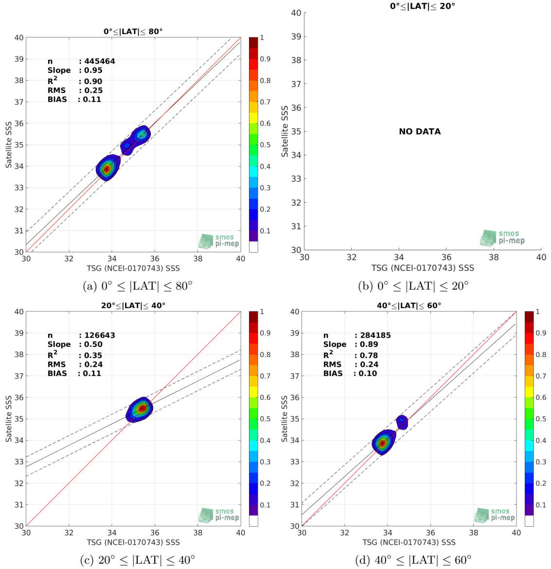
Figure 9: Contour maps of the concentration of SMOS SSS L3 v4 - 18 Days (CATDS-CECOS-LOCEAN) SSS (y-axis) versus TSG (NCEI-0170743) SSS (x-axis) at match-up pairs for different latitude bands. For each plot, the red line shows x=y . The black thin and dashed lines indicate a linear fit through the data cloud and the \pm 95\% confidence levels, respectively. The number match-up pairs n , the slope and R^2 coefficient of the linear fit, the root mean square (RMS) and the mean bias between satellite and in situ data are indicated for each latitude band in each plots.
