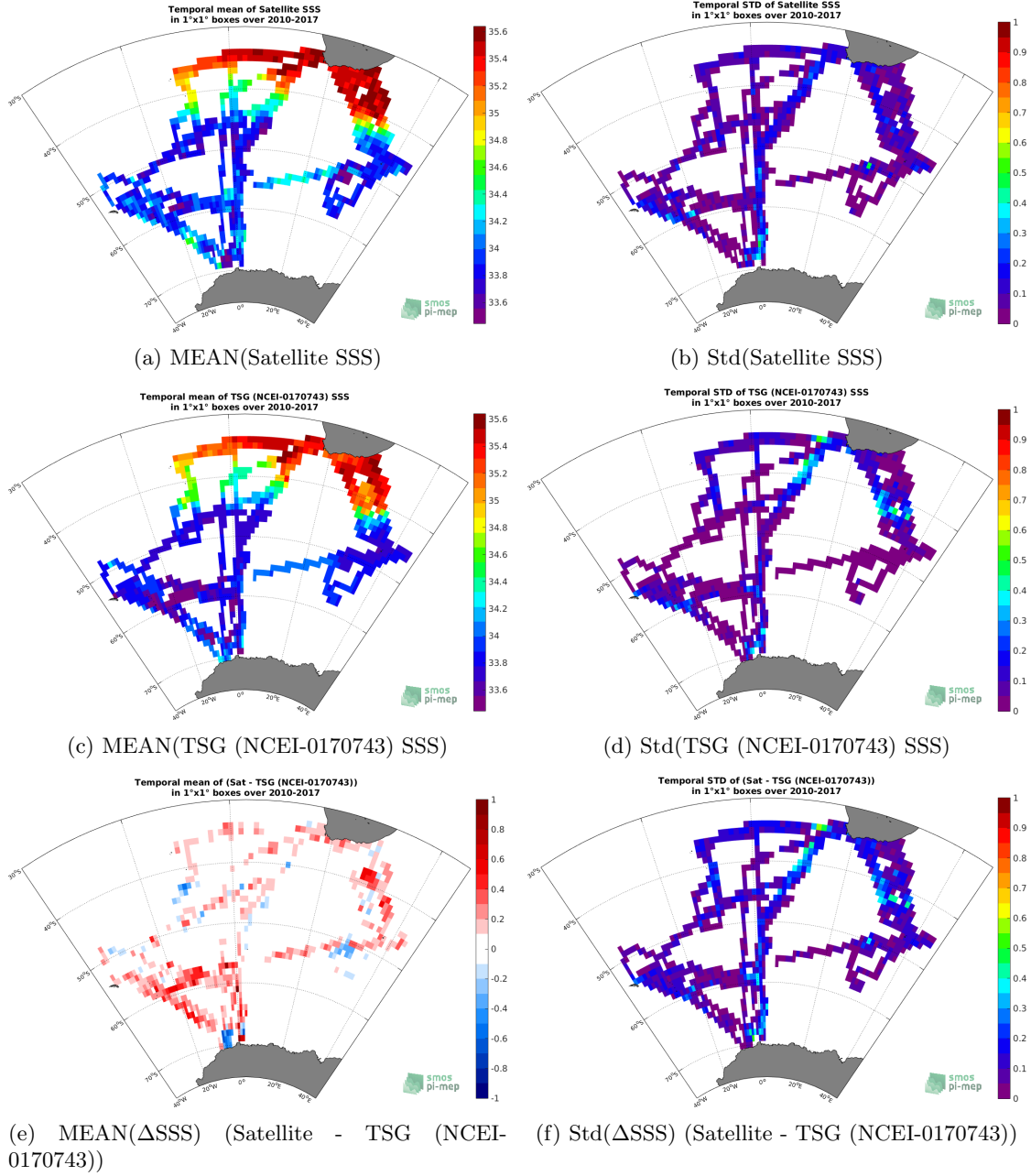
Figure 6: Temporal mean (left) and Std (right) of SSS from SMOS SSS L3 v4 - 18 Days (CATDS-CECOS-LOCEAN) (top), TSG (NCEI-0170743) (middle), and of \Delta SSS (Satellite - TSG (NCEI-0170743)). Only match-up pairs are used to generate these maps.
