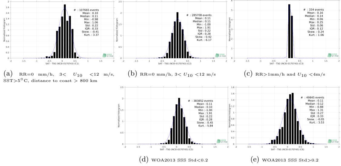
Figure 13: Normalized histogram of \Delta\text{SSS} (SMOS SSS L3 v4 - 18 Days (CATDS-CECOS-LOCEAN) - TSG (NCEI-0170743)) for 5 different subdatasets corresponding to: RR=0 mm/h, 3 < U_{10} < 12 m/s, SST > 5^{\circ}\text{C} , distance to coast > 800 km (a), RR=0 mm/h, 3 < U_{10} < 12 m/s (b), RR > 1\text{mm/h} and U_{10} < 4\text{m/s} (c), WOA2013 SSS Std < 0.2 (d), WOA2013 SSS Std > 0.2 (e).
