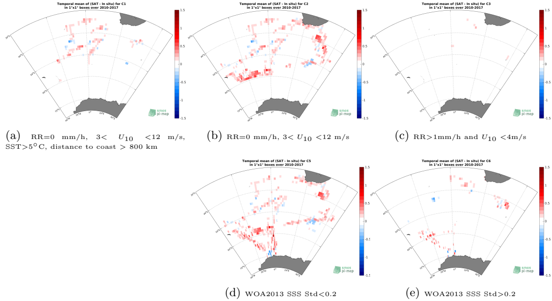
Figure 12: Temporal mean gridded over spatial boxes of size 1^{\circ}\times 1^{\circ} of \Delta\text{SSS} (SMOS SSS L3 v4 - 18 Days (CATDS-CECOS-LOCEAN) - TSG (NCEI-0170743)) for 5 different subdatasets corresponding to: RR=0 mm/h, 3 < U_{10} < 12 m/s, SST > 5^{\circ}\text{C} , distance to coast > 800 km (a), RR=0 mm/h, 3 < U_{10} < 12 m/s (b), RR > 1 mm/h and U_{10} < 4 m/s (c), WOA2013 SSS Std < 0.2 (d), WOA2013 SSS Std > 0.2 (e).
