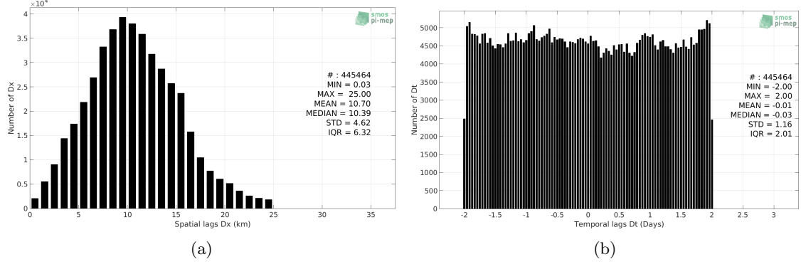
Figure 5: Histograms of the spatial (a) and temporal (b) lags between the time of the TSG (NCEI-0170743) measurements and the date of the corresponding SMOS SSS L3 v4 - 18 Days (CATDS-CECOS-LOCEAN) SSS product.
