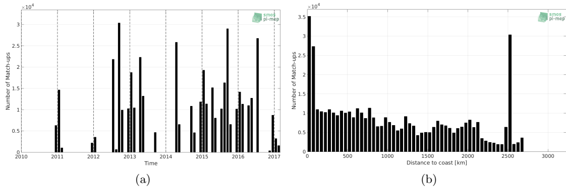
Figure 1: Number of match-ups between TSG (NCEI-0170743) and SMOS SSS L3 v4 - 18 Days (CATDS-CECOS-LOCEAN) SSS as a function of time (a) and as function of the distance to coast (b) over the Global Ocean Pi-MEP region and for the full satellite product period.
