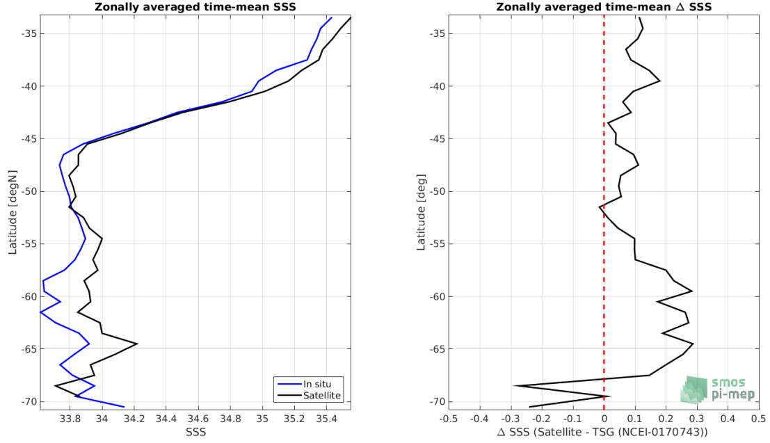
Figure 8: Left panel: Zonal mean SSS from SMOS SSS L3 v4 - 18 Days (CATDS-CECOS-LOCEAN) satellite product (black) and from TSG (NCEI-0170743) (blue). Right panel: Zonal mean of \Delta SSS (Satellite - TSG (NCEI-0170743)) for all the collected Pi-MEP match-up pairs estimated over the full satellite product period.
