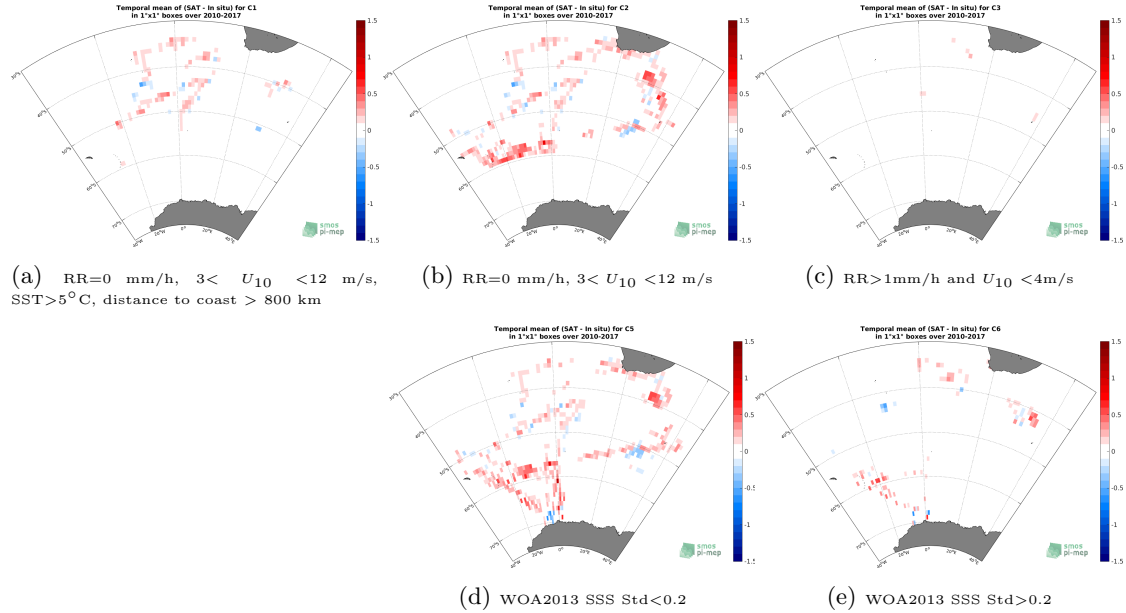
Figure 12: Temporal mean gridded over spatial boxes of size 1^{\circ}\times 1^{\circ} of \Delta\text{SSS} (SMOS-L3-CATDS-CECOS-LOCEAN-V4-18DAYS-25KM - TSG-NCEI-0170743) for 5 different subdatasets corresponding to: RR=0 mm/h, 3 < U_{10} < 12 m/s, SST >5^{\circ}\text{C} , distance to coast > 800 km (a), RR=0 mm/h, 3 < U_{10} < 12 m/s (b), RR >1 mm/h and U_{10} < 4 m/s (c), WOA2013 SSS Std <0.2 (d), WOA2013 SSS Std >0.2 (e).
