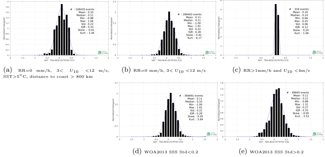
Figure 13: Normalized histogram of \Delta SSS (SMOS-L3-CATDS-CECOS-LOCEAN-V4-18DAYS-25KM - TSG-NCEI-0170743) for 5 different subdatasets corresponding to: RR=0 mm/h, 3 < U_{10} < 12 m/s, SST > 5°C, distance to coast > 800 km (a), RR=0 mm/h, 3 < U_{10} < 12 m/s (b), RR > 1mm/h and U_{10} < 4 m/s (c), WOA2013 SSS Std < 0.2 (d), WOA2013 SSS Std > 0.2 (e).
