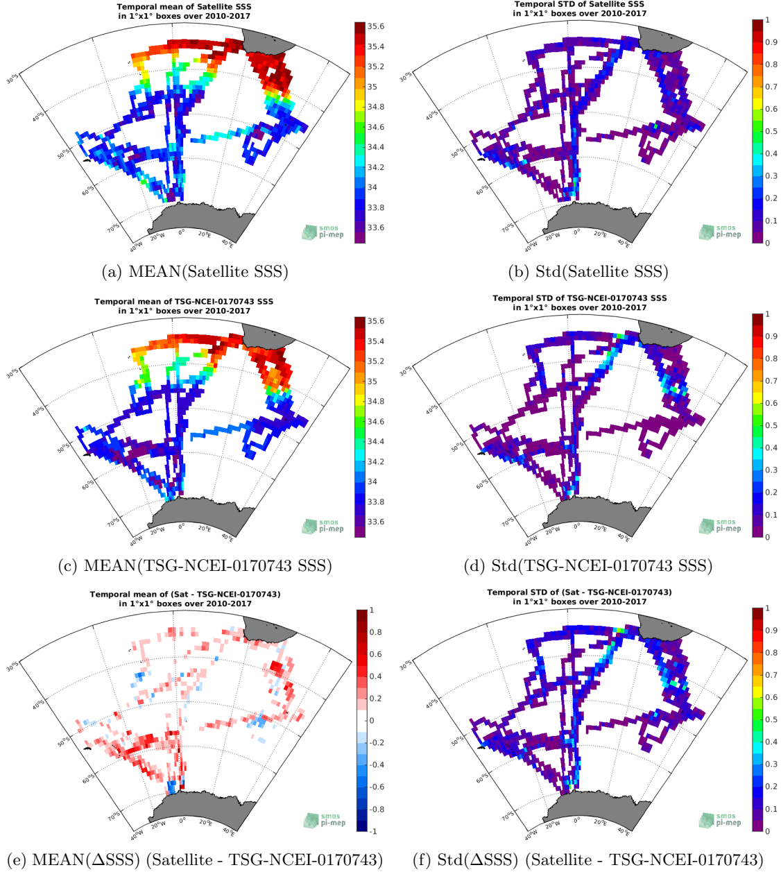
Figure 6: Temporal mean (left) and Std (right) of SSS from SMOS-L3-CATDS-CECOS-LOCEAN-V4-18DAYS-25KM (top), TSG-NCEI-0170743 (middle), and of \Delta SSS (Satellite - TSG-NCEI-0170743). Only match-up pairs are used to generate these maps.
