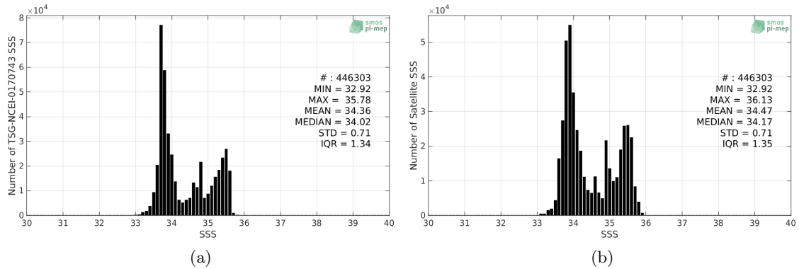
Figure 2: Histograms of SSS from TSG-NCEI-0170743 (a) and SMOS-L3-CATDS-CECOS-LOCEAN-V4-18DAYS-25KM (b) considering all match-up pairs per bins of 0.1 over the Global Ocean Pi-MEP region and for the full satellite product period.
