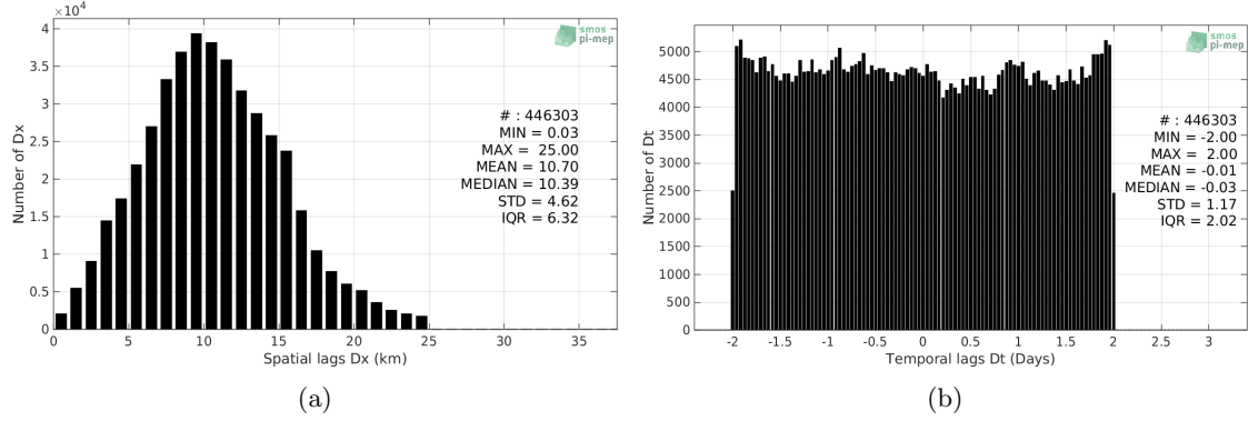
Figure 5: Histograms of the spatial (a) and temporal (b) lags between the time of the TSG-NCEI-0170743 measurements and the date of the corresponding SMOS-L3-CATDS-CECOS-LOCEAN-V4-18DAYS-25KM SSS product.
