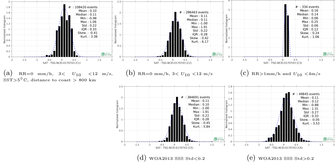
Figure 13: Normalized histogram of \Delta SSS (SMOS-L3-CATDS-CECOS-LOCEAN-V4-18DAYS-25KM - TSG-NCEI-0170743) for 5 different subdatasets corresponding to: RR=0 mm/h, 3 < U_{10} < 12 m/s, SST>5°C, distance to coast > 800 km (a), RR=0 mm/h, 3 < U_{10} < 12 m/s (b), RR>1mm/h and U_{10} < 4 m/s (c), WOA2013 SSS Std<0.2 (d), WOA2013 SSS Std>0.2 (e).
