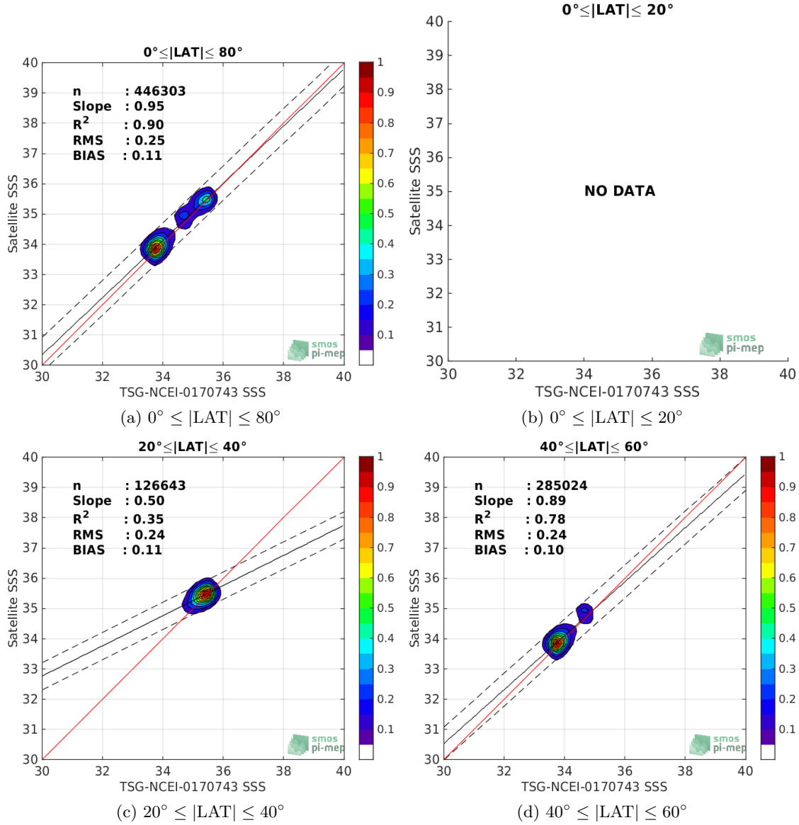
Figure 9: Contour maps of the concentration of SMOS-L3-CATDS-CECOS-LOCEAN-V4-18DAYS-25KM SSS (y-axis) versus TSG-NCEI-0170743 SSS (x-axis) at match-up pairs for different latitude bands. For each plot, the red line shows x=y . The black thin and dashed lines indicate a linear fit through the data cloud and the \pm 95\% confidence levels, respectively. The number match-up pairs n , the slope and R^2 coefficient of the linear fit, the root mean square (RMS) and the mean bias between satellite and in situ data are indicated for each latitude band in each plots.
