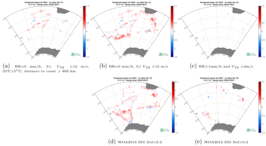
Figure 12: Temporal mean gridded over spatial boxes of size 1^\circ \times 1^\circ of \Delta SSS (SMOS-L3-CATDS-CECOS-LOCEAN-V4-18DAYS-25KM - TSG-NCEI-0170743) for 5 different subdatasets corresponding to:RR=0 mm/h, 3 < U_{10} < 12 m/s, SST >5^\circ C, distance to coast > 800 km (a), RR=0 mm/h, 3 < U_{10} < 12 m/s (b), RR >1 mm/h and U_{10} < 4 m/s (c), WOA2013 SSS Std <0.2 (d), WOA2013 SSS Std >0.2 (e).
