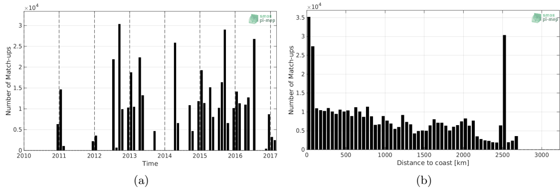
Figure 1: Number of match-ups between TSG-NCEI-0170743 and SMOS-L3-CATDS-CECOS-LOCEAN-V4-18DAYS-25KM SSS as a function of time (a) and as function of the distance to coast (b) over the Global Ocean Pi-MEP region and for the full satellite product period.
