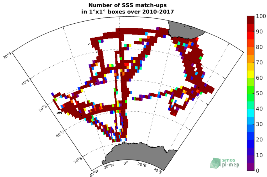
Figure 4: Number of SSS match-ups between TSG-NCEI-0170743 SSS and the SMOS-L3-CATDS-CECOS-LOCEAN-V4-18DAYS-25KM SSS product for the Global Ocean Pi-MEP region over 1°x1° boxes and for the full satellite product period.
