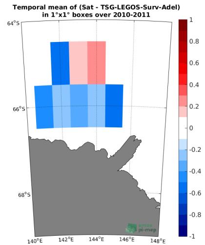
(e) MEAN( \Delta SSS) (Satellite - TSG-LEGOS-Surv-Adel)
