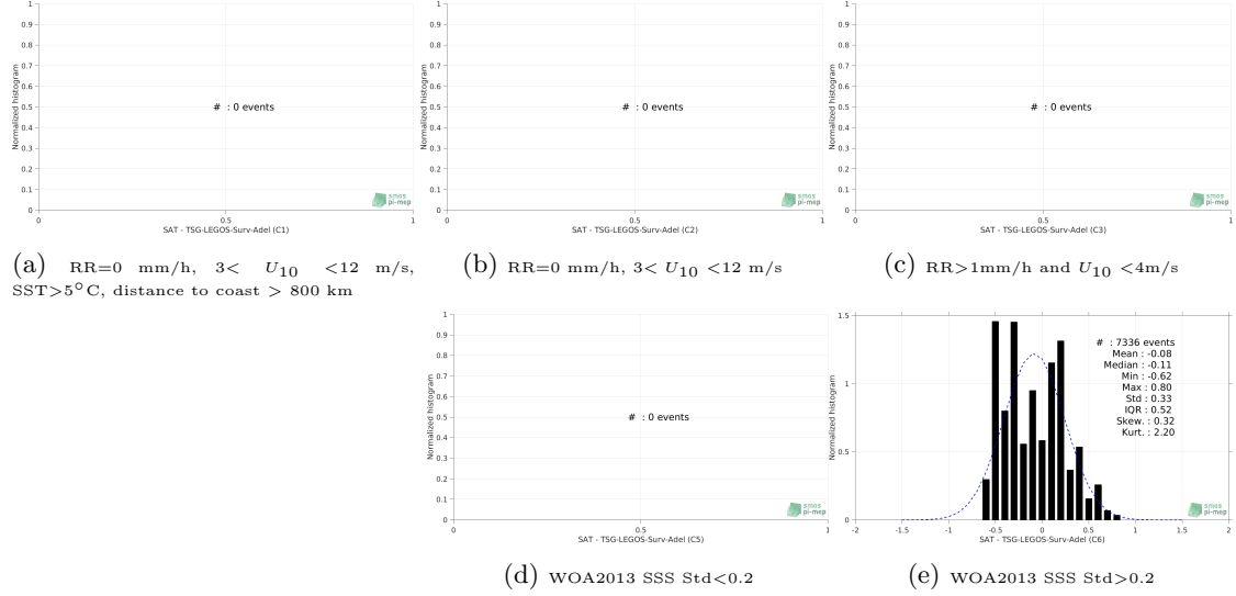
Figure 13: Normalized histogram of \Delta SSS (SMOS-L3-CATDS-CECOS-LOCEAN-V4-18DAYS-25KM - TSG-LEGOS-Surv-Adel) for 5 different subdatasets corresponding to: RR=0 mm/h, 3 < U_{10} < 12 m/s, SST>5°C, distance to coast > 800 km (a), RR=0 mm/h, 3 < U_{10} < 12 m/s (b), RR>1 mm/h and U_{10} < 4 m/s (c), WOA2013 SSS Std<0.2 (d), WOA2013 SSS Std>0.2 (e).
