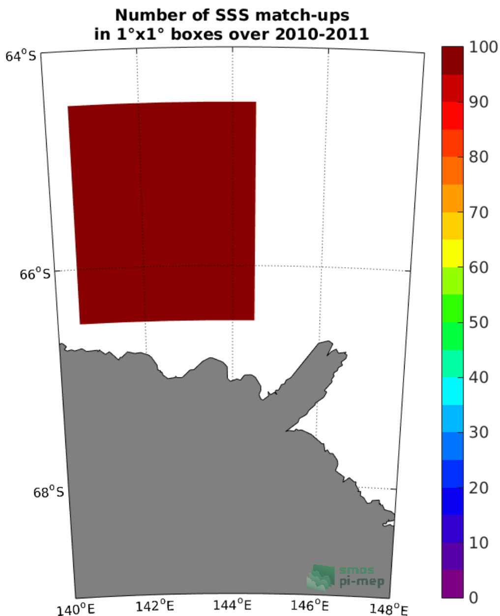
Figure 4: Number of SSS match-ups between TSG-LEGOS-Surv-Adel SSS and the SMOS-L3-CATDS-CECOS-LOCEAN-V4-18DAYS-25KM SSS product for the Global Ocean Pi-MEP region over 1°x1° boxes and for the full satellite product period.
