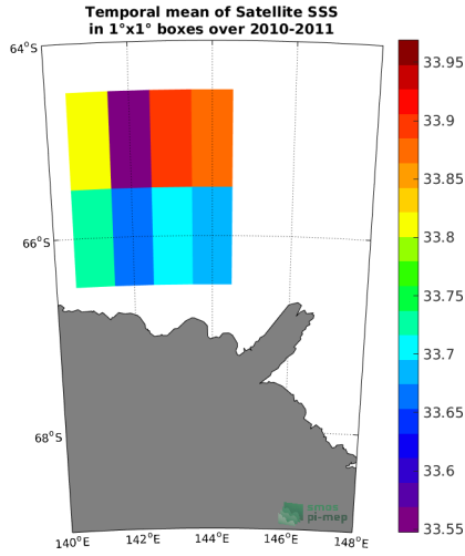
(a) MEAN(Satellite SSS)
