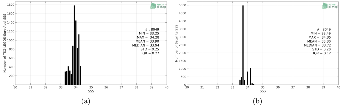
Figure 2: Histograms of SSS from TSG-LEGOS-Surv-Adel (a) and SMOS-L3-CATDS-CECOS-LOCEAN-V4-18DAYS-25KM (b) considering all match-up pairs per bins of 0.1 over the Global Ocean Pi-MEP region and for the full satellite product period.
