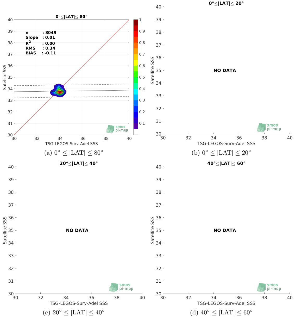
Figure 9: Contour maps of the concentration of SMOS-L3-CATDS-CECOS-LOCEAN-V4-18DAYS-25KM SSS (y-axis) versus TSG-LEGOS-Surv-Adel SSS (x-axis) at match-up pairs for different latitude bands. For each plot, the red line shows x=y . The black thin and dashed lines indicate a linear fit through the data cloud and the \pm 95\% confidence levels, respectively. The number match-up pairs n , the slope and R^2 coefficient of the linear fit, the root mean square (RMS) and the mean bias between satellite and in situ data are indicated for each latitude band in each plots.
