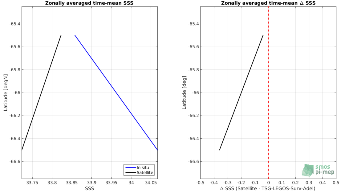
Figure 8: Left panel: Zonal mean SSS from SMOS-L3-CATDS-CECOS-LOCEAN-V4-18DAYS-25KM satellite product (black) and from TSG-LEGOS-Surv-Adel (blue). Right panel: Zonal mean of \Delta SSS (Satellite - TSG-LEGOS-Surv-Adel) for all the collected Pi-MEP match-up pairs estimated over the full satellite product period.
