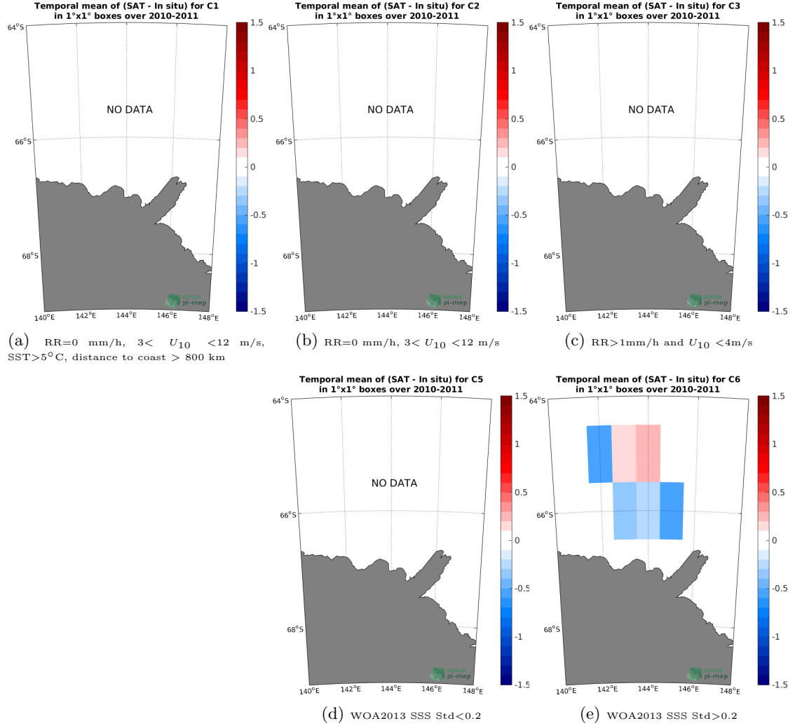
Figure 12: Temporal mean gridded over spatial boxes of size 1°x1° of \Delta SSS (SMOS-L3-CATDS-CECOS-LOCEAN-V4-18DAYS-25KM - TSG-LEGOS-Surv-Adel) for 5 different subdatasets corresponding to: RR=0 mm/h, 3 < U_{10} < 12 m/s, SST>5°C, distance to coast > 800 km (a), RR=0 mm/h, 3 < U_{10} < 12 m/s (b), RR>1mm/h and U_{10} < 4 m/s (c), WOA2013 SSS Std<0.2 (d), WOA2013 SSS Std>0.2 (e).
