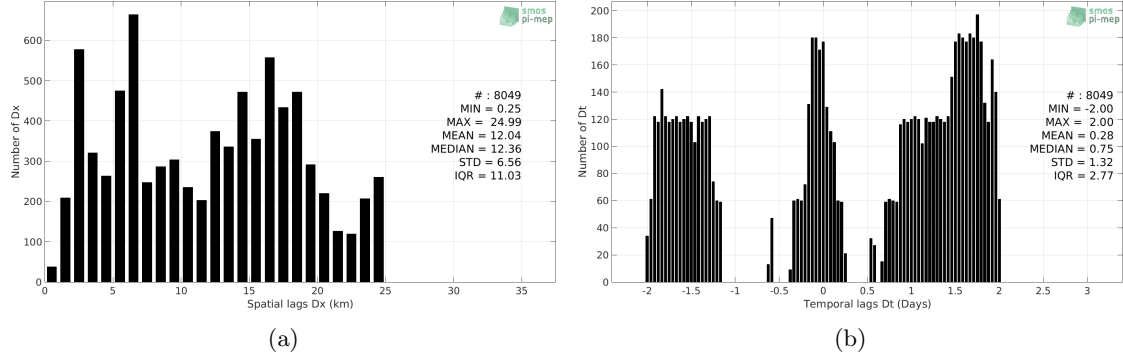
Figure 5: Histograms of the spatial (a) and temporal (b) lags between the time of the TSG-LEGOS-Surv-Adel measurements and the date of the corresponding SMOS-L3-CATDS-CECOS-LOCEAN-V4-18DAYS-25KM SSS product.
