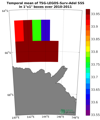
(c) MEAN(TSG-LEGOS-Surv-Adel SSS)
