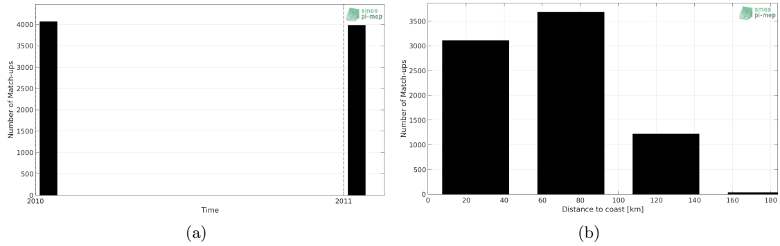
Figure 1: Number of match-ups between TSG-LEGOS-Surv-Adel and SMOS-L3-CATDS-CECOS-LOCEAN-V4-18DAYS-25KM SSS as a function of time (a) and as function of the distance to coast (b) over the Global Ocean Pi-MEP region and for the full satellite product period.
