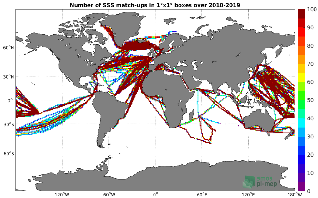
Figure 4: Number of SSS match-ups between TSG (LEGOS-DM) SSS and the SMOS SSS L3 v4 - 18 Days (CATDS-CECOS-LOCEAN) SSS product for the Global Ocean Pi-MEP region over 1^\circ \times 1^\circ boxes and for the full satellite product period.
