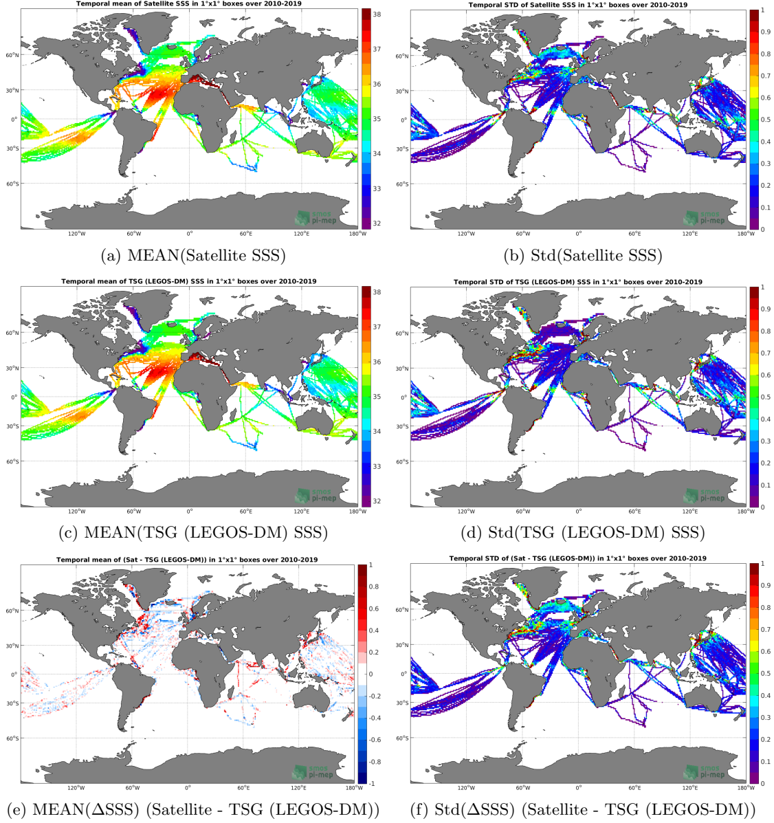
Figure 6: Temporal mean (left) and Std (right) of SSS from SMOS SSS L3 v4 - 18 Days (CATDS-CECOS-LOCEAN) (top), TSG (LEGOS-DM) (middle), and of \Delta SSS (Satellite - TSG (LEGOS-DM)). Only match-up pairs are used to generate these maps.
