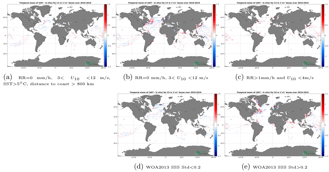
Figure 12: Temporal mean gridded over spatial boxes of size 1^\circ \times 1^\circ of \Delta SSS (SMOS SSS L3 v4 - 18 Days (CATDS-CECOS-LOCEAN) - TSG (LEGOS-DM)) for 5 different subdatasets corresponding to: RR=0 mm/h, 3 < U_{10} < 12 m/s, SST > 5^\circ C , distance to coast > 800 km (a), RR=0 mm/h, 3 < U_{10} < 12 m/s (b), RR > 1 mm/h and U_{10} < 4 m/s (c), WOA2013 SSS Std < 0.2 (d), WOA2013 SSS Std > 0.2 (e).
