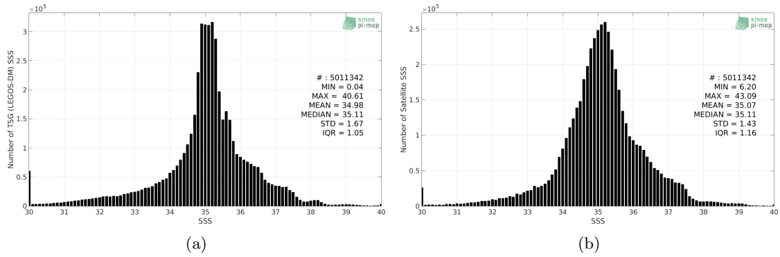
Figure 2: Histograms of SSS from TSG (LEGOS-DM) (a) and SMOS SSS L3 v4 - 18 Days (CATDS-CECOS-LOCEAN) (b) considering all match-up pairs per bins of 0.1 over the Global Ocean Pi-MEP region and for the full satellite product period.
