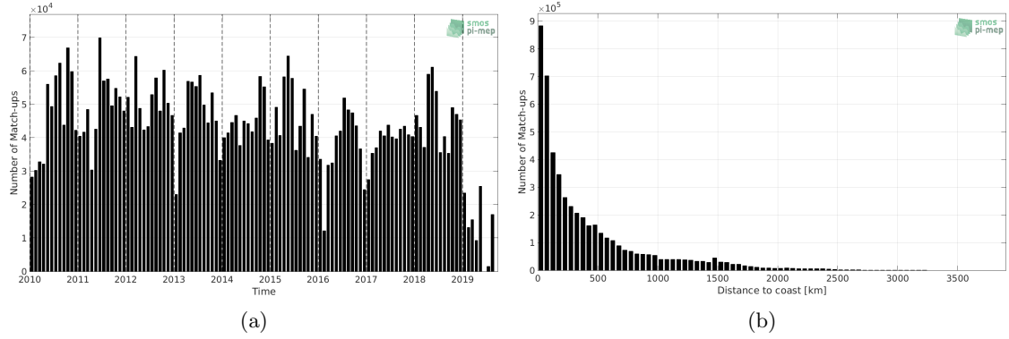
Figure 1: Number of match-ups between TSG (LEGOS-DM) and SMOS SSS L3 v4 - 18 Days (CATDS-CECOS-LOCEAN) SSS as a function of time (a) and as function of the distance to coast (b) over the Global Ocean Pi-MEP region and for the full satellite product period.
