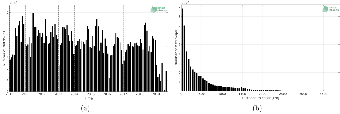
Figure 1: Number of match-ups between TSG-LEGOS-DM and SMOS-L3-CATDS-CECOS-LOCEAN-V4-18DAYS-25KM SSS as a function of time (a) and as function of the distance to coast (b) over the Global Ocean Pi-MEP region and for the full satellite product period.
