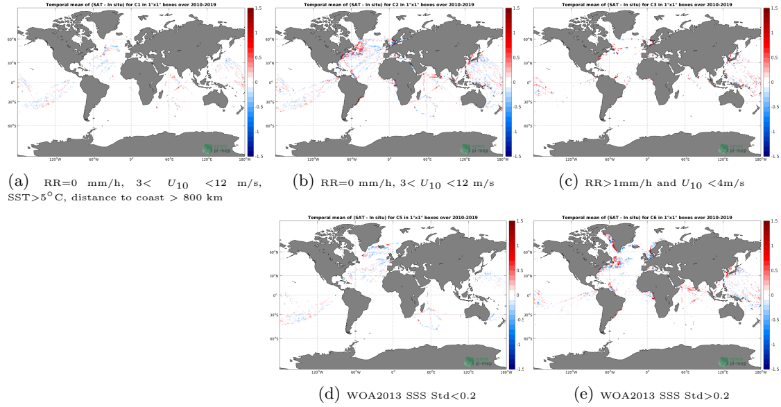
Figure 12: Temporal mean gridded over spatial boxes of size 1^\circ \times 1^\circ of \Delta SSS (SMOS-L3-CATDS-CECOS-LOCEAN-V4-18DAYS-25KM - TSG-LEGOS-DM) for 5 different subdatasets corresponding to: RR=0 mm/h, 3 < U_{10} < 12 m/s, SST > 5^\circ C , distance to coast > 800 km (a), RR=0 mm/h, 3 < U_{10} < 12 m/s (b), RR > 1 mm/h and U_{10} < 4 m/s (c), WOA2013 SSS Std < 0.2 (d), WOA2013 SSS Std > 0.2 (e).
