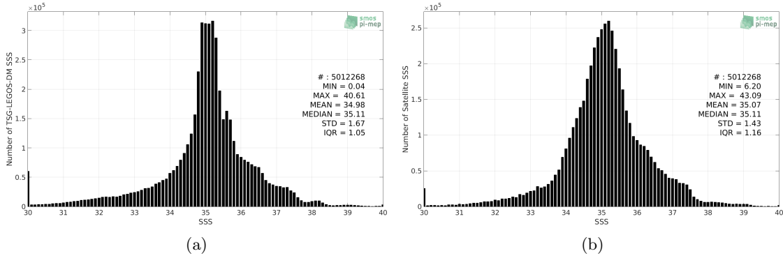
Figure 2: Histograms of SSS from TSG-LEGOS-DM (a) and SMOS-L3-CATDS-CECOS-LOCEAN-V4-18DAYS-25KM (b) considering all match-up pairs per bins of 0.1 over the Global Ocean Pi-MEP region and for the full satellite product period.
