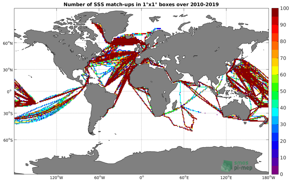
Figure 4: Number of SSS match-ups between TSG-LEGOS-DM SSS and the SMOS-L3-CATDS-CECOS-LOCEAN-V4-18DAYS-25KM SSS product for the Global Ocean Pi-MEP region over 1°x1° boxes and for the full satellite product period.
