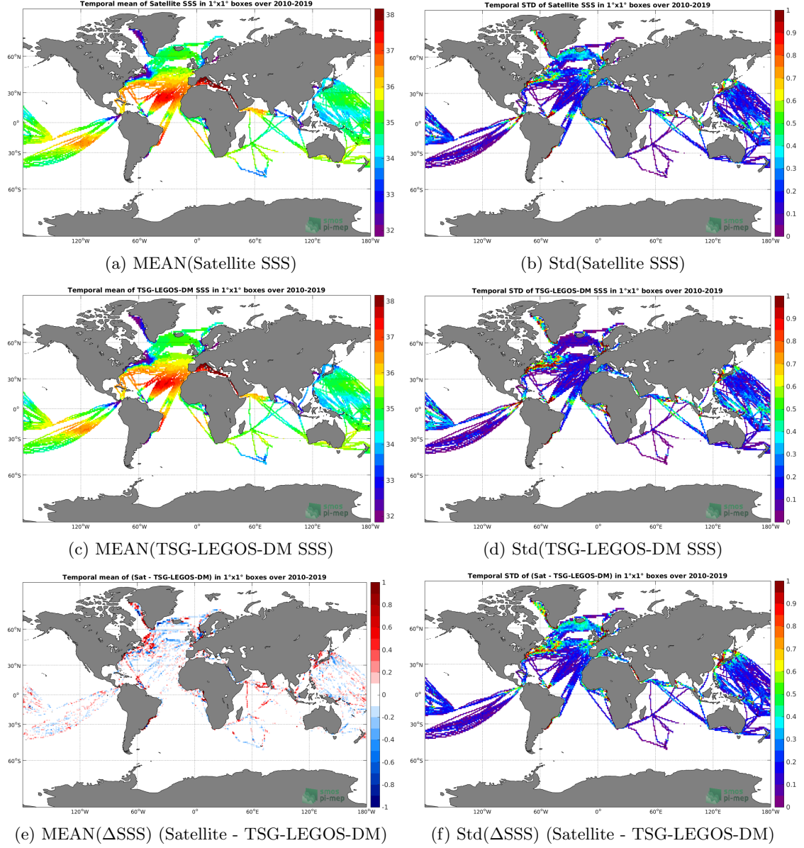
Figure 6: Temporal mean (left) and Std (right) of SSS from SMOS-L3-CATDS-CECOS-LOCEAN-V4-18DAYS-25KM (top), TSG-LEGOS-DM (middle), and of \Delta SSS (Satellite - TSG-LEGOS-DM). Only match-up pairs are used to generate these maps.
