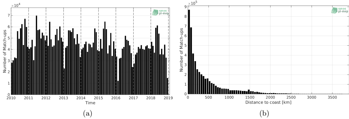
Figure 1: Number of match-ups between TSG-LEGOS-DM and SMOS-L3-CATDS-CECOS-LOCEAN-V4-18DAYS-25KM SSS as a function of time (a) and as function of the distance to coast (b) over the Global Ocean Pi-MEP region and for the full satellite product period.
