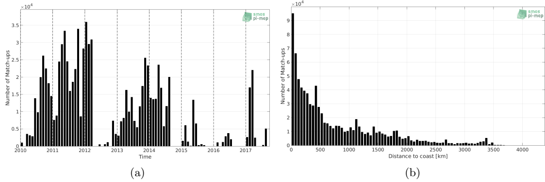
Figure 1: Number of match-ups between TSG (GOSUD-Sailing-ship) and SMOS SSS L3 v4 - 18 Days (CATDS-CECOS-LOCEAN) SSS as a function of time (a) and as function of the distance to coast (b) over the Global Ocean Pi-MEP region and for the full satellite product period.
