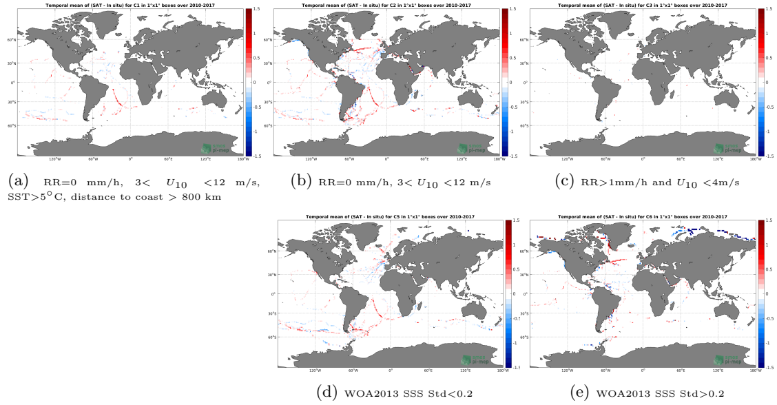
Figure 12: Temporal mean gridded over spatial boxes of size 1^\circ \times 1^\circ of \Delta SSS (SMOS SSS L3 v4 - 18 Days (CATDS-CECOS-LOCEAN) - TSG (GOSUD-Sailing-ship)) for 5 different subdatasets corresponding to: RR=0 mm/h, 3 < U_{10} < 12 m/s, SST>5°C, distance to coast > 800 km (a), RR=0 mm/h, 3 < U_{10} < 12 m/s (b), RR>1mm/h and U_{10} < 4 m/s (c), WOA2013 SSS Std<0.2 (d), WOA2013 SSS Std>0.2 (e).
