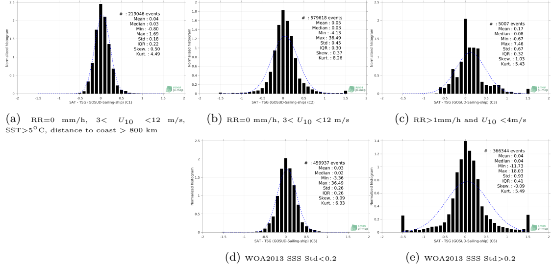
Figure 13: Normalized histogram of \Delta SSS (SMOS SSS L3 v4 - 18 Days (CATDS-CECOS-LOCEAN) - TSG (GOSUD-Sailing-ship)) for 5 different subdatasets corresponding to: RR=0 mm/h, 3 < U_{10} < 12 m/s, SST>5°C, distance to coast > 800 km (a), RR=0 mm/h, 3 < U_{10} < 12 m/s (b), RR>1mm/h and U_{10} < 4 m/s (c), WOA2013 SSS Std<0.2 (d), WOA2013 SSS Std>0.2 (e).
