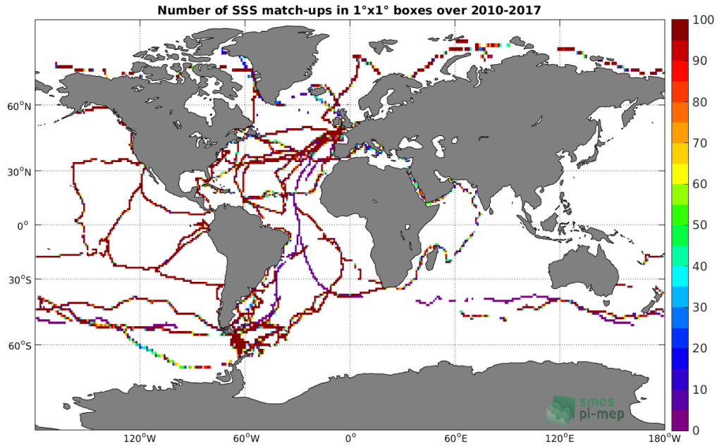
Figure 4: Number of SSS match-ups between TSG (GOSUD-Sailing-ship) SSS and the SMOS SSS L3 v4 - 18 Days (CATDS-CECOS-LOCEAN) SSS product for the Global Ocean Pi-MEP region over 1°x1° boxes and for the full satellite product period.
