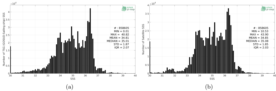
Figure 2: Histograms of SSS from TSG (GOSUD-Sailing-ship) (a) and SMOS SSS L3 v4 - 18 Days (CATDS-CECOS-LOCEAN) (b) considering all match-up pairs per bins of 0.1 over the Global Ocean Pi-MEP region and for the full satellite product period.
